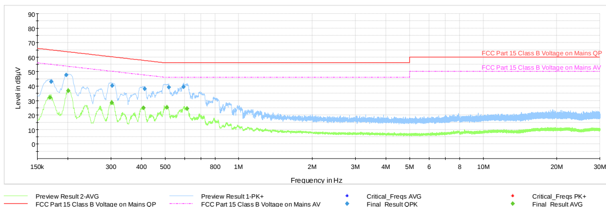
Plot 7-304. Line Conducted Plot with 802.11n UNII Band 1 Ch.36 (N) with AC/DC Adapter
