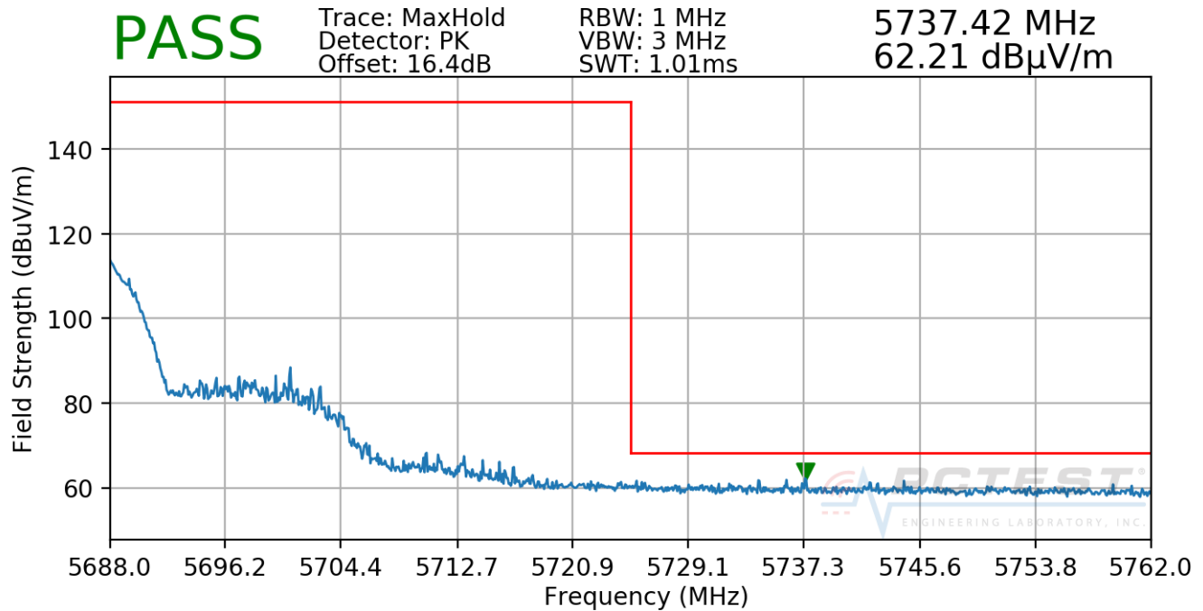
Plot 7-239. Radiated Upper Band Edge Plot SISO CORE 1 (UNII Band 2C)
