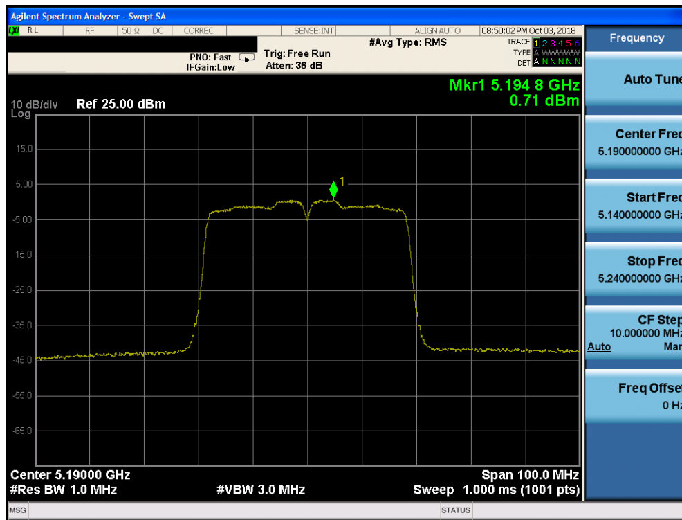
Plot 7-111. Power Spectral Density Plot CDD CORE 0 (40MHz BW 802.11n (UNII Band 1) – Ch. 38) - ISED
