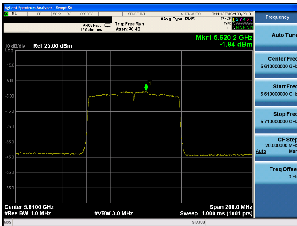
Plot 7-153. Power Spectral Density Plot CDD CORE 0 (80MHz BW 802.11ac (UNII Band 2C) – Ch. 122)
