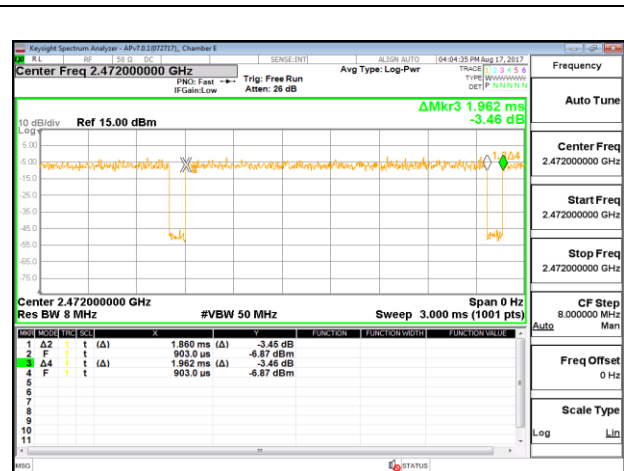
DUTY CYCLE 802.11n 1TX MODE
