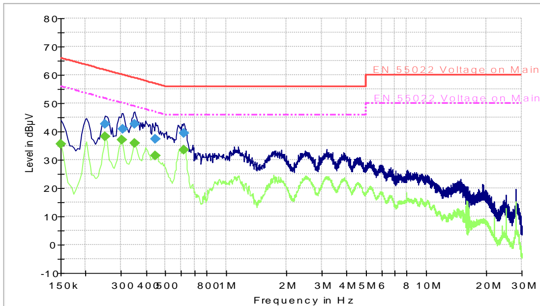
CISPR 22 Mains Conducted FCC_LISN
