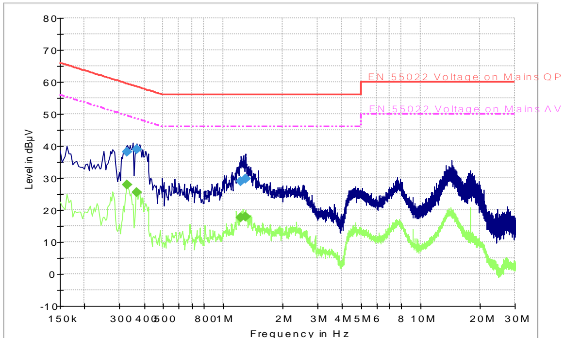
CISPR 22 Mains Conducted FCC_LISN
