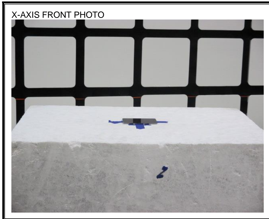
RADIATED RF MEASUREMENT SETUP FOR PORTABLE CONFIGURATION
