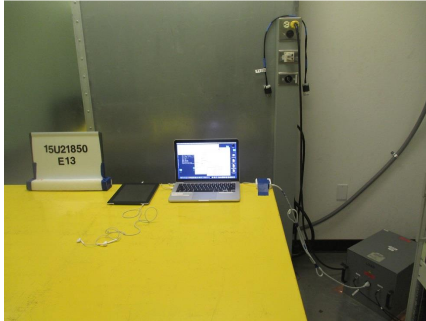
EUT WITH LAPTOP LINE CONDUCTED FRONT PHOTO
