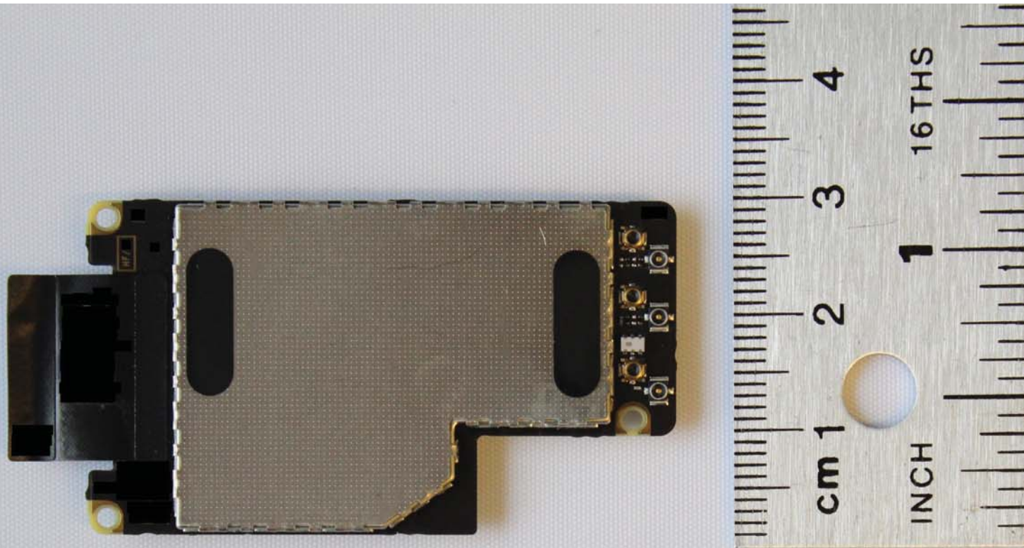
A1430 - Photo 32 Cellular radio MLB with shields - Back
