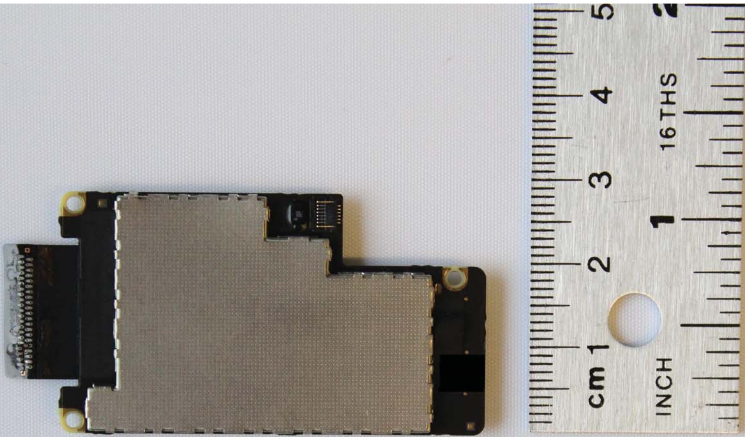
A1430 - Photo 31 Cellular radio MLB with shield - Front
