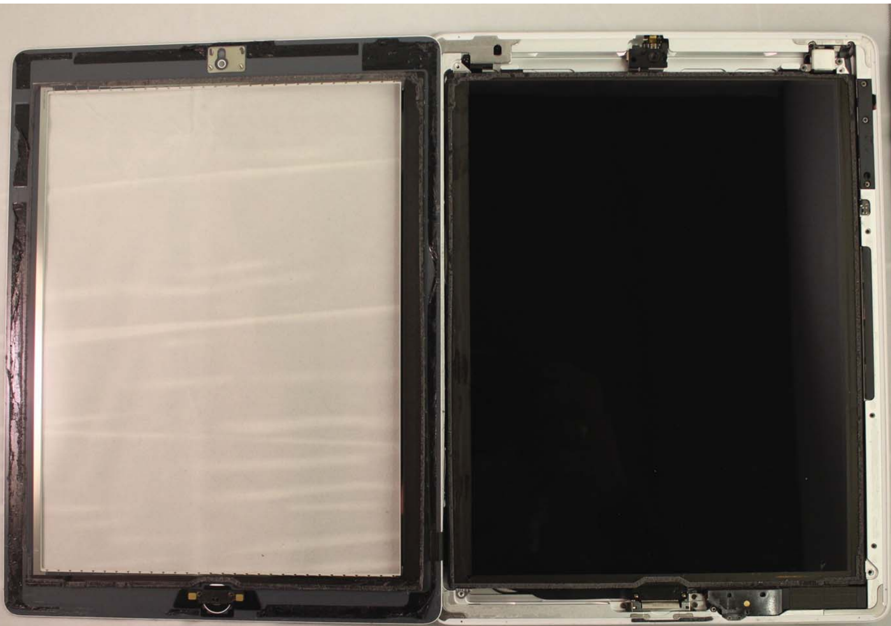
A1416 - Photo 1 Front glass removed
