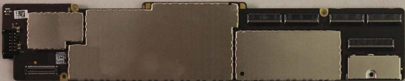
A1416 - Photo 19 Main MLB with shields - Front
