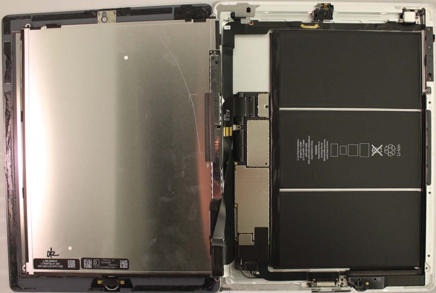
A1416 - Photo 2 LCD Panel removed
