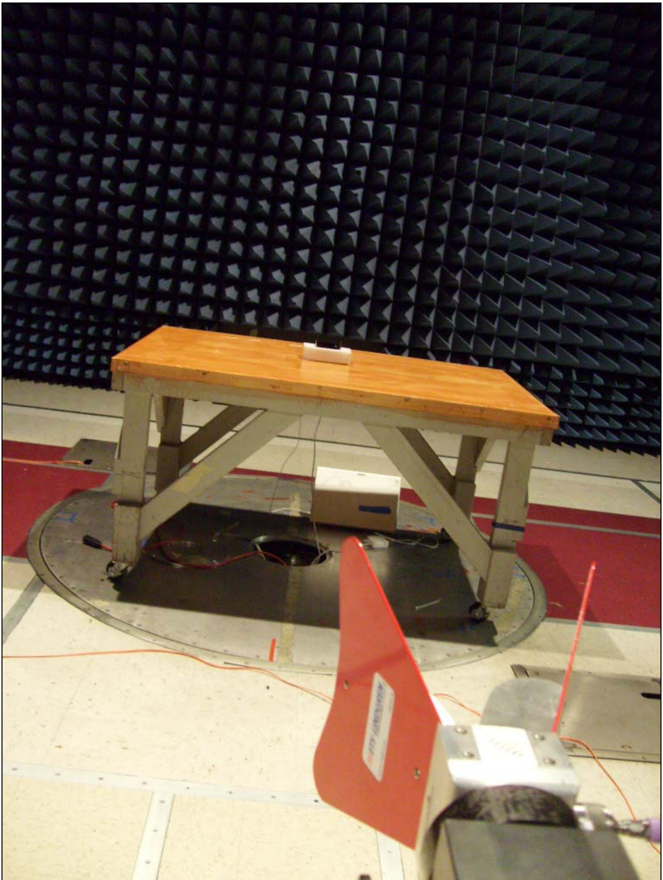
Photograph 4. Radiated Emission (Above 1GHz) @3m
