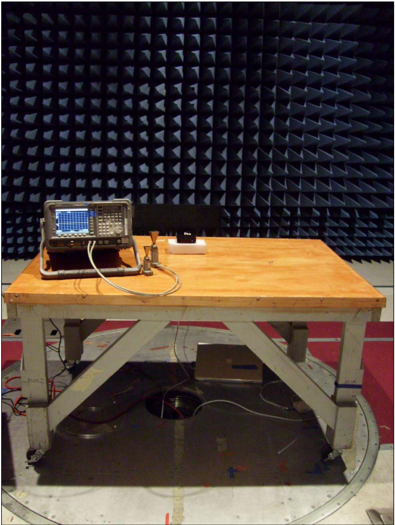
Photograph 2. Radiated Emission (18GHz - 40GHz)
