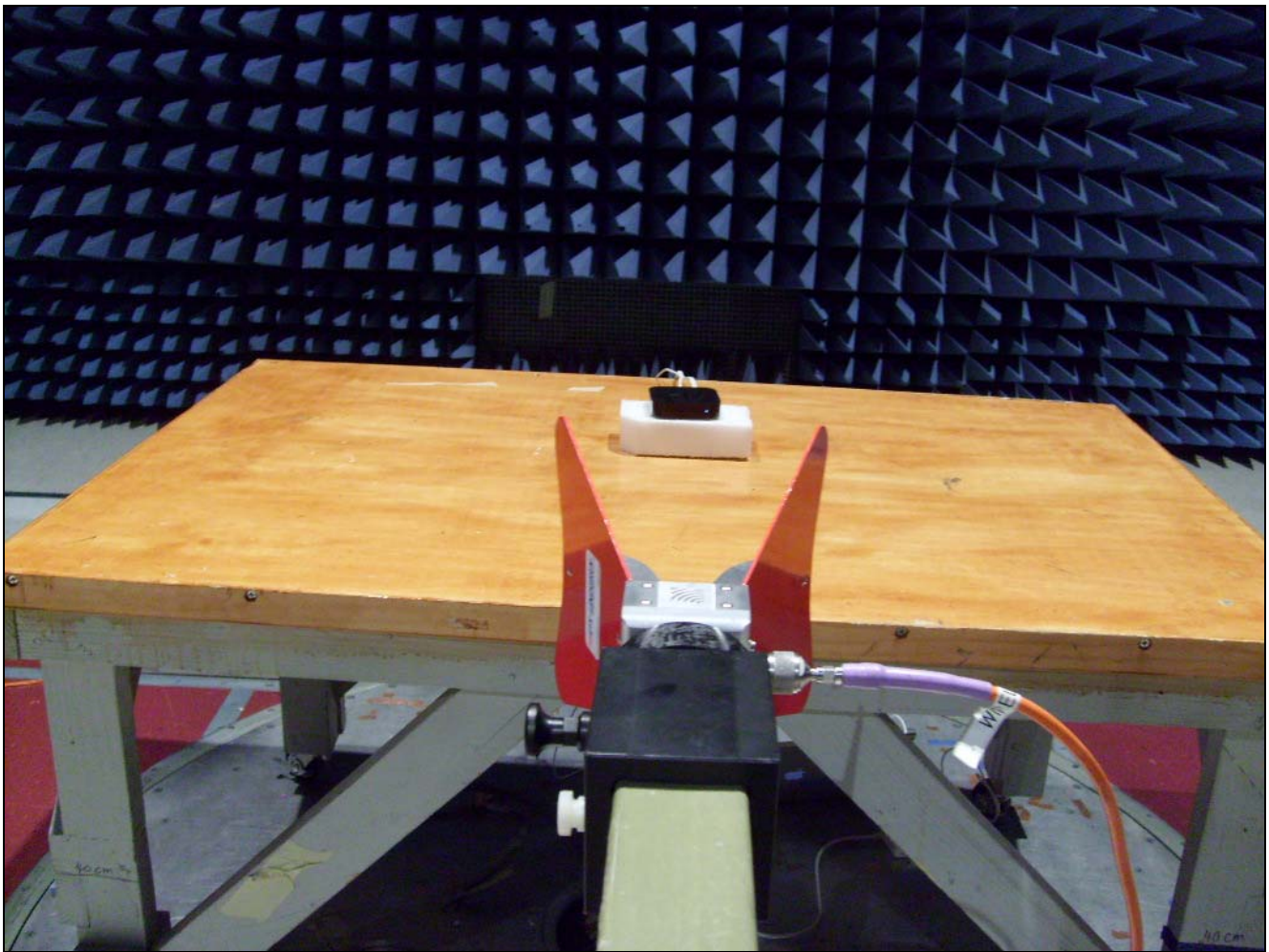
Photograph 3. Radiated Emission (Above 1GHz) @1m
