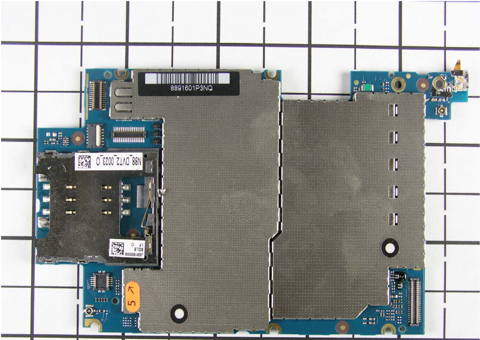
IPHONE INTERIOR PHOTO 4 MAIN PCB TOP SIDE WITH SHIELDS OVER CIRCUITS
