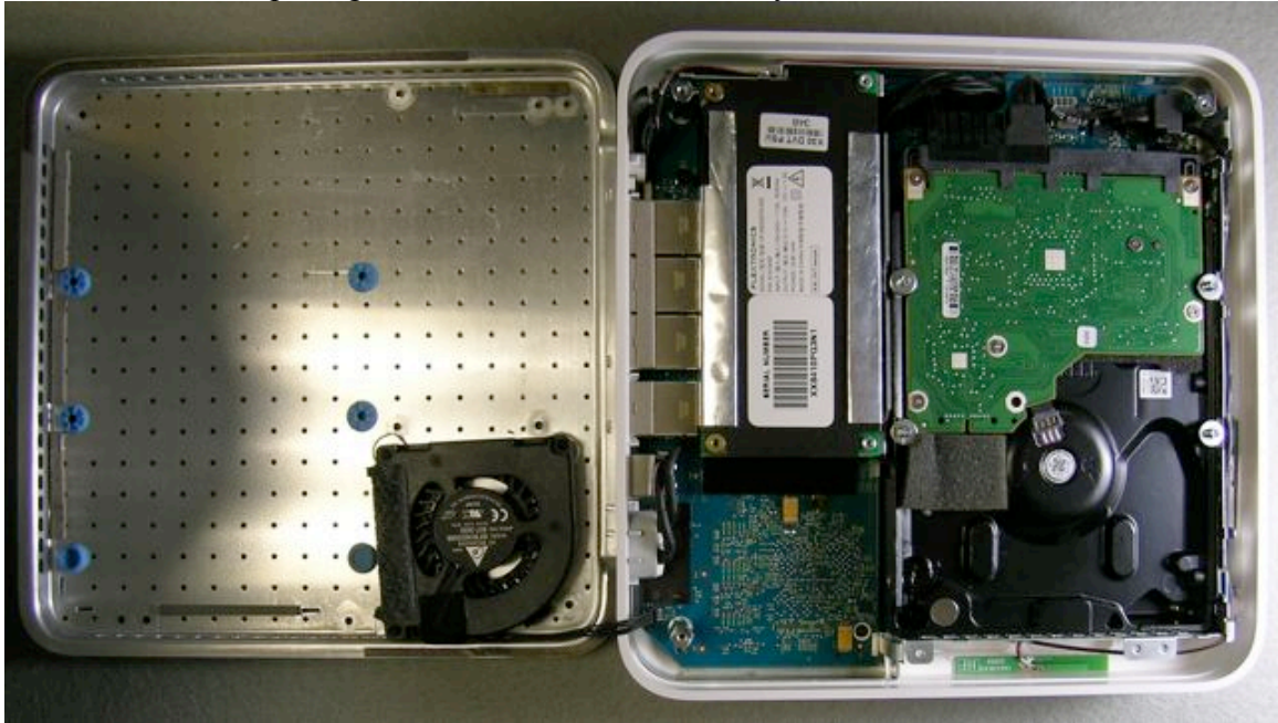
Shield removed exposing enclosure's internal assembly
