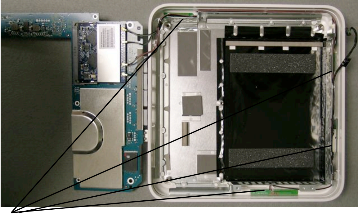
Location of Four Antennas
