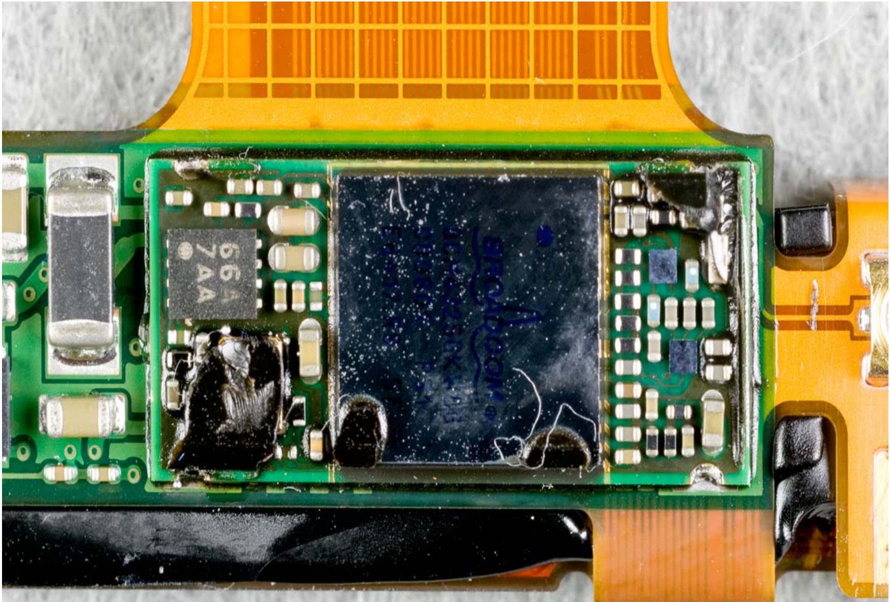
Interior Photo 15 FCC ID: BCGA1288 IC #: 579C-A1288 Touchpad chip shield removed. Closeup view
