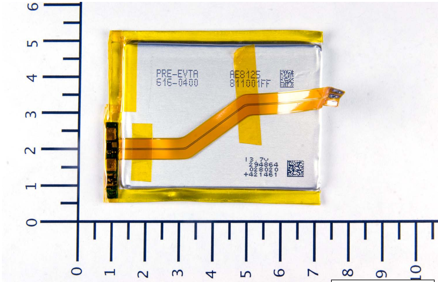
Interior Photo 4 FCC ID: BCGA1288 IC #: 579C-A1288 Battery, and battery flex cable
