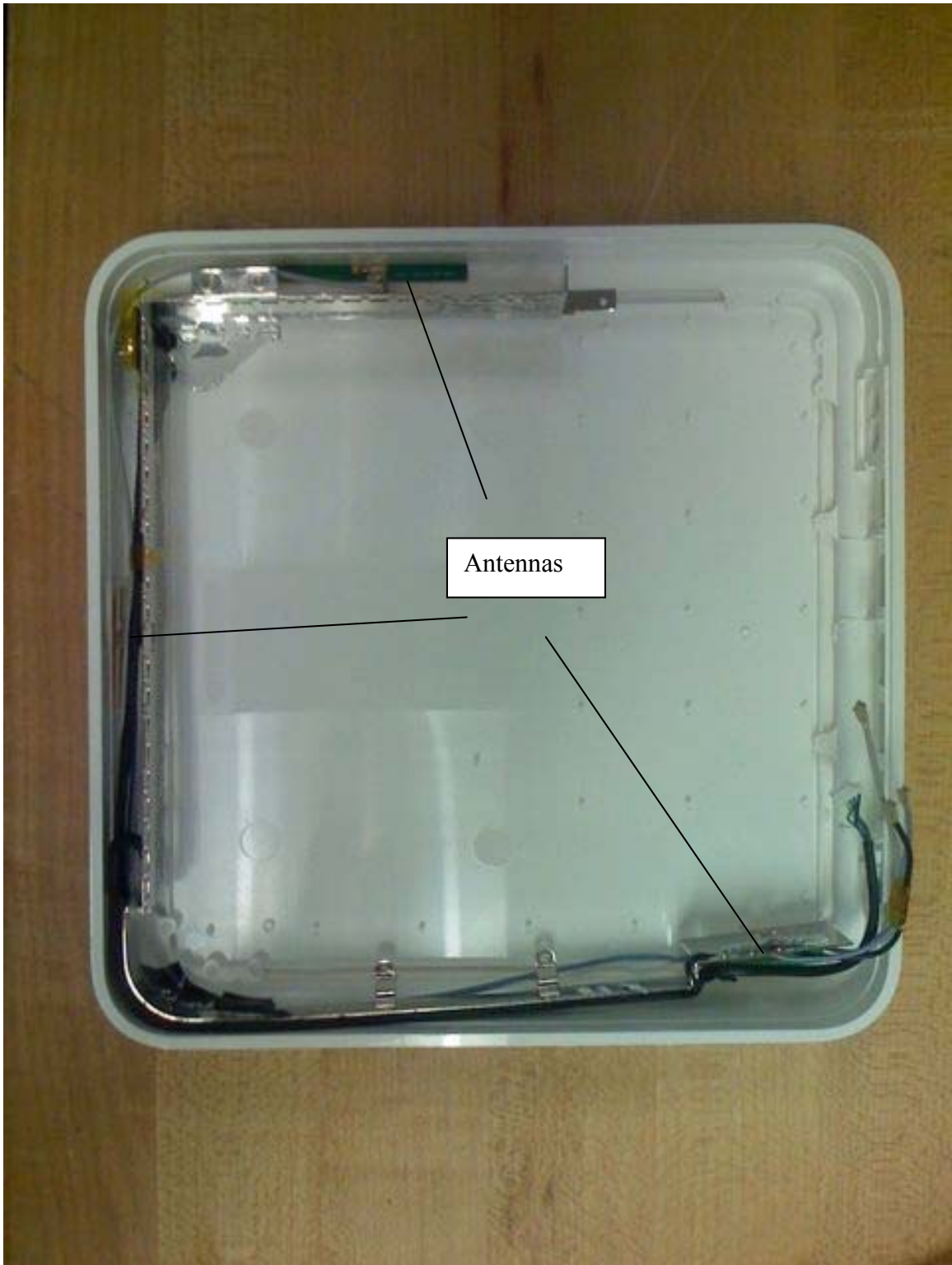
Enclosure with Antenna bracket installed
