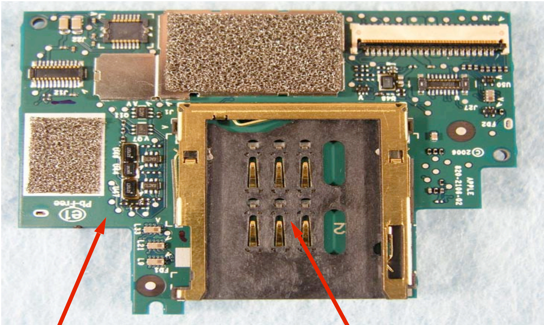
Applications Processor Board
