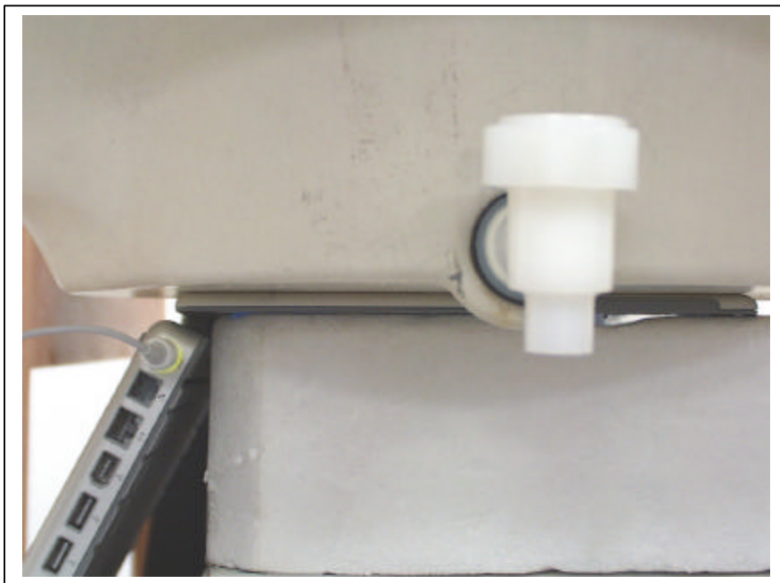
EUT Setup Configuration 2 [12" PowerBook G4 with Inverted F (603-1203) antenna] Spacing between host device and phantom - In contact (0 cm).
