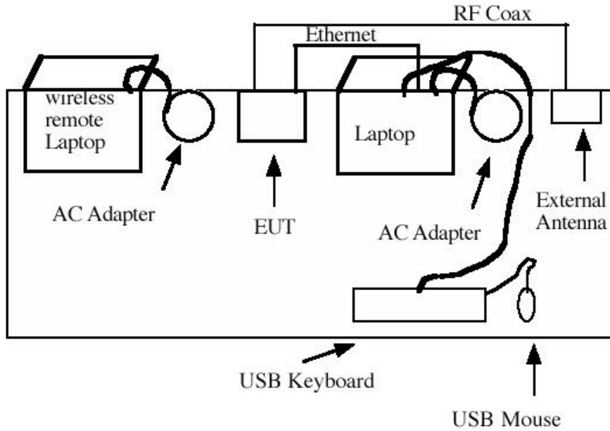
Radiated Test Setup - Top View
