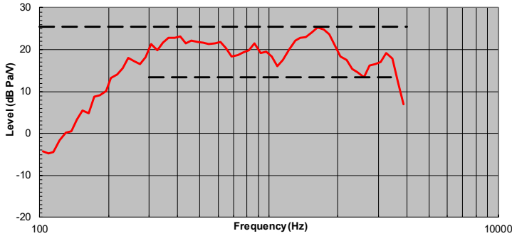
TIA-5050 Free Field Measurement at 8N Receive Frequency Response
