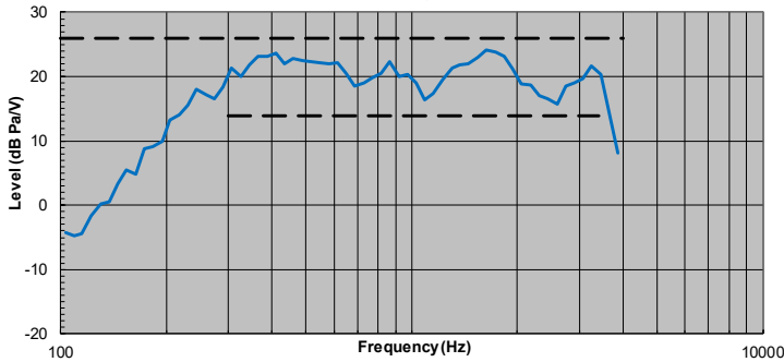
TIA-5050 Diffuse Field Measurement at 8N Receive Frequency Response
