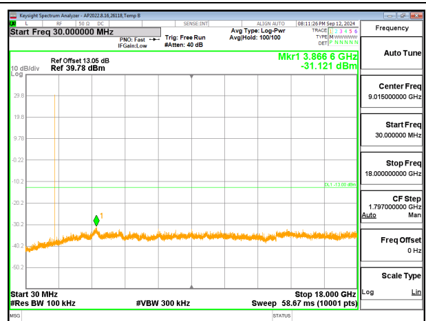
Low Channel 30MHz to 18GHz Ant4
