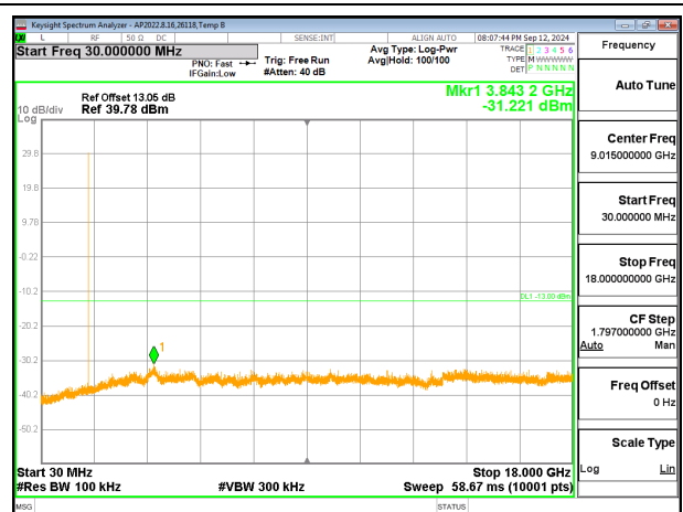
High Channel 30MHz to 18GHz Ant4
