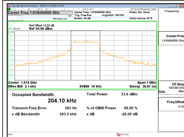
Occupied Bandwidth, Mid Channel, Ant 1
