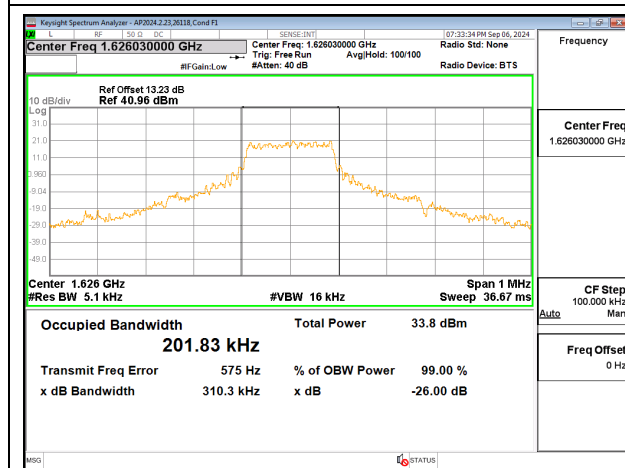
Occupied Bandwidth, High Channel, Ant 1
