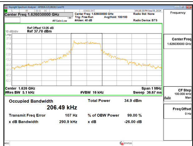
Occupied Bandwidth, High Channel, Ant 4
