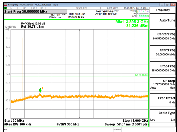
Mid Channel 30MHz to 18GHz Ant4
