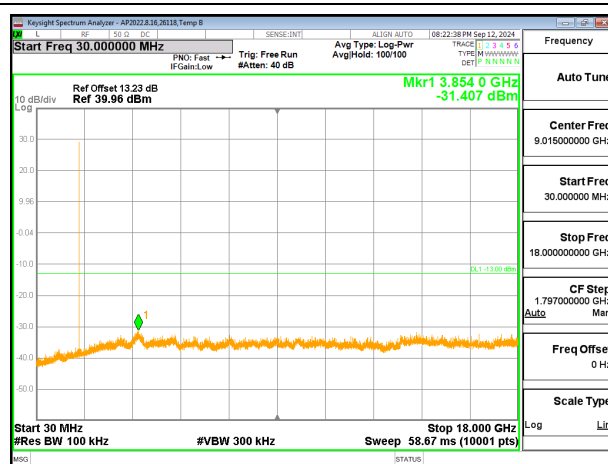
High Channel 30MHz to 18GHz Ant1
