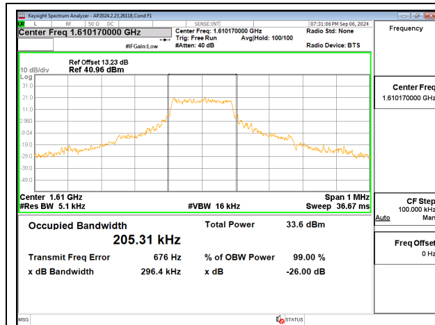
Occupied Bandwidth, Low Channel, Ant 1
