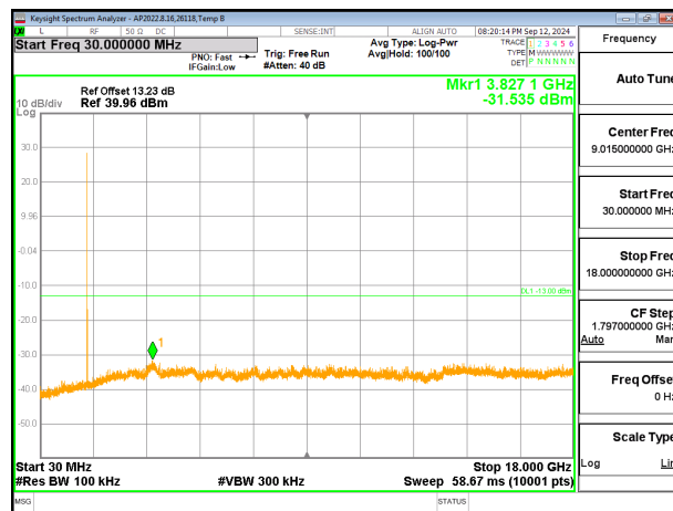
Mid Channel 30MHz to 18GHz Ant1
