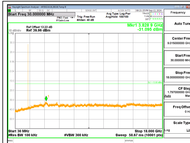
Low Channel 30MHz to 18GHz Ant1
