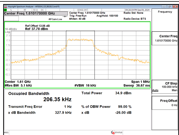
Occupied Bandwidth, Low Channel, Ant 4
