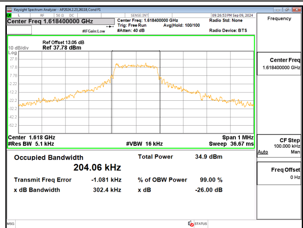
Occupied Bandwidth, Mid Channel, Ant 4
