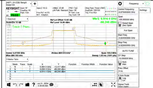
STRADDLE CHANNEL ANT 5 6875
