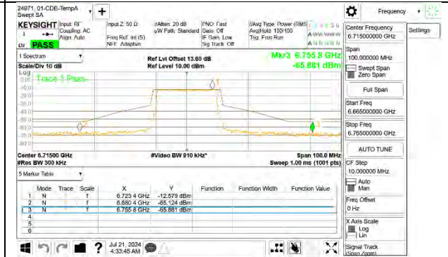
MID CHANNEL ANT 5 6715
