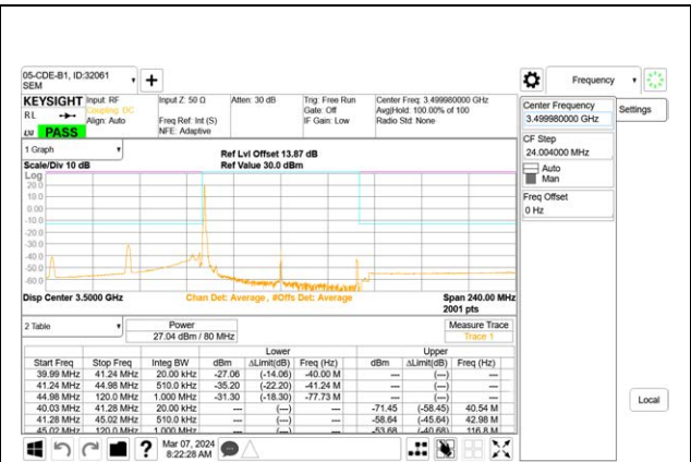
5G NR n77 80MHz BPSK Middle Channel RB1-0
