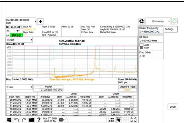
5G NR n77 80MHz BPSK Middle Channel RB1-216
