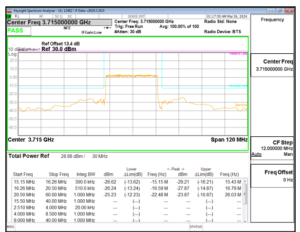
5G NR n77 30MHz BPSK Low Channel RB50-0
