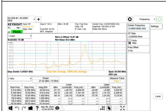
5G NR n77 10MHz BPSK Low Channel RB1-23
