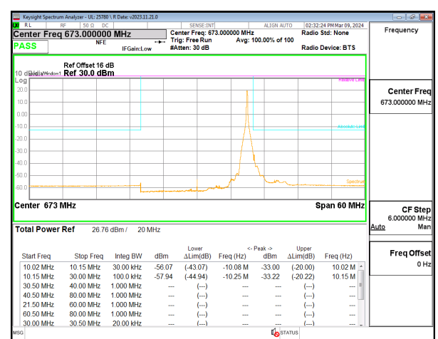
LTE B71 20MHz QPSK Low Channel RB1-99
