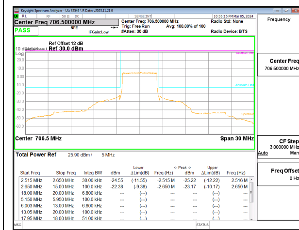
LTE B17 5MHz QPSK Low Channel RB25-0
