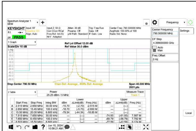
5G NR n14 5MHz BPSK Low Channel RB1-0, ID: 28774
