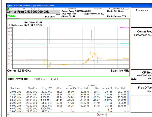
5G NR n7 40MHz BPSK Middle Channel RB1-215, ID:12482
