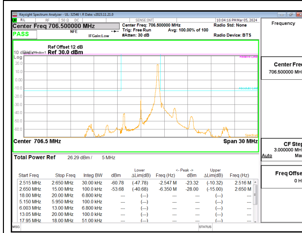
LTE B17 5MHz QPSK Low Channel RB1-24
