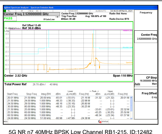
5G NR n7 40MHz BPSK Low Channel RB1-215, ID:12482
