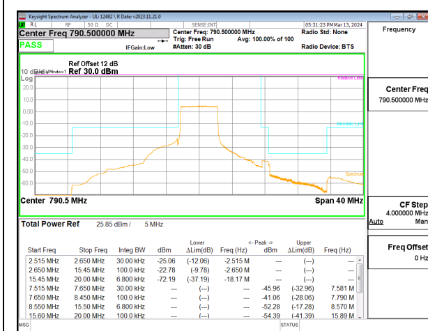
LTE B14 5MHz QPSK Low Channel RB25-0
