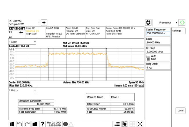
5G NR n26 15MHz BPSK Middle Channel RB75-0
