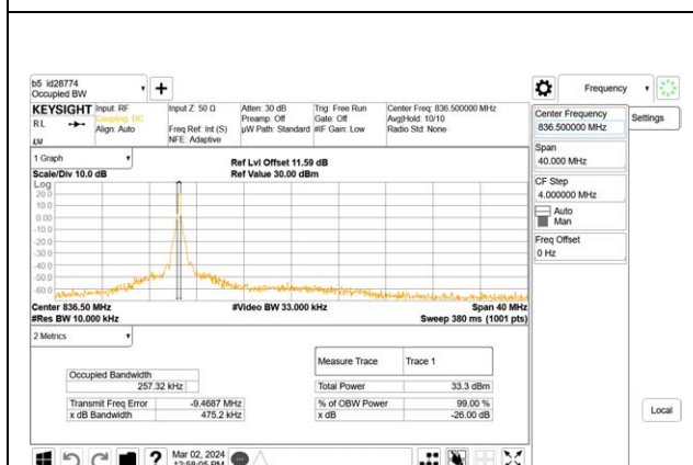
5G NR n26 20MHz Middle High Channel RB1-0
