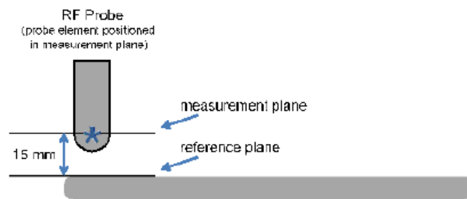
Figure 1 - WD reference and plane for RF emission measurements
