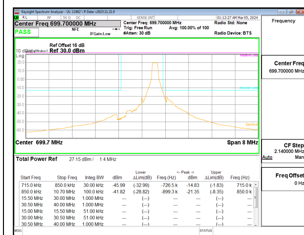
LTE B12 1.4MHz QPSK Low Channel RB1-5
