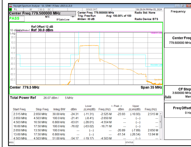
LTE B13 5MHz QPSK Low Channel RB25-0
