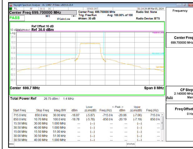
LTE B12 1.4MHz QPSK Low Channel RB6-0
