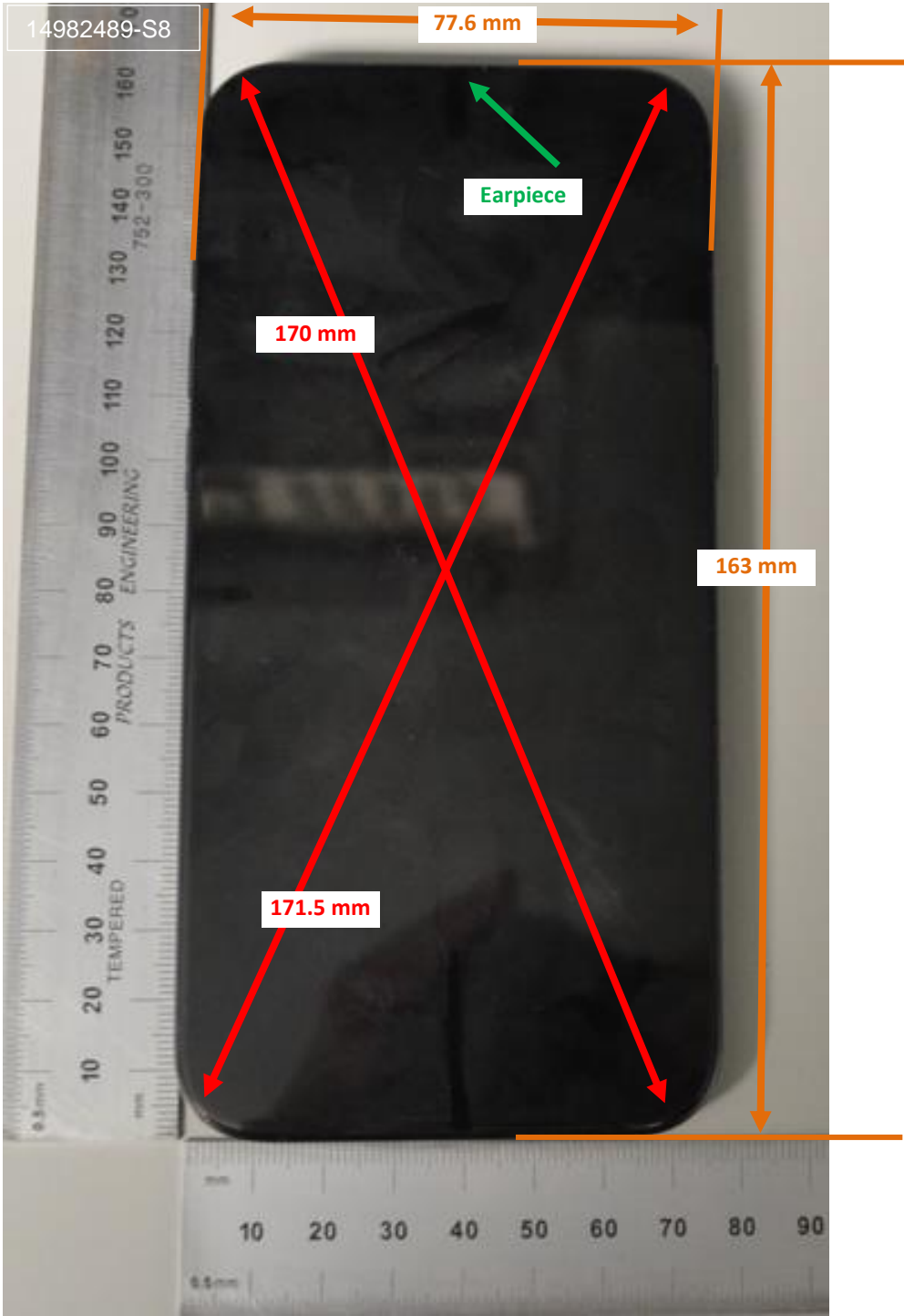
Photograph 1: Overall Dimensions
