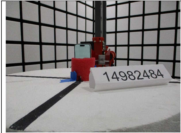
0.96-6Hz (FRONT)
