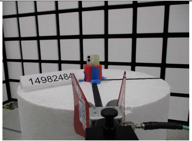
0.96-6GHz (BACK)
