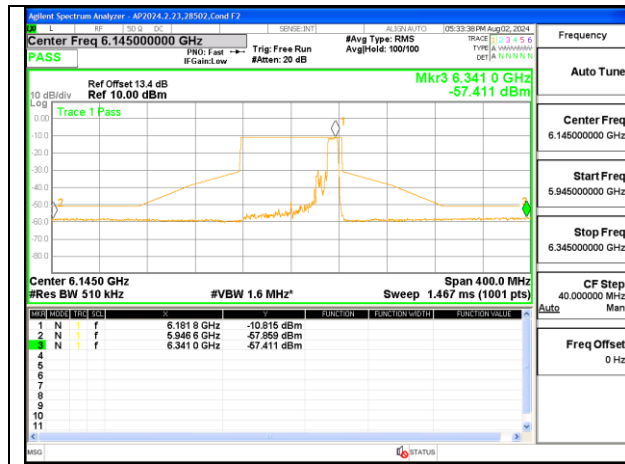
LOW CHANNEL 6145
