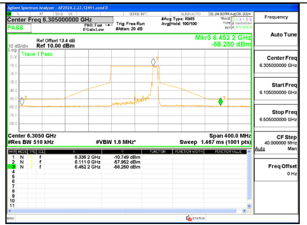
MID CHANNEL 6305
