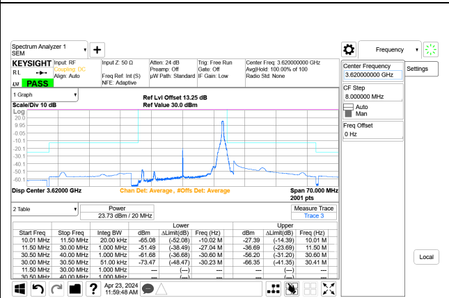
5G NR n48 20MHz QPSK Mid Channel RB1-50 Port A+B, ID:28567
