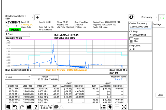
5G NR n48 30MHz QPSK Low Channel RB1-0 Port A+B, ID:28567
