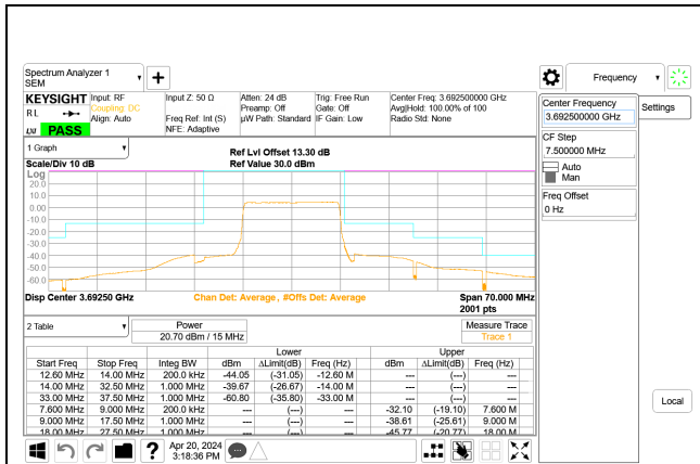
5G NR n48 15MHz QPSK High Channel RB38-0 Port A, ID:28567
