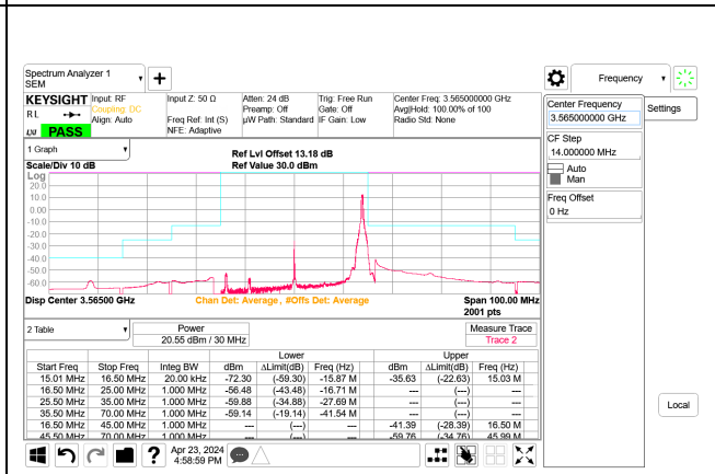
5G NR n48 30MHz QPSK Low Channel RB1-77 Port B, ID:28567
