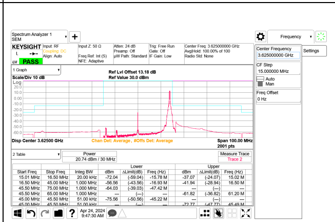
5G NR n48 30MHz QPSK Mid Channel RB1-77 Port B, ID:28567
