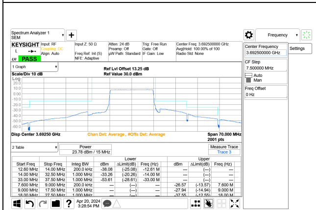
5G NR n48 15MHz QPSK High Channel RB38-0 Port A+B, ID:28567
