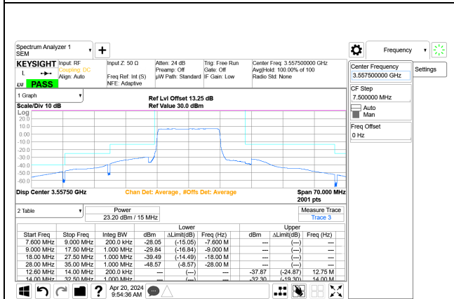
5G NR n48 15MHz QPSK Low Channel RB38-0 Port A+B, ID:28567
