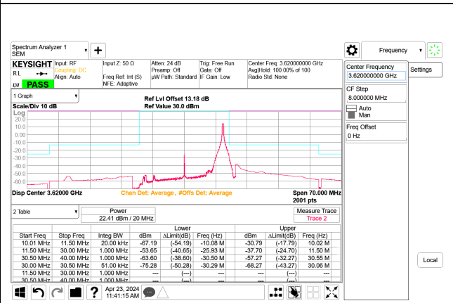
5G NR n48 20MHz QPSK Mid Channel RB1-50 Port B, ID:28567
