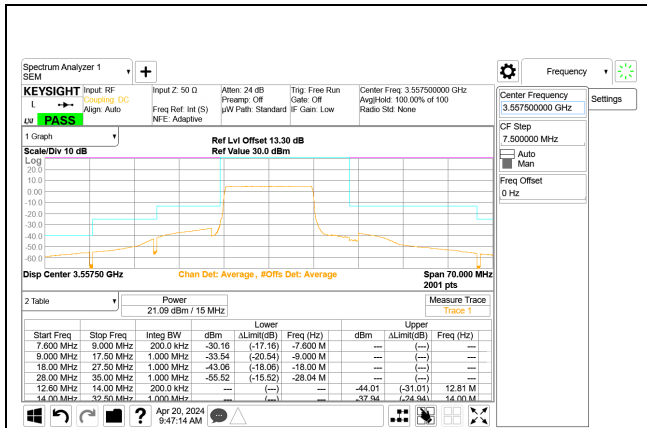
5G NR n48 15MHz QPSK Low Channel RB38-0 Port A, ID:28567
