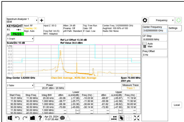
5G NR n48 20MHz QPSK Middle Channel RB1-0 Port A, ID:28567
