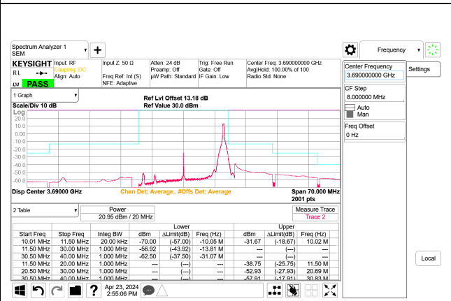
5G NR n48 20MHz QPSK High Channel RB1-50 Port B, ID:28567
