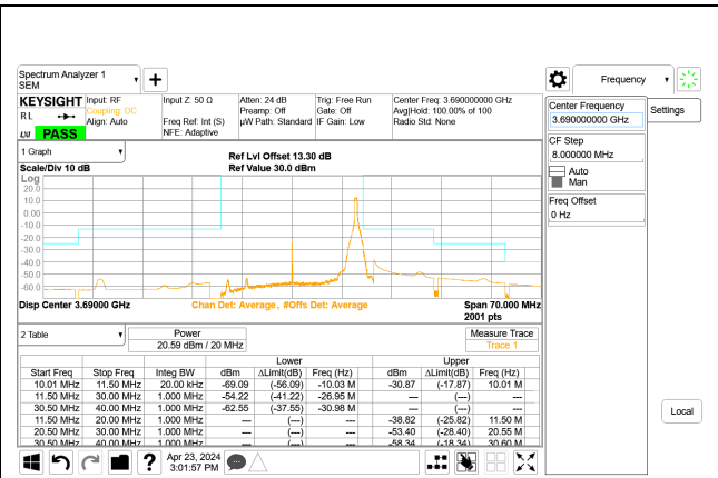
5G NR n48 20MHz QPSK High Channel RB1-50 Port A, ID:28567
