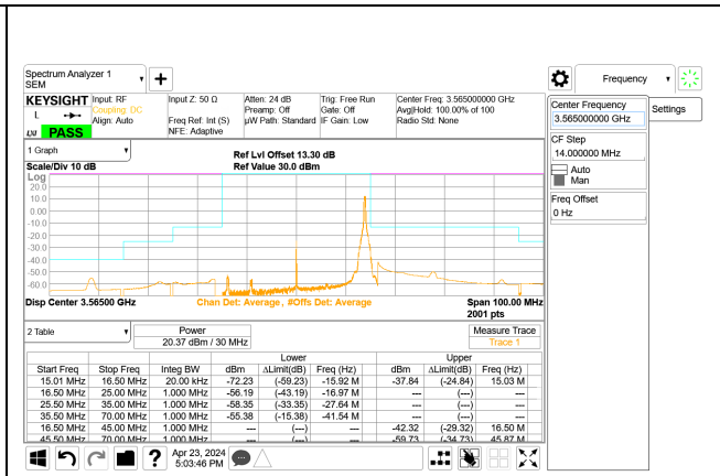
5G NR n48 30MHz QPSK Low Channel RB1-77 Port A, ID:28567
