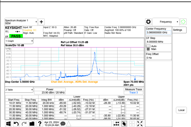
5G NR n48 20MHz QPSK Low Channel RB1-50 Port A+B, ID:28567
