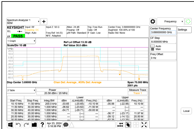
5G NR n48 20MHz QPSK High Channel RB51-0 Port A, ID:28567
