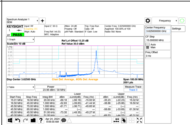
5G NR n48 30MHz QPSK Mid Channel RB1-77 Port A+B, ID:28567
