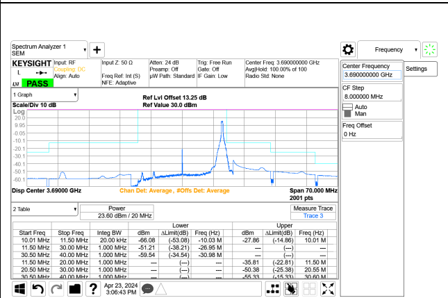
5G NR n48 20MHz QPSK High Channel RB1-50 Port A+B, ID:28567
