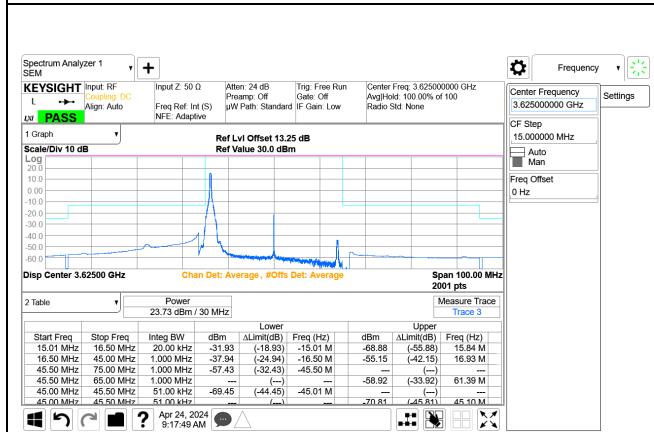
5G NR n48 30MHz QPSK Middle Channel RB1-0 Port A+B, ID:28567
