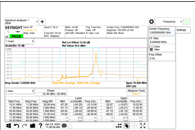
5G NR n48 20MHz QPSK Mid Channel RB1-50 Port A, ID:28567
