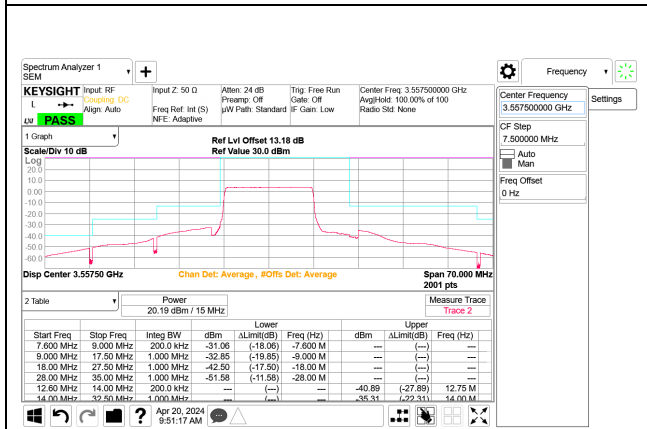
5G NR n48 15MHz QPSK Low Channel RB38-0 Port B, ID:28567
