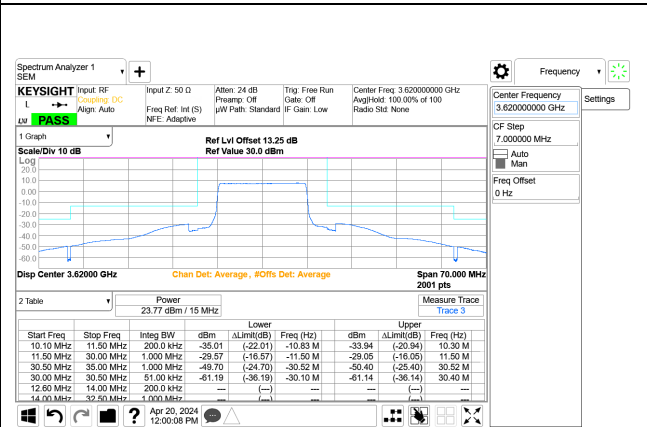
5G NR n48 15MHz QPSK Mid Channel RB38-0 Port A+B, ID:28567
