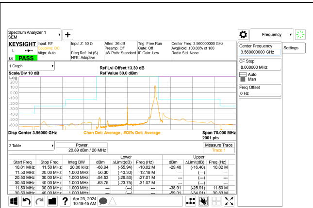
5G NR n48 20MHz QPSK Low Channel RB1-50 Port A, ID:28567
