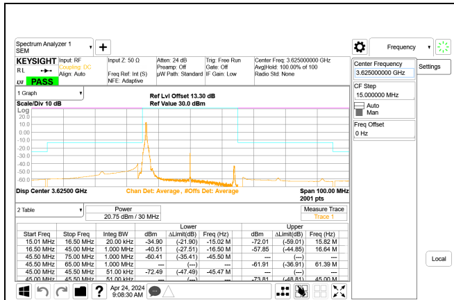
5G NR n48 30MHz QPSK Middle Channel RB1-0 Port A, ID:28567
