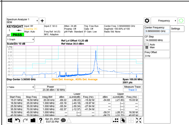
5G NR n48 30MHz QPSK Low Channel RB1-77 Port A+B, ID:28567
