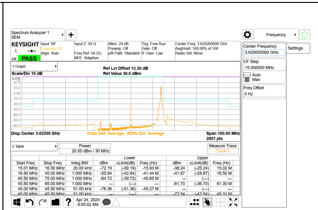
5G NR n48 30MHz QPSK Mid Channel RB1-77 Port A, ID:28567
