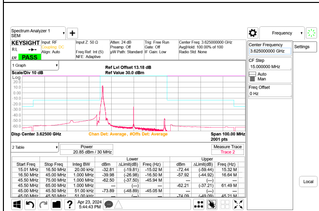
5G NR n48 30MHz QPSK Middle Channel RB1-0 Port B, ID:28567
