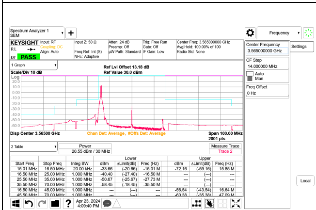
5G NR n48 30MHz QPSK Low Channel RB1-0 Port B, ID:28567
