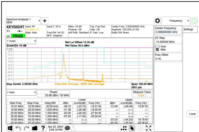
5G NR n48 30MHz QPSK Low Channel RB1-0 Port A, ID:28567
