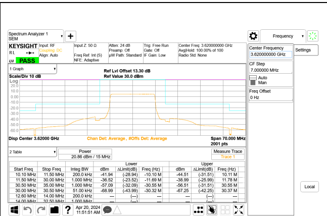
5G NR n48 15MHz QPSK Mid Channel RB38-0 Port A, ID:28567
