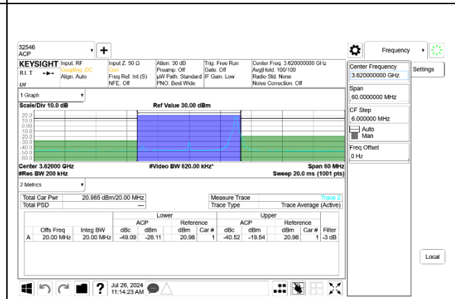
5G NR n48 20MHz BPSK Mid Channel RB1-50 Port B
