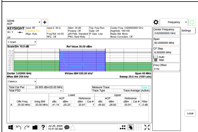
5G NR n48 20MHz BPSK Mid Channel RB1-0 Port B
