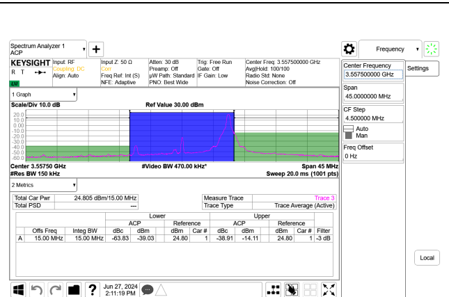
5G NR n48 15MHz QPSK Low Channel RB1-37 Port A+B, ID:32546
