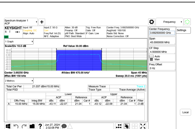
5G NR n48 15MHz BPSK High Channel RB38-0 Port B, ID:32546
