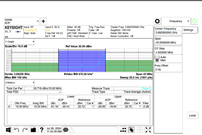
5G NR n48 15MHz BPSK High Channel RB1-37 Port B
