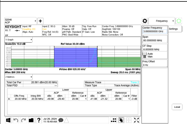
5G NR n48 20MHz BPSK High Channel RB1-50 Port B
