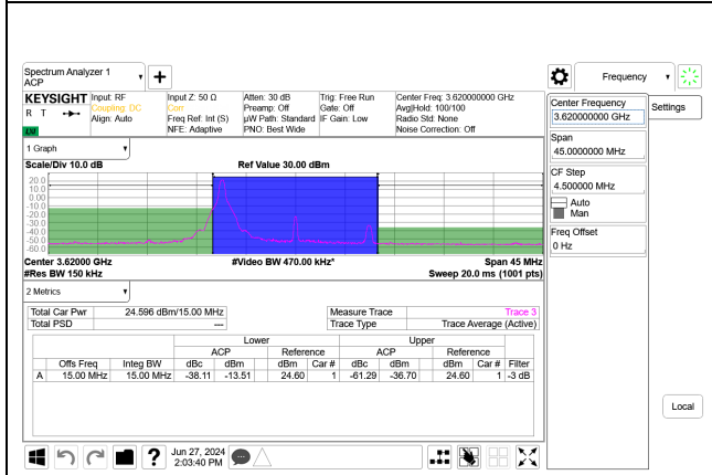
5G NR n48 15MHz BPSK Mid Channel RB1-0 Port A+B, ID:32546
