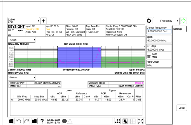
5G NR n48 20MHz BPSK Mid Channel RB1-50 Port A+B
