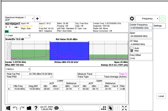
5G NR n48 15MHz QPSK Low Channel RB1-0 Port A+B, ID:32546
