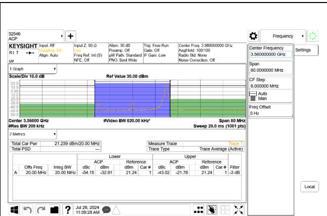
5G NR n48 20MHz BPSK Low Channel RB1-50 Port A
