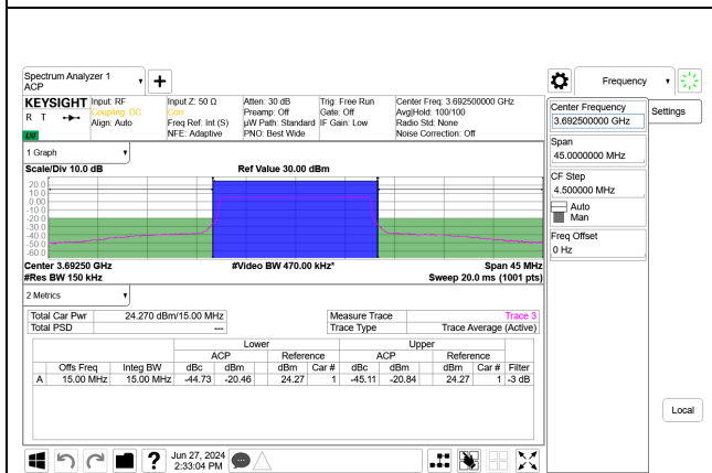
5G NR n48 15MHz BPSK High Channel RB38-0 Port A+B, ID:32546
