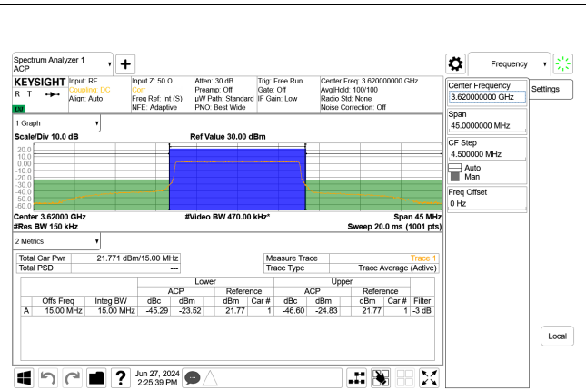
5G NR n48 15MHz BPSK Mid Channel RB38-0 Port A, ID:32546
