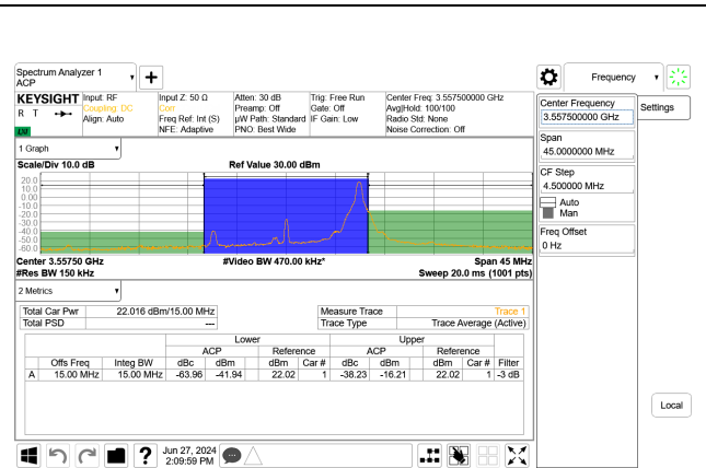
5G NR n48 15MHz QPSK Low Channel RB1-37 Port A, ID:32546
