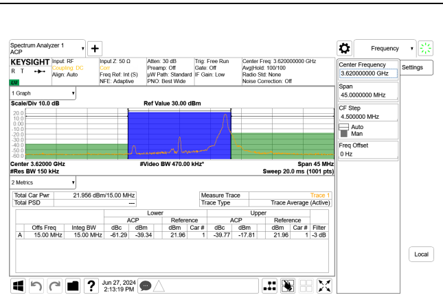
5G NR n48 15MHz BPSK Mid Channel RB1-37 Port A, ID:32546
