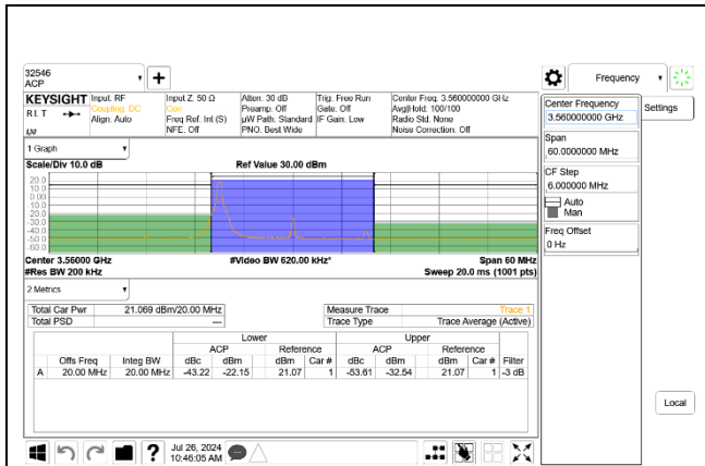
5G NR n48 20MHz BPSK Low Channel RB1-0 Port A
