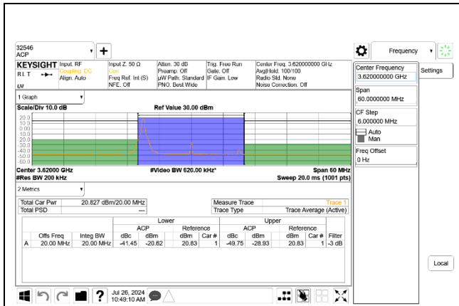
5G NR n48 20MHz BPSK Mid Channel RB1-0 Port A
