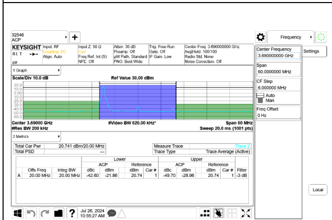
5G NR n48 20MHz BPSK High Channel RB1-0 Port B
