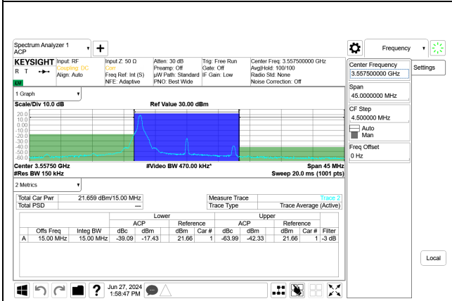
5G NR n48 15MHz QPSK Low Channel RB1-0 Port B, ID:32546
