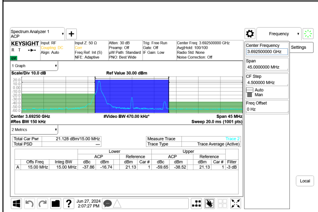
5G NR n48 15MHz BPSK High Channel RB1-0 Port B, ID:32546
