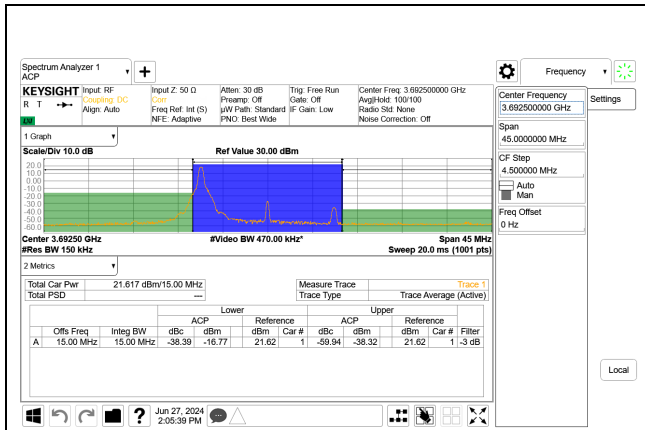
5G NR n48 15MHz BPSK High Channel RB1-0 Port A, ID:32546
