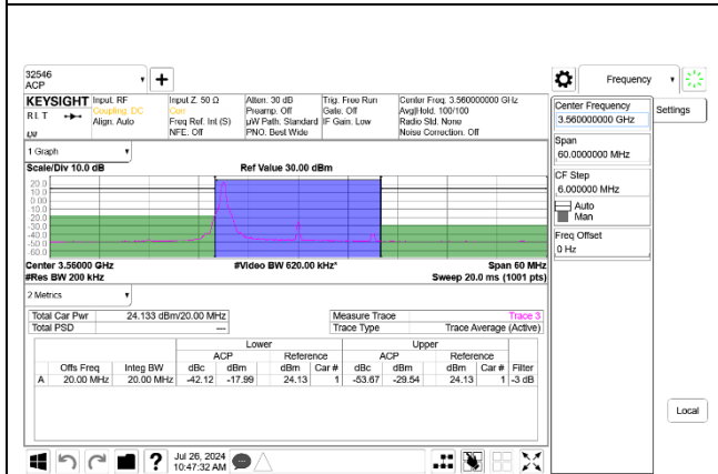
5G NR n48 20MHz BPSK Low Channel RB1-0 Port A+B
