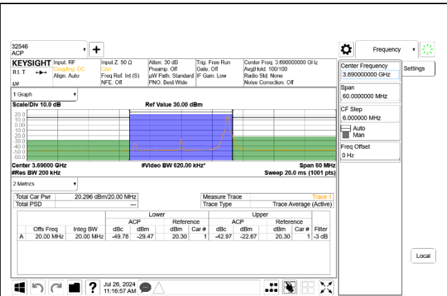
5G NR n48 20MHz BPSK High Channel RB1-50 Port A
