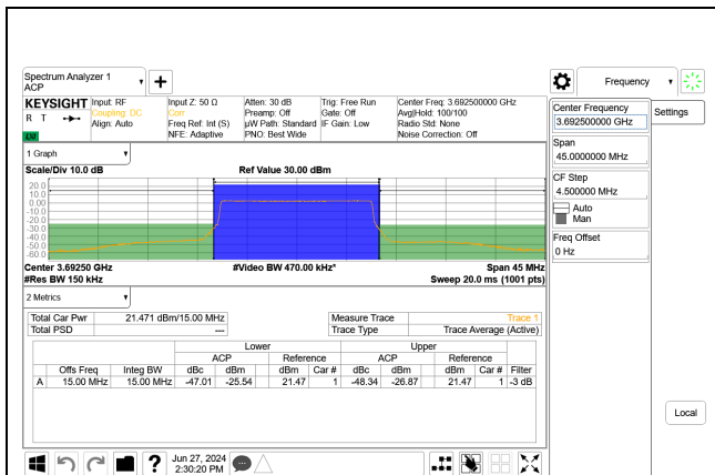
5G NR n48 15MHz BPSK High Channel RB38-0 Port A, ID:32546
