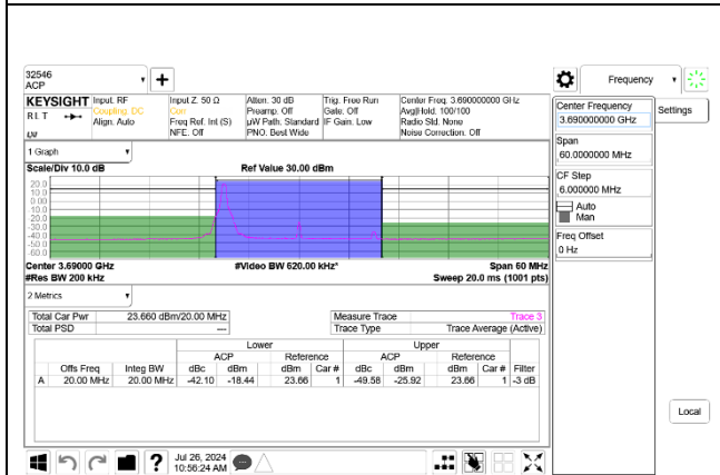
5G NR n48 20MHz BPSK High Channel RB1-0 Port A+B
