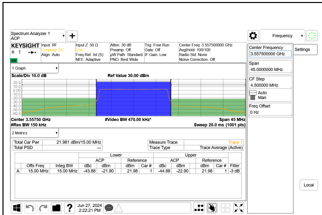
5G NR n48 15MHz BPSK Low Channel RB38-0 Port A, ID:32546
