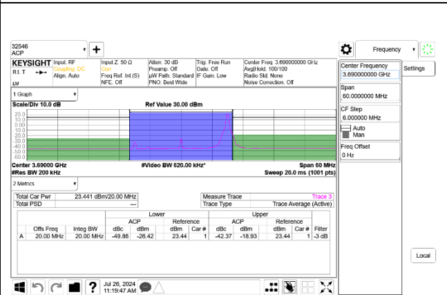
5G NR n48 20MHz BPSK High Channel RB1-50 Port A+B
