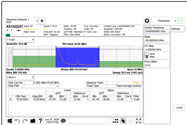
5G NR n48 15MHz BPSK Mid Channel RB1-0 Port A, ID:32546
