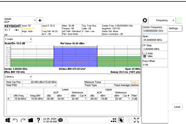
5G NR n48 15MHz BPSK High Channel RB1-37 Port A
