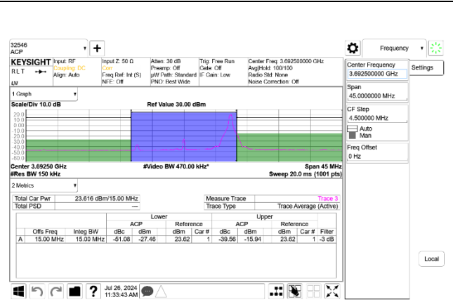
5G NR n48 15MHz BPSK High Channel RB1-37 Port A+B
