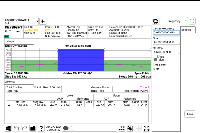
5G NR n48 15MHz BPSK Mid Channel RB38-0 Port A+B, ID:32546
