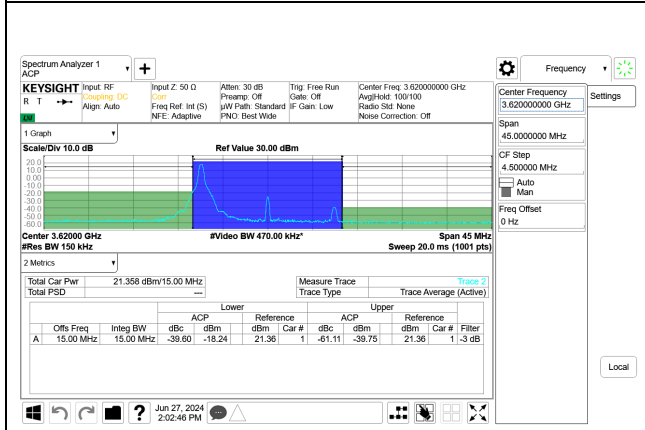
5G NR n48 15MHz BPSK Mid Channel RB1-0 Port B, ID:32546
