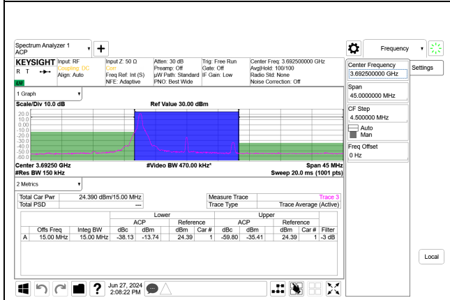
5G NR n48 15MHz BPSK High Channel RB1-0 Port A+B, ID:32546
