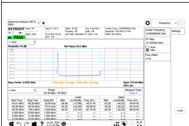
5G NR n77 90MHz BPSK High Channel RB1-0 Port A+B
