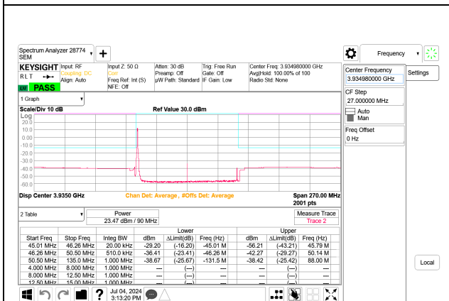
5G NR n77 90MHz BPSK High Channel RB1-0 Port B
