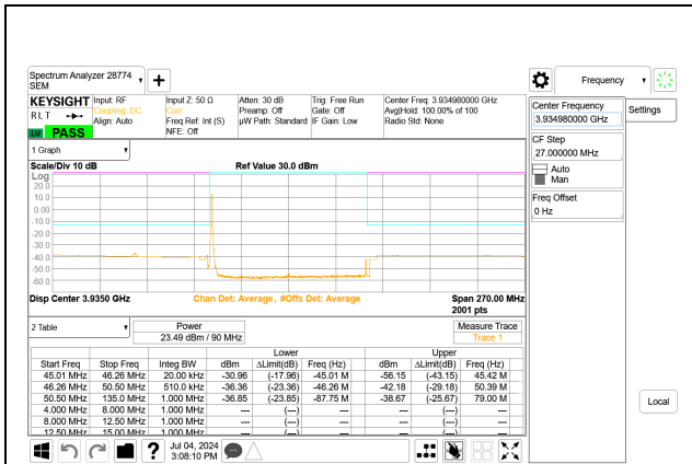
5G NR n77 90MHz BPSK High Channel RB1-0 Port A
