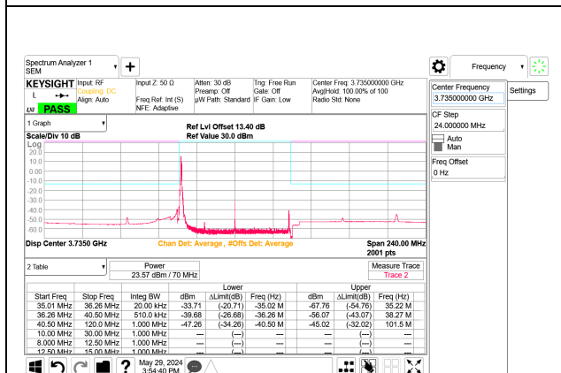
5G NR n77 70MHz BPSK Low Channel RB1-0 Port B ID: 32546
