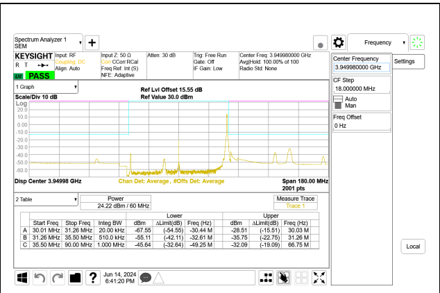
5G NR n77 60MHz BPSK High Channel RB1-161 Port A ID: 28774
