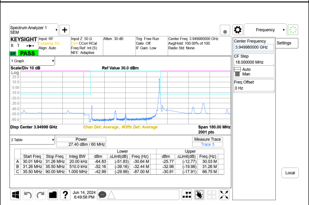
5G NR n77 60MHz BPSK High Channel RB1-161 Port A+B ID: 28774
