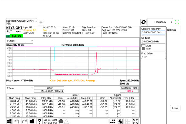
5G NR n77 80MHz BPSK Low Channel RB1-216 Port B
