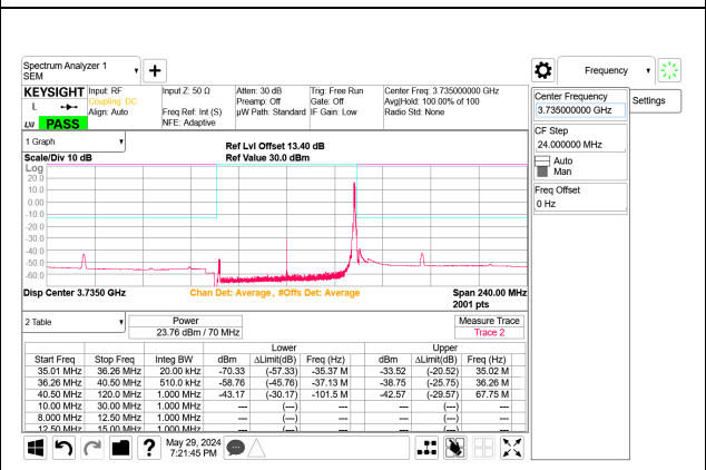
5G NR n77 70MHz BPSK Low Channel RB1-188 Port B ID: 32546
