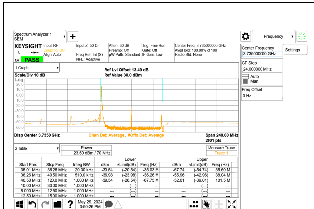
5G NR n77 70MHz BPSK Low Channel RB1-0 Port A ID: 32546
