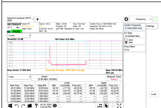
5G NR n77 80MHz BPSK Low Channel RB1-0 Port B
