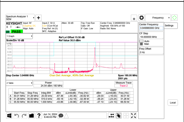
5G NR n77 60MHz BPSK High Channel RB1-161 Port B ID: 28774
