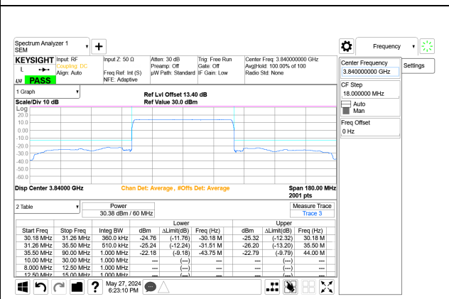
5G NR n77 60MHz BPSK Mid Channel RB162-0 Port A+B ID: 28774
