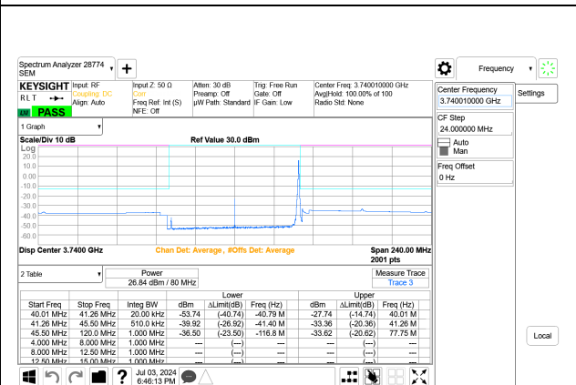
5G NR n77 80MHz BPSK Low Channel RB1-216 Port A+B
