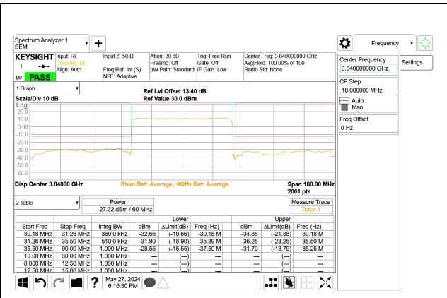
5G NR n77 60MHz BPSK Mid Channel RB162-0 Port A ID: 28774
