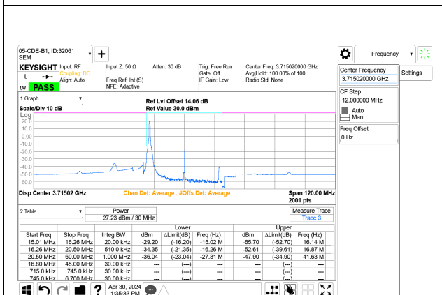
5G NR n77 30MHz BPSK Low Channel RB1-0 Port A+B
