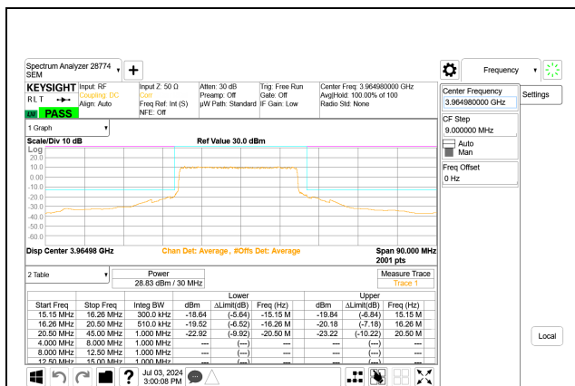
5G NR n77 30MHz BPSK High Channel RB75-0 Port A
