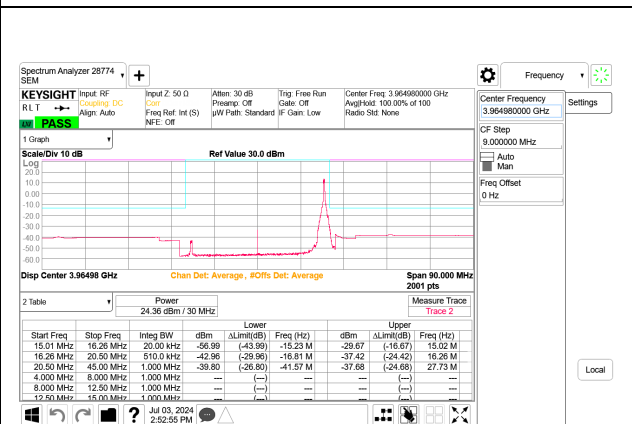
5G NR n77 30MHz BPSK High Channel RB1-77 Port B
