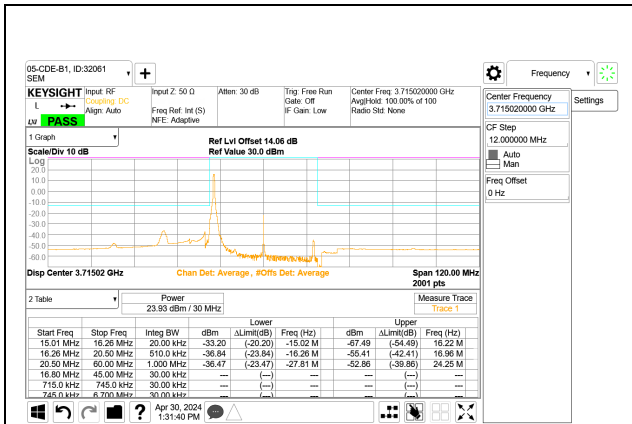
5G NR n77 30MHz BPSK Low Channel RB1-0 Port A
