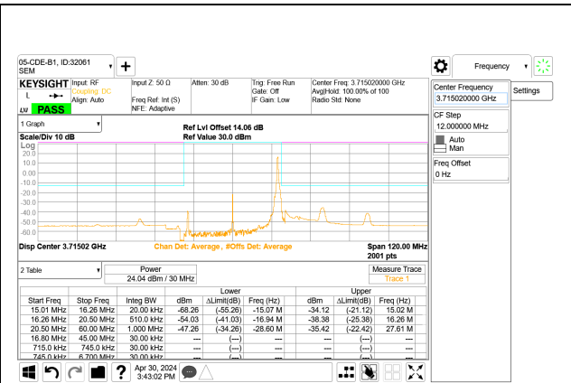
5G NR n77 30MHz BPSK Low Channel RB1-77 Port A
