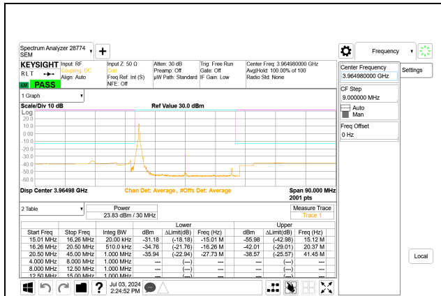
5G NR n77 30MHz BPSK High Channel RB1-0 Port A
