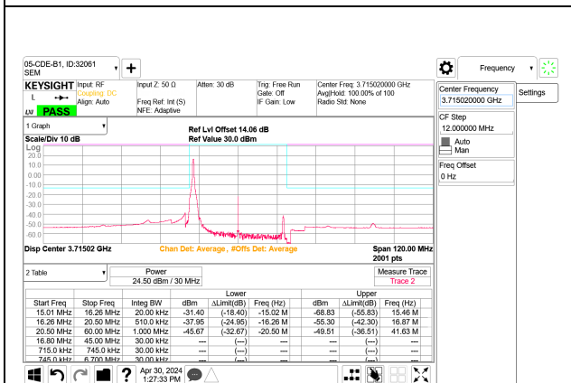
5G NR n77 30MHz BPSK Low Channel RB1-0 Port B
