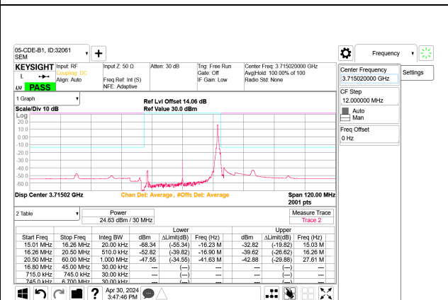
5G NR n77 30MHz BPSK Low Channel RB1-77 Port B
