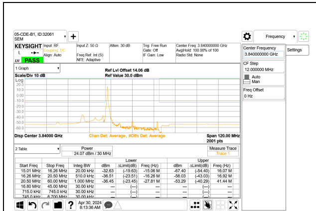
5G NR n77 30MHz BPSK Middle Channel RB1-0 Port A
