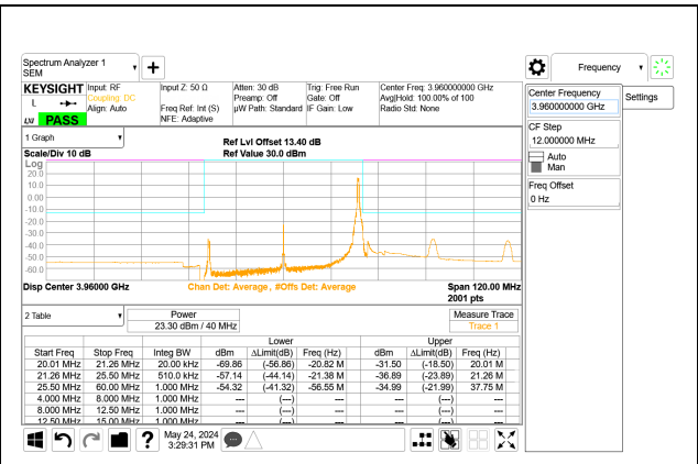
5G NR n77 40MHz BPSK High Channel RB1-105 Port A ID: 32546
