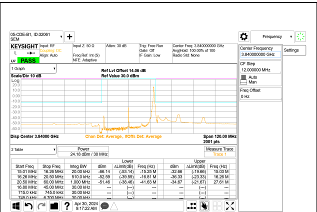
5G NR n77 30MHz BPSK Mid Channel RB1-77 Port A
