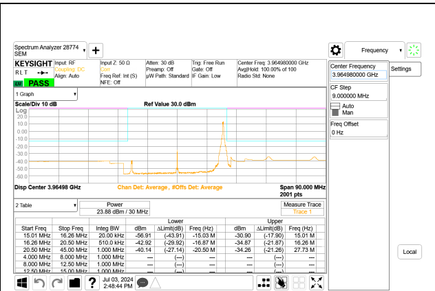
5G NR n77 30MHz BPSK High Channel RB1-77 Port A
