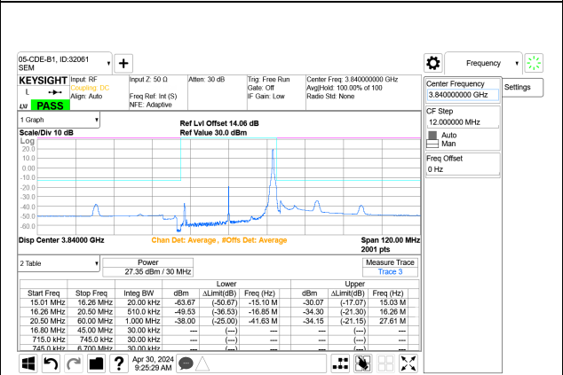
5G NR n77 30MHz BPSK Mid Channel RB1-77 Port A+B
