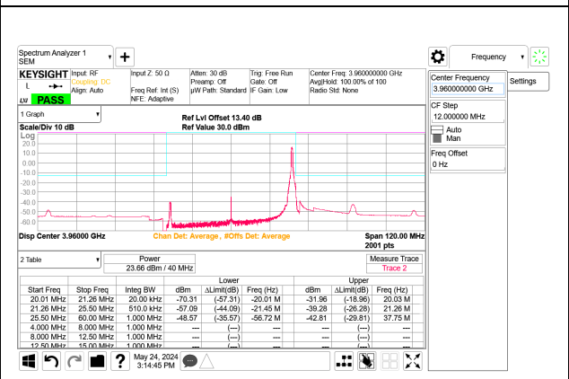
5G NR n77 40MHz BPSK High Channel RB1-105 Port B ID: 32546
