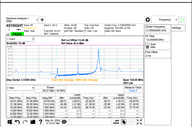
5G NR n77 40MHz BPSK Low Channel RB1-105 Port A+B, ID:32061
