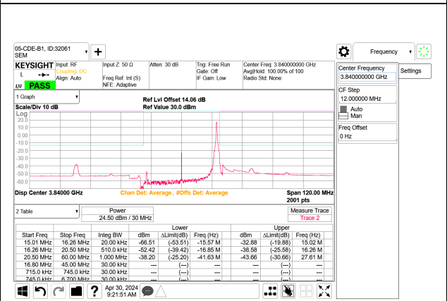
5G NR n77 30MHz BPSK Mid Channel RB1-77 Port B
