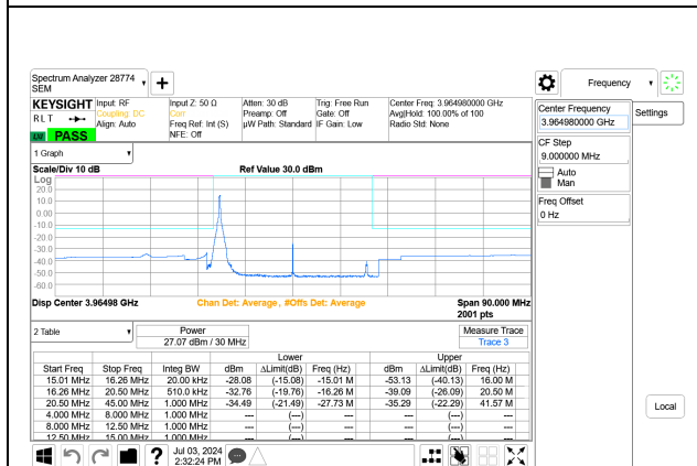
5G NR n77 30MHz BPSK High Channel RB1-0 Port A+B
