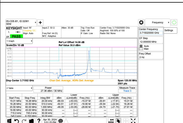
5G NR n77 30MHz BPSK Low Channel RB1-77 Port A+B
