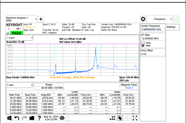
5G NR n77 40MHz BPSK High Channel RB1-105 Port A+B ID: 32546
