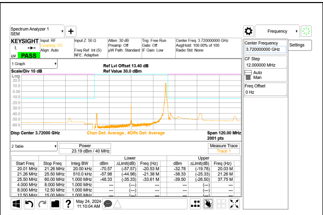
5G NR n77 40MHz BPSK Low Channel RB1-105 Port A, ID:32061
