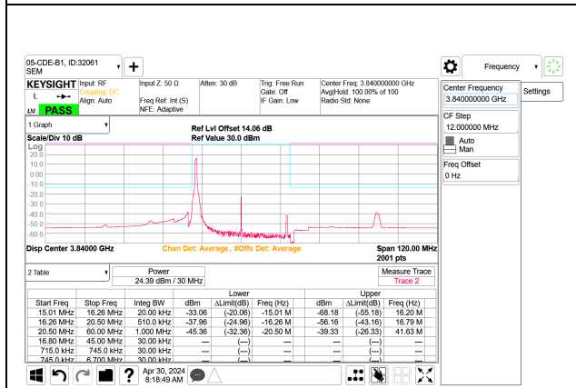
5G NR n77 30MHz BPSK Middle Channel RB1-0 Port B
