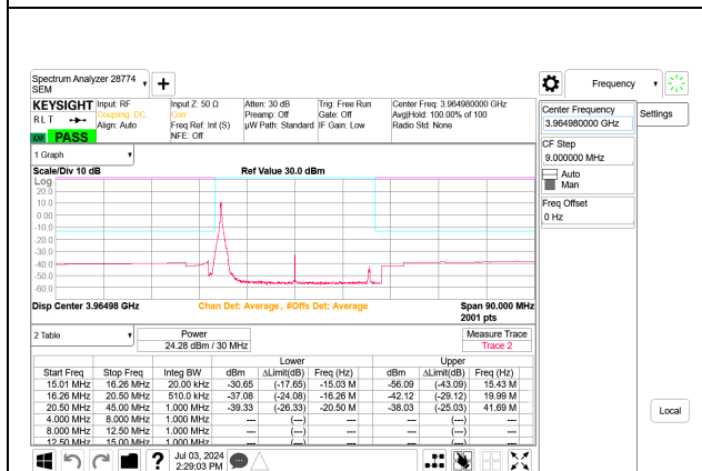
5G NR n77 30MHz BPSK High Channel RB1-0 Port B
