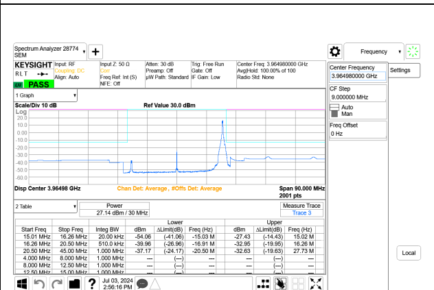
5G NR n77 30MHz BPSK High Channel RB1-77 Port A+B
