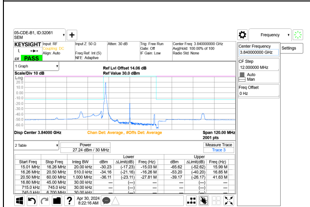
5G NR n77 30MHz BPSK Middle Channel RB1-0 Port A+B
