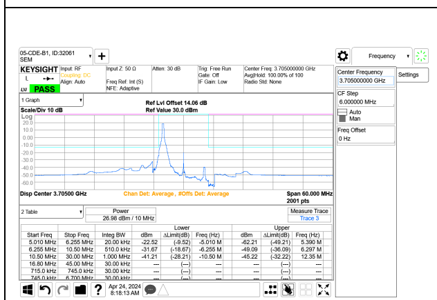
5G NR n77 10MHz BPSK Low Channel RB1-0 Port A+B ID 27342
