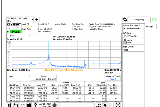
5G NR n77 100MHz BPSK Middle Channel RB1-0 Port A+B
