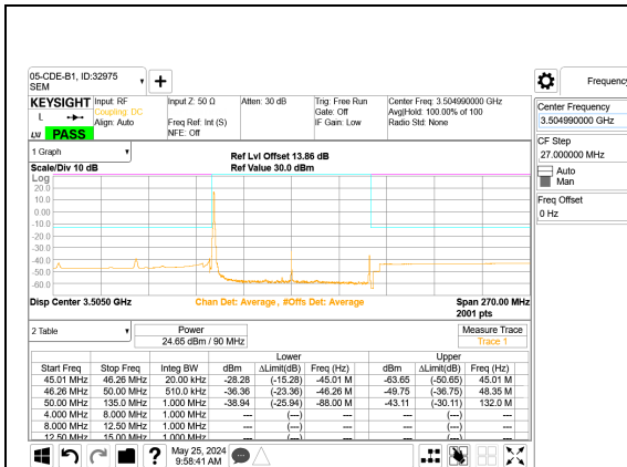
5G NR n77 90MHz BPSK High Channel RB1-0 Port A
