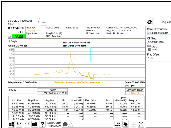
5G NR n77 10MHz BPSK Middle Channel RB1-0 Port A
