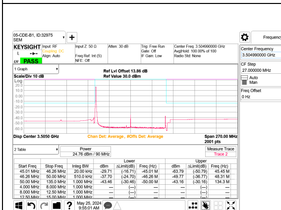
5G NR n77 90MHz BPSK High Channel RB1-0 Port B
