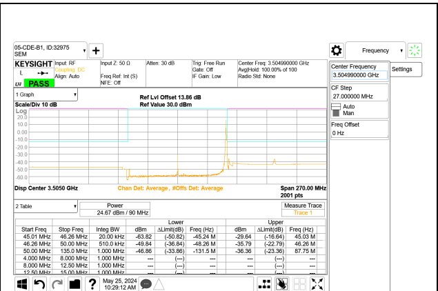
5G NR n77 90MHz BPSK High Channel RB1-244 Port A
