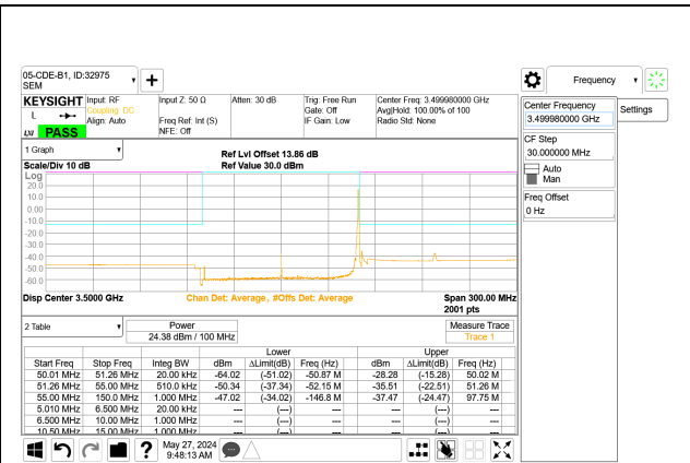
5G NR n77 100MHz BPSK Mid Channel RB1-272 Port A
