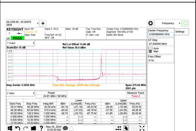
5G NR n77 90MHz BPSK High Channel RB1-244 Port B
