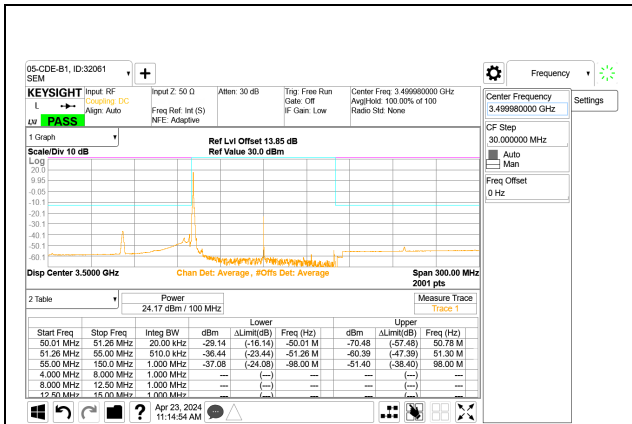
5G NR n77 100MHz BPSK Middle Channel RB1-0 Port A
