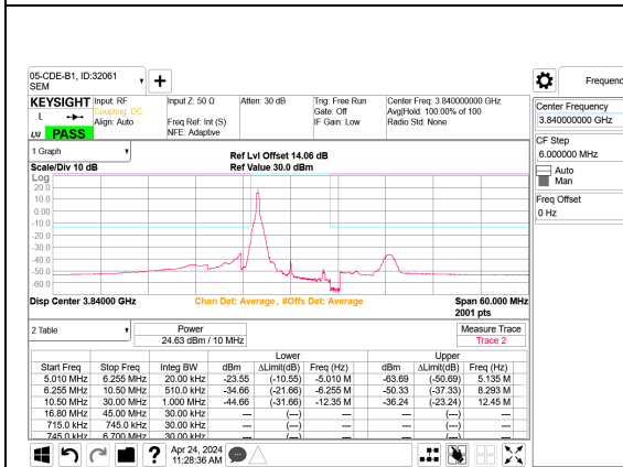
5G NR n77 10MHz BPSK Middle Channel RB1-0 Port B
