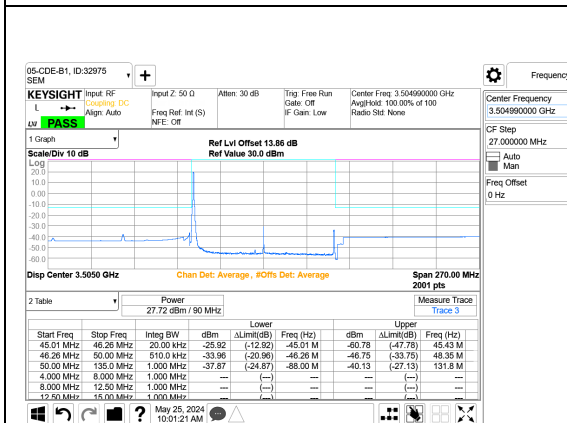
5G NR n77 90MHz BPSK High Channel RB1-0 Port A+B
