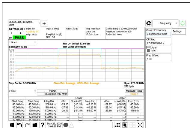
5G NR n77 90MHz BPSK High Channel RB243-0 Port A
