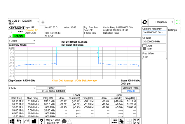
5G NR n77 100MHz BPSK Middle Channel RB270-0 Port A+B
