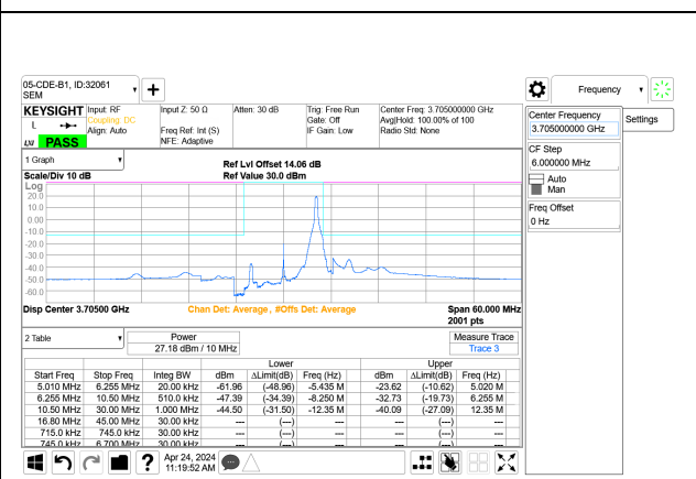
5G NR n77 10MHz BPSK Low Channel RB1-23 Port A+B ID 27342
