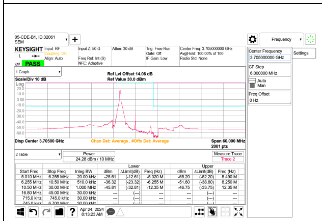
5G NR n77 10MHz BPSK Low Channel RB1-0 Port B ID 27342
