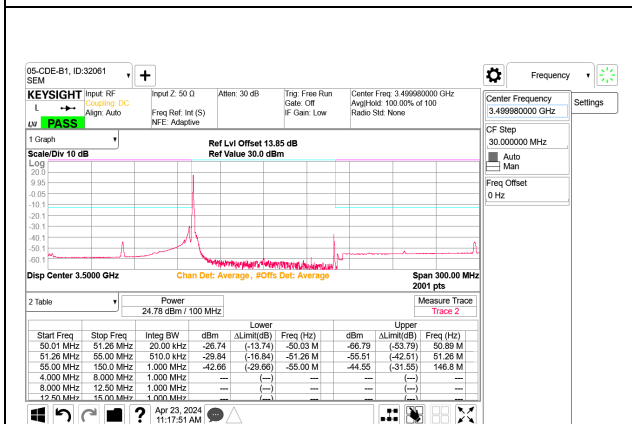
5G NR n77 100MHz BPSK Middle Channel RB1-0 Port B
