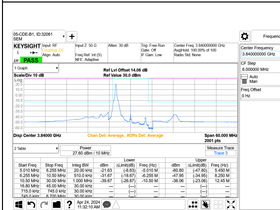
5G NR n77 10MHz BPSK Middle Channel RB1-0 Port A+B
