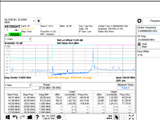
5G NR n77 80MHz BPSK Mid Channel RB1-216 Port A+B
