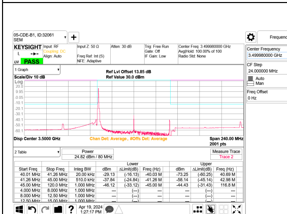
5G NR n77 80MHz BPSK Middle Channel RB1-0 Port B
