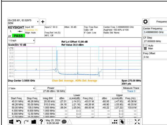
5G NR n77 90MHz BPSK Middle Channel RB1-0 Port A+B
