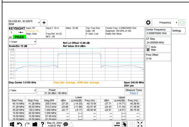
5G NR n77 80MHz BPSK High Channel RB216-0 Port A+B
