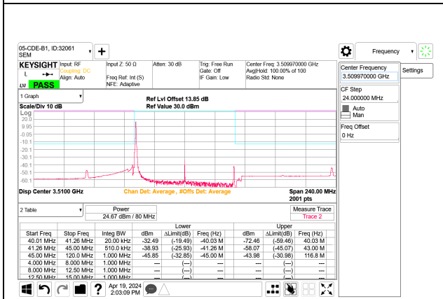
5G NR n77 80MHz BPSK High Channel RB1-0 Port B
