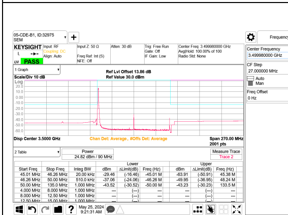
5G NR n77 90MHz BPSK Middle Channel RB1-0 Port B
