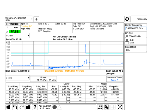
5G NR n77 90MHz BPSK Mid Channel RB1-244 Port A+B
