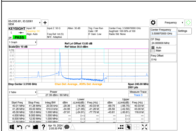
5G NR n77 80MHz BPSK High Channel RB1-0 Port A+B
