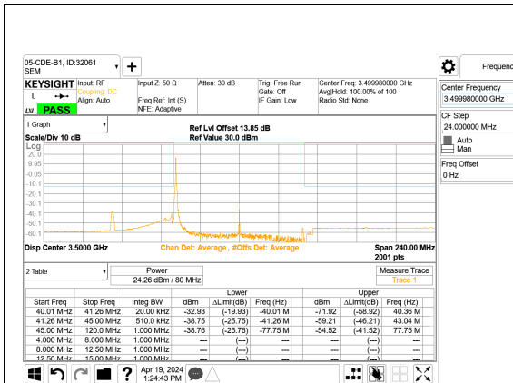
5G NR n77 80MHz BPSK Middle Channel RB1-0 Port A
