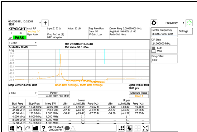
5G NR n77 80MHz BPSK High Channel RB1-0 Port A
