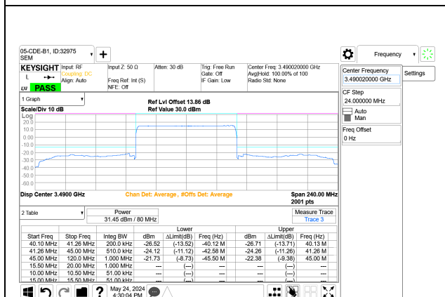
5G NR n77 80MHz BPSK Low Channel RB216-0 Port A+B
