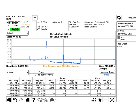
5G NR n77 80MHz BPSK Middle Channel RB1-0 Port A+B
