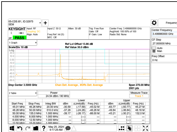
5G NR n77 90MHz BPSK Middle Channel RB1-0 Port A
