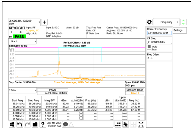
5G NR n77 70MHz BPSK High Channel RB1-0 Port A
