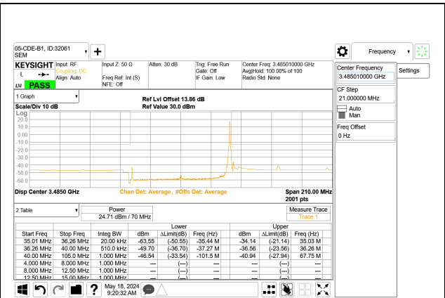
5G NR n77 70MHz BPSK Low Channel RB1-188 Port A
