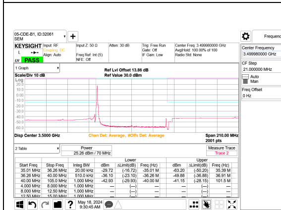
5G NR n77 70MHz BPSK Middle Channel RB1-0 Port B
