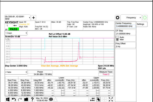
5G NR n77 70MHz BPSK Mid Channel RB1-188 Port B
