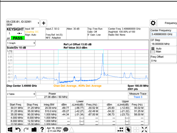
5G NR n77 60MHz BPSK Mid Channel RB1-161 Port A+B
