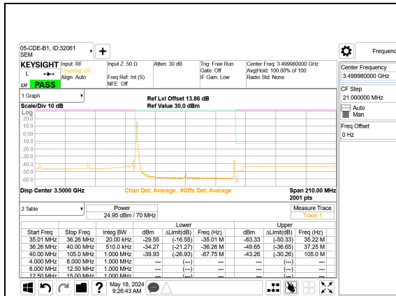
5G NR n77 70MHz BPSK Middle Channel RB1-0 Port A
