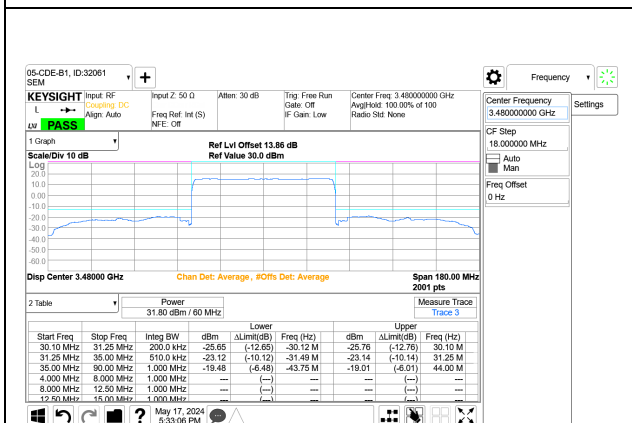
5G NR n77 60MHz BPSK Low Channel RB162-0 Port A+B
