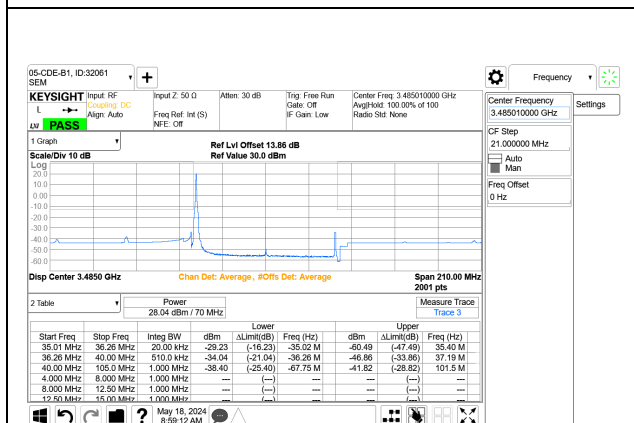
5G NR n77 70MHz BPSK Low Channel RB1-0 Port A+B
