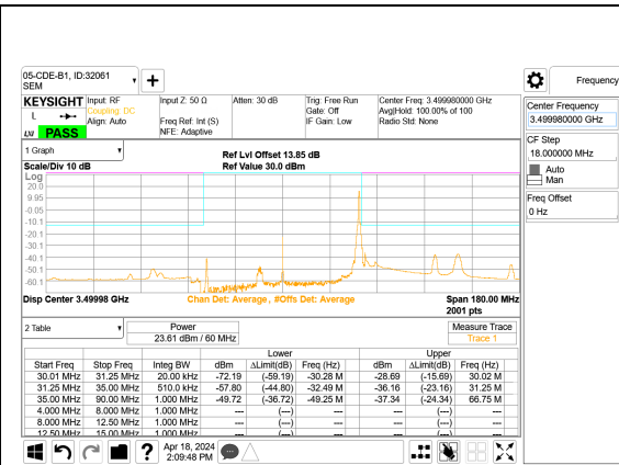
5G NR n77 60MHz BPSK Mid Channel RB1-161 Port A
