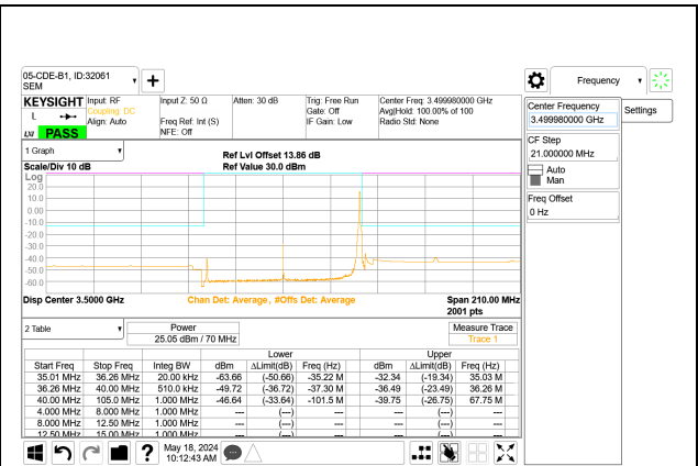
5G NR n77 70MHz BPSK Mid Channel RB1-188 Port A
