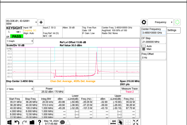
5G NR n77 70MHz BPSK Low Channel RB1-188 Port B
