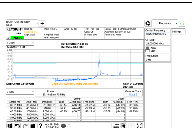
5G NR n77 70MHz BPSK High Channel RB1-188 Port A+B
