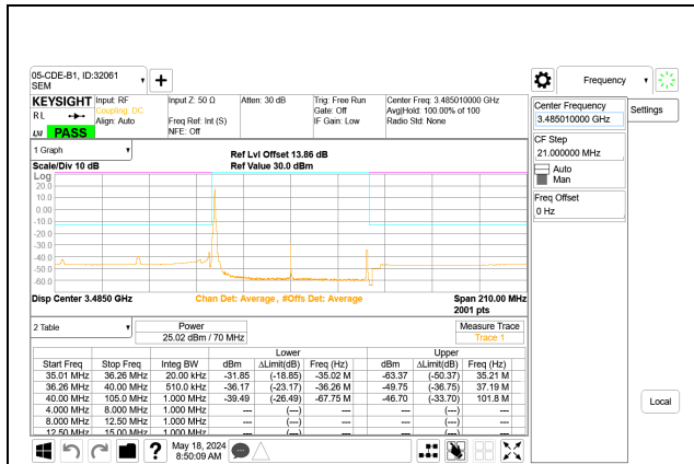
5G NR n77 70MHz BPSK Low Channel RB1-0 Port A
