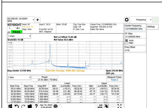
5G NR n77 70MHz BPSK High Channel RB1-0 Port A+B
