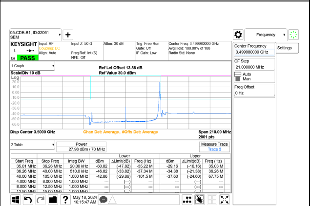
5G NR n77 70MHz BPSK Mid Channel RB1-188 Port A+B
