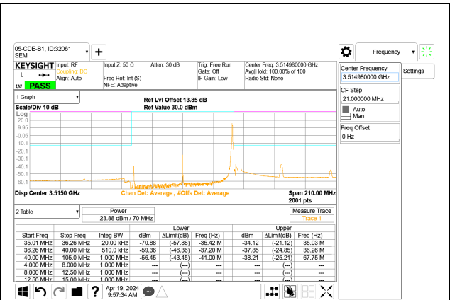
5G NR n77 70MHz BPSK High Channel RB1-188 Port A
