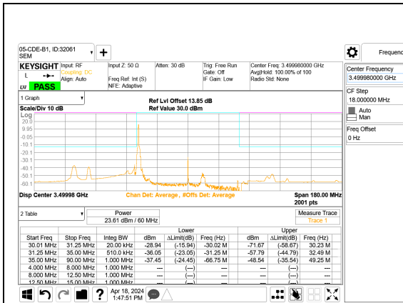
5G NR n77 60MHz BPSK Middle Channel RB1-0 Port A
