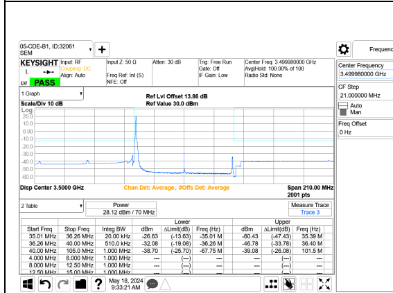
5G NR n77 70MHz BPSK Middle Channel RB1-0 Port A+B
