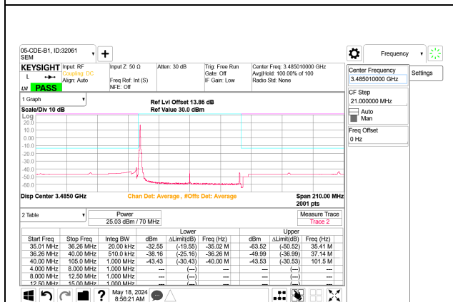
5G NR n77 70MHz BPSK Low Channel RB1-0 Port B
