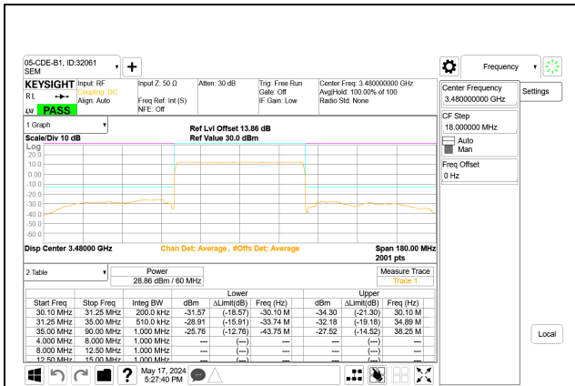
5G NR n77 60MHz BPSK Low Channel RB162-0 Port A
