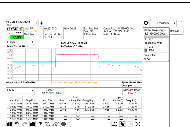
5G NR n77 60MHz BPSK High Channel RB162-0 Port B
