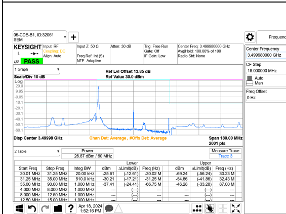
5G NR n77 60MHz BPSK Middle Channel RB1-0 Port A+B
