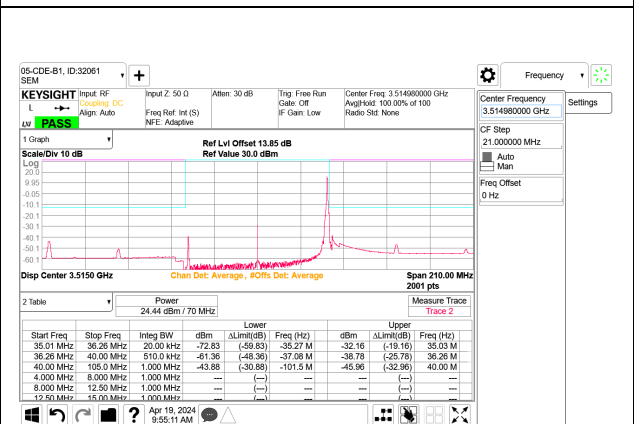
5G NR n77 70MHz BPSK High Channel RB1-188 Port B
