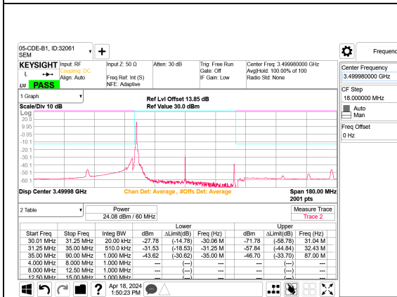
5G NR n77 60MHz BPSK Middle Channel RB1-0 Port B
