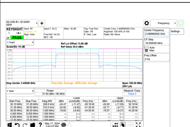
5G NR n77 60MHz BPSK Mid Channel RB162-0 Port A+B
