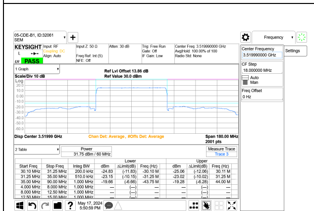
5G NR n77 60MHz BPSK High Channel RB162-0 Port A+B
