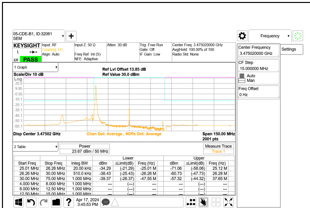
5G NR n77 50MHz BPSK Low Channel RB1-0 Port A
