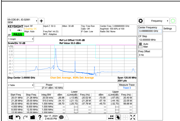
5G NR n77 40MHz BPSK Middle Channel RB1-0 Port A+B
