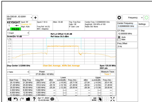
5G NR n77 40MHz BPSK High Channel RB100-0 Port A
