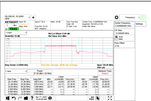
5G NR n77 40MHz BPSK High Channel RB100-0 Port B
