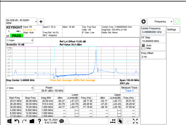
5G NR n77 50MHz BPSK Mid Channel RB1-132 Port A+B
