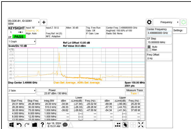
5G NR n77 50MHz BPSK Middle Channel RB1-0 Port A
