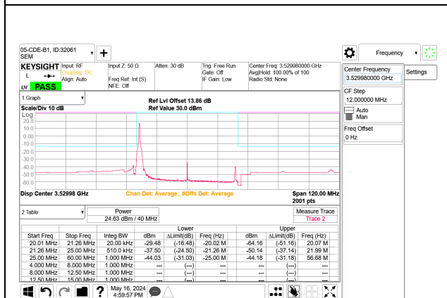
5G NR n77 40MHz BPSK High Channel RB1-0 Port B
