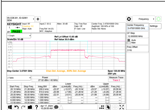
5G NR n77 40MHz BPSK Low Channel RB100-0 Port B
