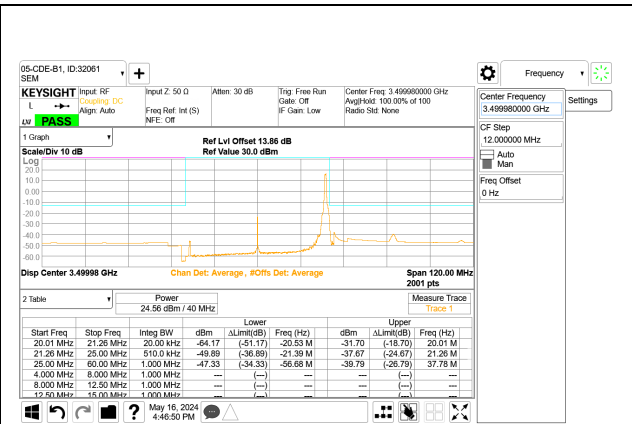
5G NR n77 40MHz BPSK Mid Channel RB1-105 Port A
