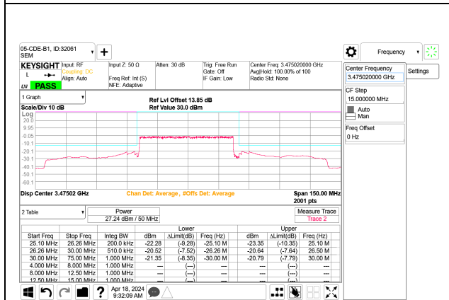
5G NR n77 50MHz BPSK Low Channel RB128-0 Port B
