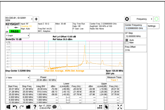
5G NR n77 40MHz BPSK High Channel RB1-105 Port A
