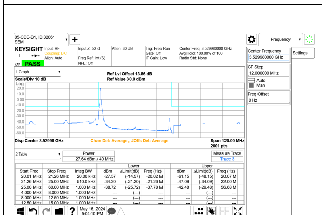
5G NR n77 40MHz BPSK High Channel RB1-0 Port A+B
