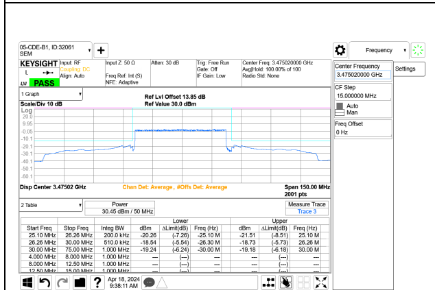
5G NR n77 50MHz BPSK Low Channel RB128-0 Port A+B
