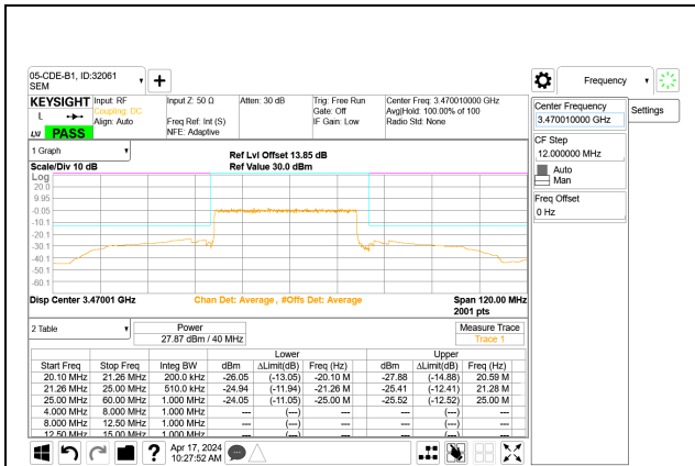
5G NR n77 40MHz BPSK Low Channel RB100-0 Port A
