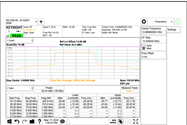
5G NR n77 50MHz BPSK Mid Channel RB128-0 Port A
