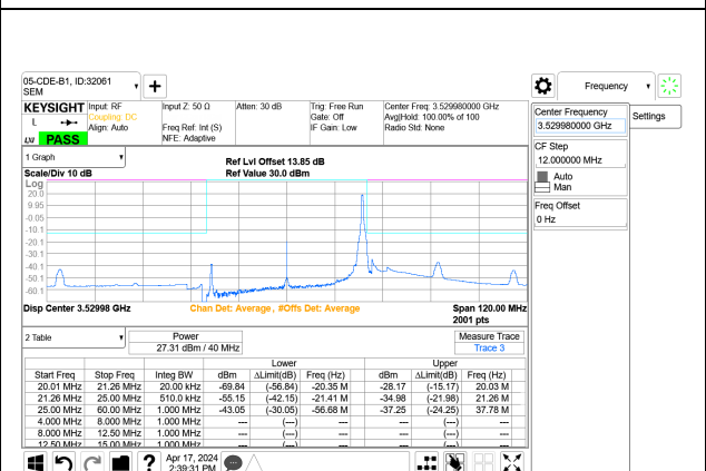
5G NR n77 40MHz BPSK High Channel RB1-105 Port A+B
