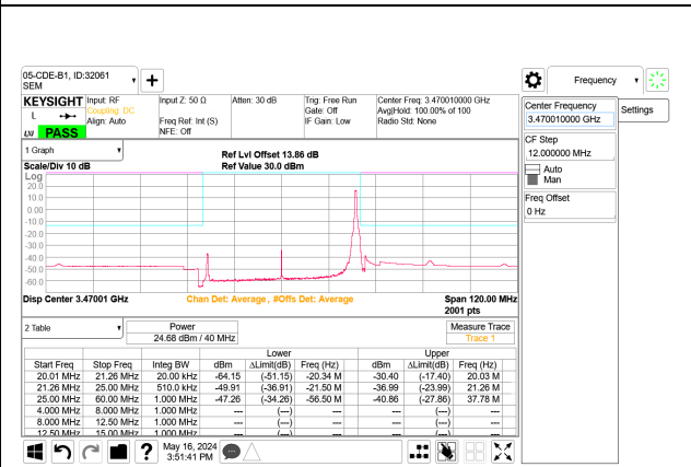
5G NR n77 40MHz BPSK Low Channel RB1-105 Port B
