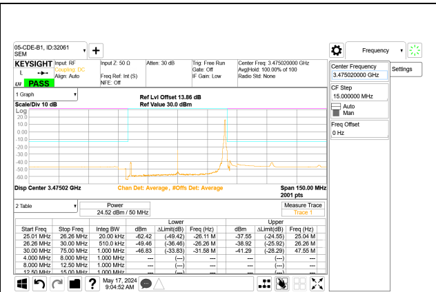
5G NR n77 50MHz BPSK Low Channel RB1-132 Port A
