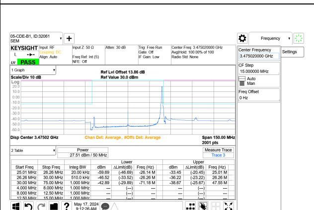
5G NR n77 50MHz BPSK Low Channel RB1-132 Port A+B
