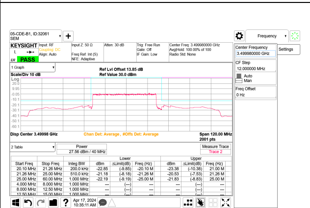
5G NR n77 40MHz BPSK Mid Channel RB100-0 Port B
