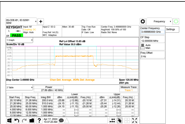
5G NR n77 40MHz BPSK Mid Channel RB100-0 Port A
