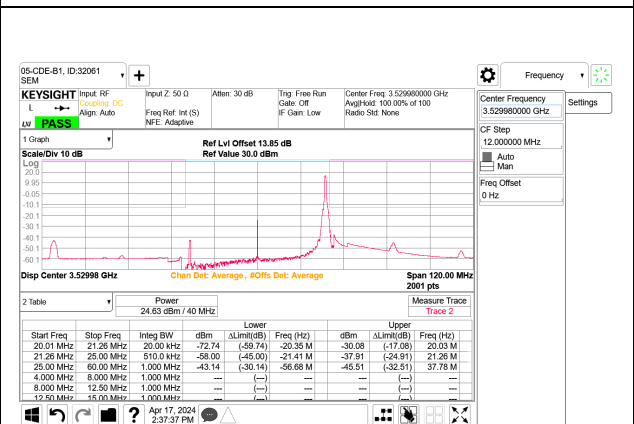
5G NR n77 40MHz BPSK High Channel RB1-105 Port B
