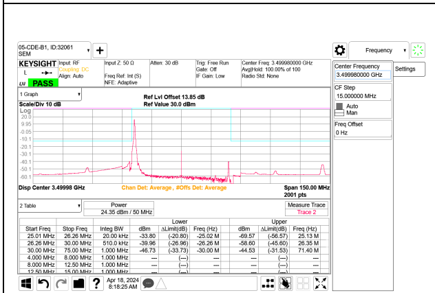
5G NR n77 50MHz BPSK Middle Channel RB1-0 Port B
