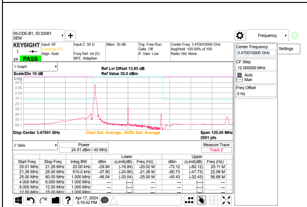
5G NR n77 40MHz BPSK Low Channel RB1-0 Port B
