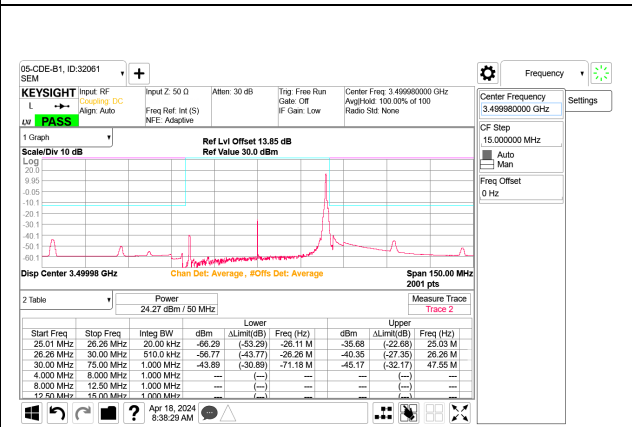
5G NR n77 50MHz BPSK Mid Channel RB1-132 Port B
