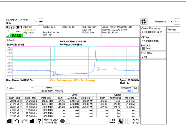
5G NR n77 40MHz BPSK Mid Channel RB1-105 Port A+B
