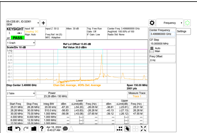
5G NR n77 50MHz BPSK Mid Channel RB1-132 Port A
