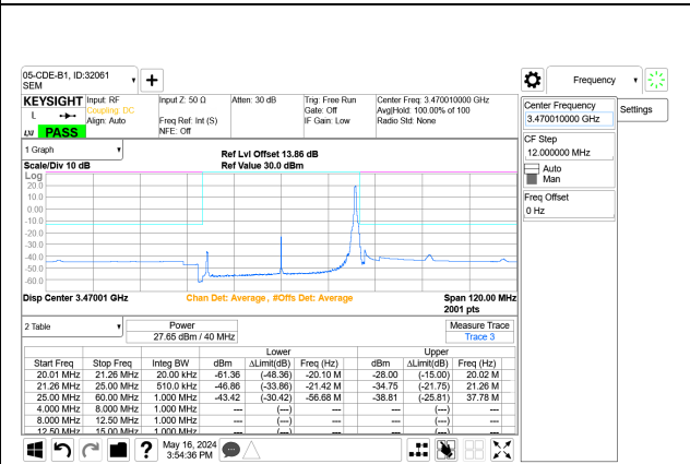
5G NR n77 40MHz BPSK Low Channel RB1-105 Port A+B
