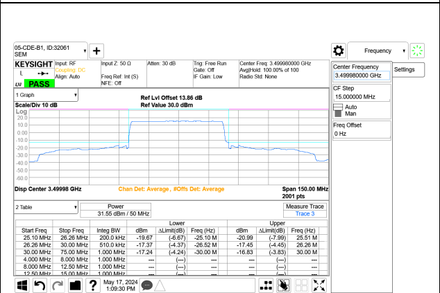
5G NR n77 50MHz BPSK Mid Channel RB128-0 Port A+B
