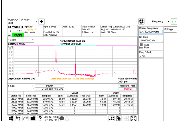
5G NR n77 50MHz BPSK Low Channel RB1-0 Port B
