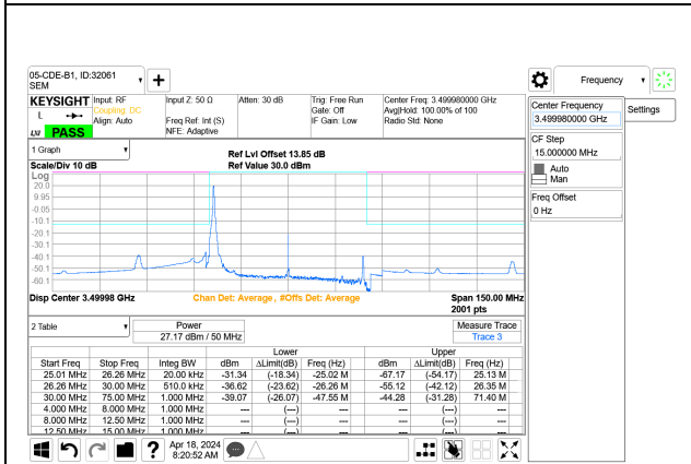
5G NR n77 50MHz BPSK Middle Channel RB1-0 Port A+B
