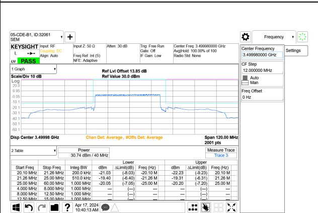
5G NR n77 40MHz BPSK Mid Channel RB100-0 Port A+B
