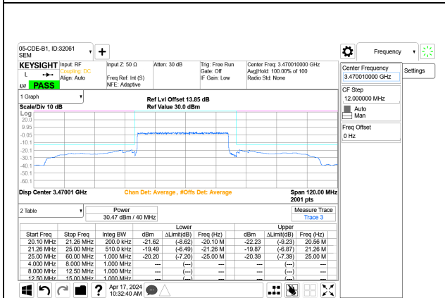
5G NR n77 40MHz BPSK Low Channel RB100-0 Port A+B
