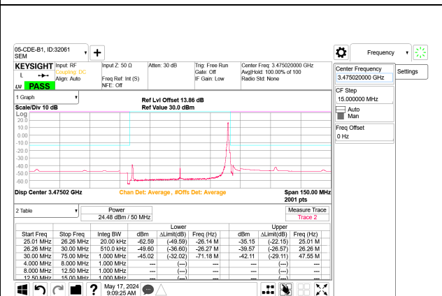
5G NR n77 50MHz BPSK Low Channel RB1-132 Port B
