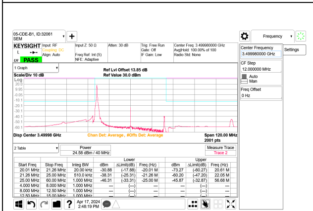
5G NR n77 40MHz BPSK Middle Channel RB1-0 Port B
