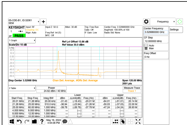
5G NR n77 40MHz BPSK High Channel RB1-0 Port A
