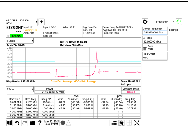
5G NR n77 40MHz BPSK Mid Channel RB1-105 Port B
