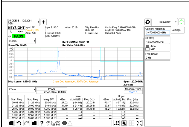
5G NR n77 40MHz BPSK Low Channel RB1-0 Port A+B
