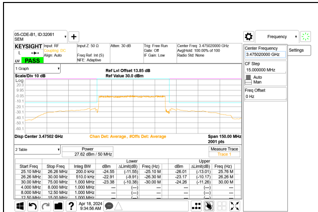
5G NR n77 50MHz BPSK Low Channel RB128-0 Port A
