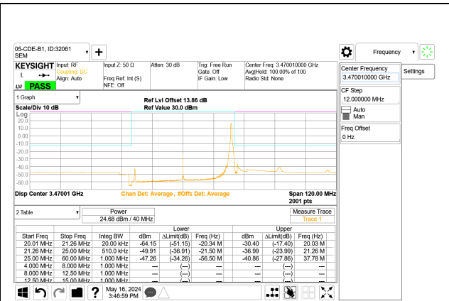
5G NR n77 40MHz BPSK Low Channel RB1-105 Port A
