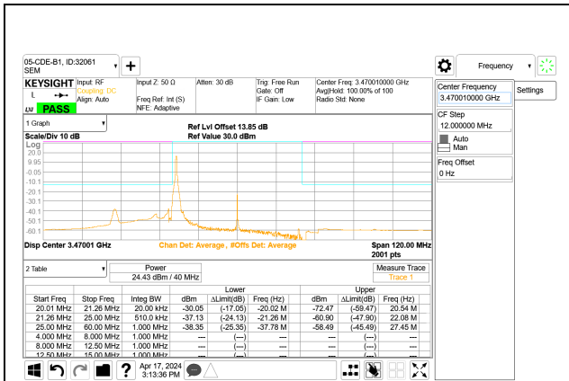
5G NR n77 40MHz BPSK Low Channel RB1-0 Port A
