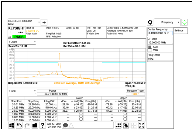
5G NR n77 40MHz BPSK Middle Channel RB1-0 Port A
