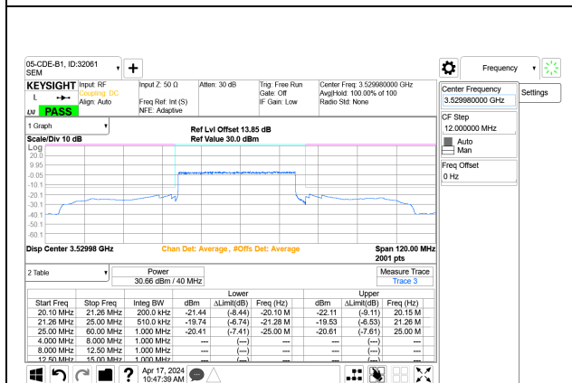
5G NR n77 40MHz BPSK High Channel RB100-0 Port A+B
