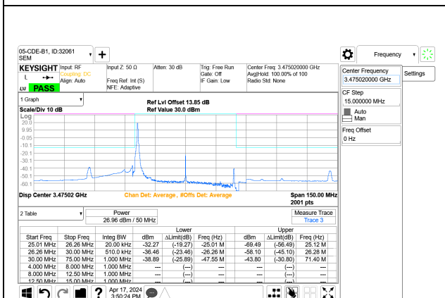
5G NR n77 50MHz BPSK Low Channel RB1-0 Port A+B
