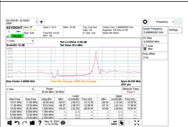
5G NR n77 20MHz BPSK Mid Channel RB1-50 Port B
