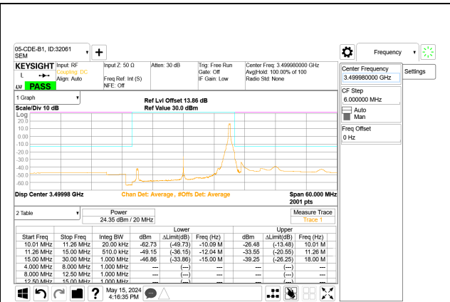
5G NR n77 20MHz BPSK Mid Channel RB1-50 Port A
