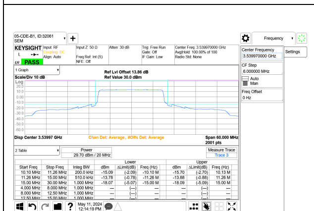
5G NR n77 20MHz BPSK High Channel RB50-0 Port A+B
