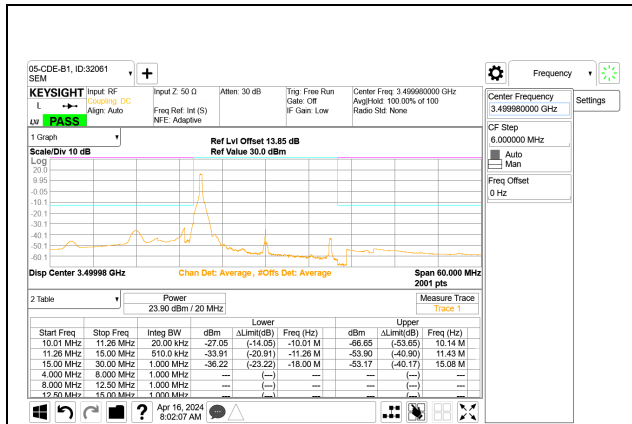
5G NR n77 20MHz BPSK Middle Channel RB1-0 Port A
