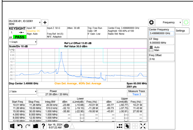
5G NR n77 20MHz BPSK Middle Channel RB1-0 Port A+B
