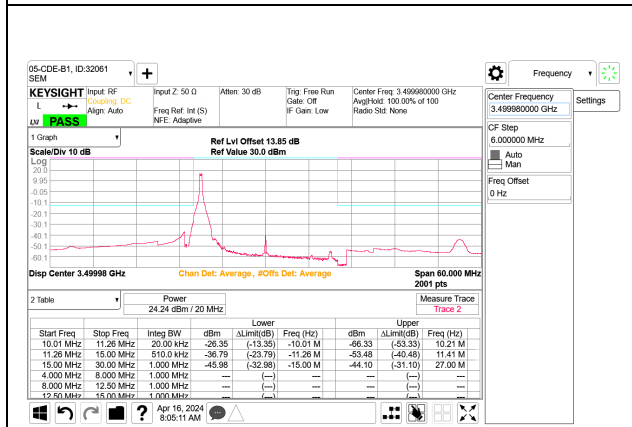
5G NR n77 20MHz BPSK Middle Channel RB1-0 Port B
