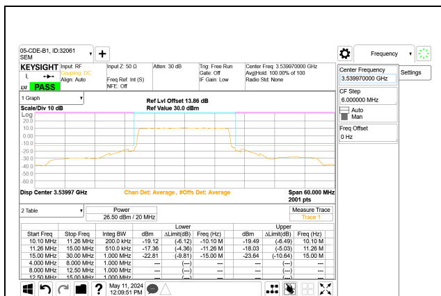
5G NR n77 20MHz BPSK High Channel RB50-0 Port A
