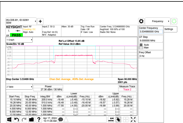
5G NR n77 30MHz BPSK High Channel RB75-0 Port B
