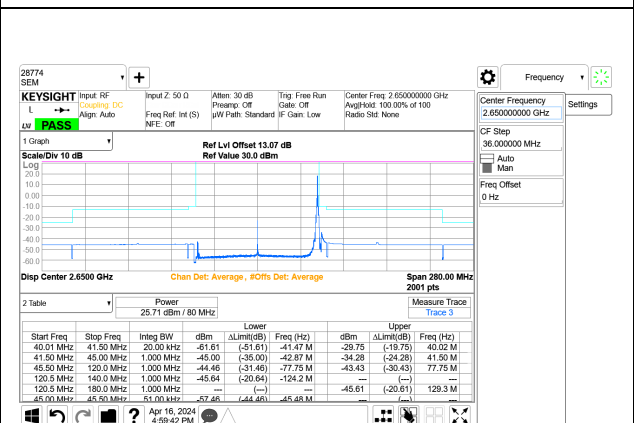
5G NR n41 80MHz BPSK High Channel RB1-216 Port A+B
