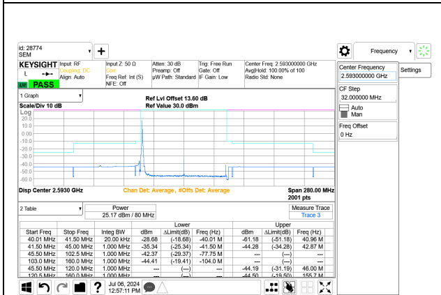
5G NR n41 80MHz BPSK Middle Channel RB1-0 Port A+B
