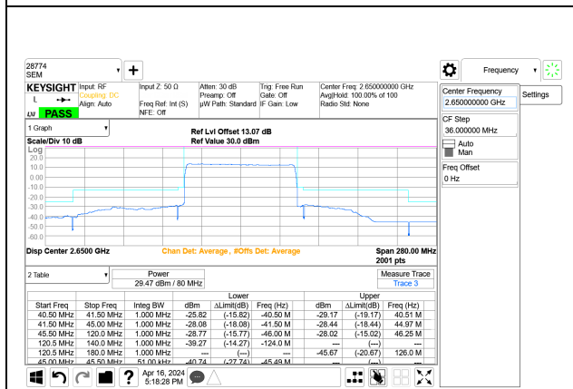
5G NR n41 80MHz BPSK High Channel RB216-0 Port A+B
