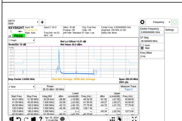
5G NR n41 80MHz BPSK High Channel RB1-0 Port A+B
