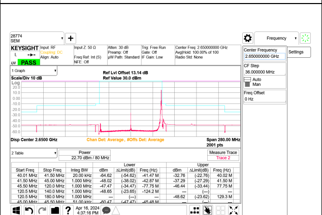
5G NR n41 80MHz BPSK High Channel RB1-216 Port B
