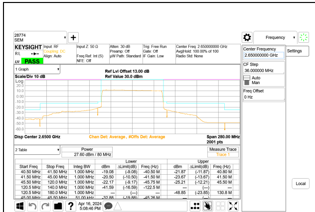
5G NR n41 80MHz BPSK High Channel RB216-0 Port A
