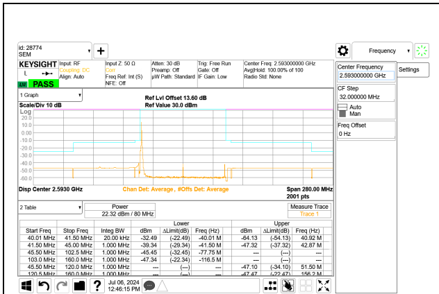
5G NR n41 80MHz BPSK Middle Channel RB1-0 Port A
