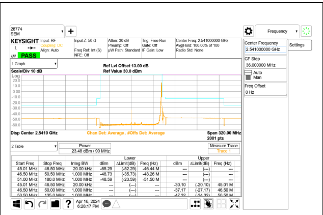
5G NR n41 90MHz BPSK Low Channel RB1-244 Port A ID: 32546
