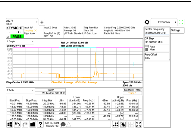
5G NR n41 80MHz BPSK High Channel RB1-216 Port A
