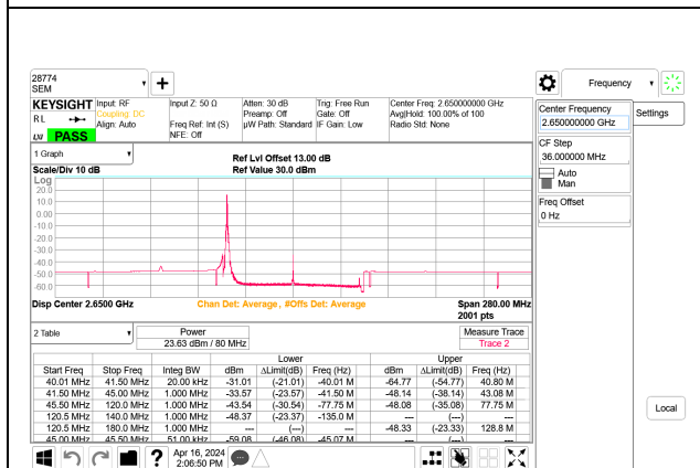
5G NR n41 80MHz BPSK High Channel RB1-0 Port B
