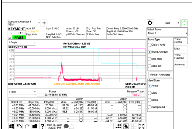
5G NR n41 80MHz BPSK Low Channel RB1-0 Port B ID: 32546
