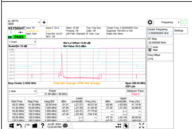
5G NR n41 80MHz BPSK Middle Channel RB1-0 Port B
