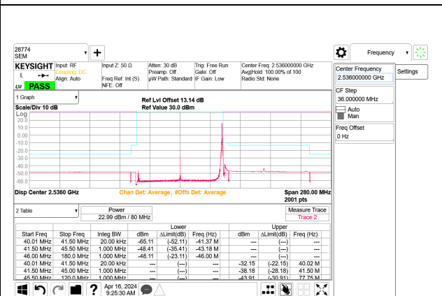
5G NR n41 80MHz BPSK Low Channel RB1-216 Port B
