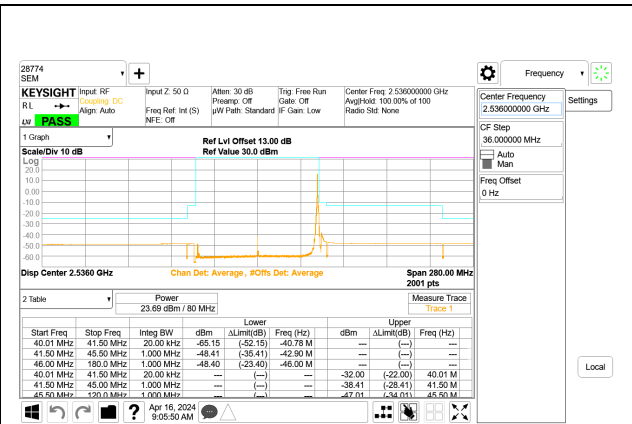
5G NR n41 80MHz BPSK Low Channel RB1-216 Port A
