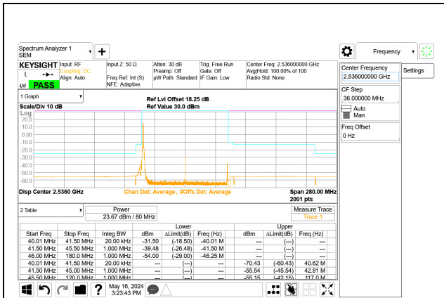
5G NR n41 80MHz BPSK Low Channel RB1-0 Port A ID: 32546
