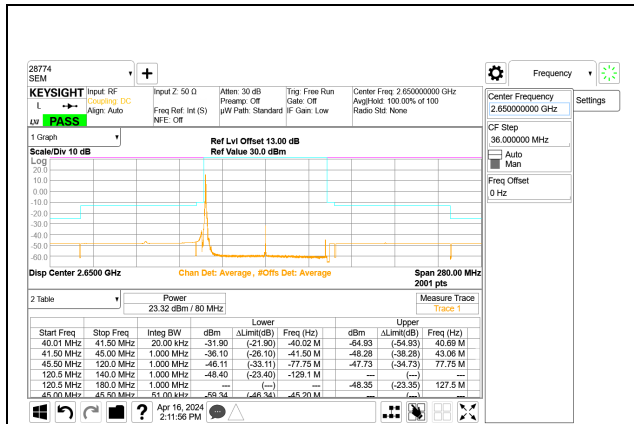
5G NR n41 80MHz BPSK High Channel RB1-0 Port A
