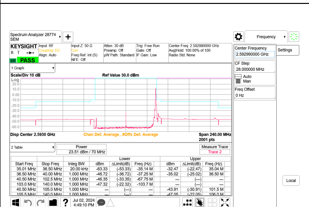
5G NR n41 70MHz BPSK Mid Channel RB1-188 Port B
