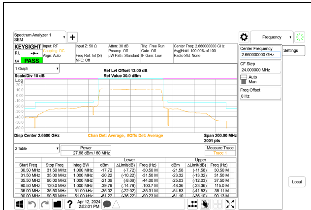
5G NR n41 60MHz BPSK High Channel RB162-0 Port A ID: 32546
