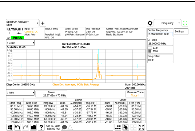
5G NR n41 70MHz BPSK High Channel RB1-188 Port A ID: 32546
