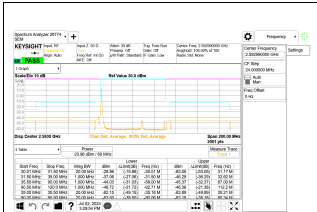
5G NR n41 60MHz BPSK Middle Channel RB1-0 Port A
