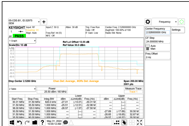
5G NR n41 60MHz BPSK Low Channel RB162-0 Port A
