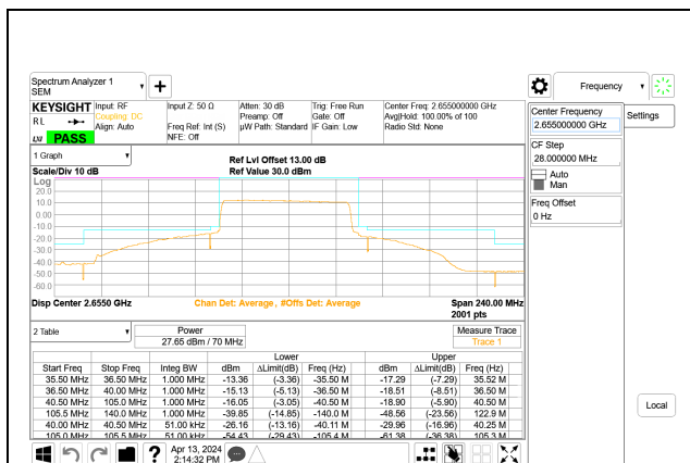
5G NR n41 70MHz BPSK High Channel RB180-0 Port A ID: 32546
