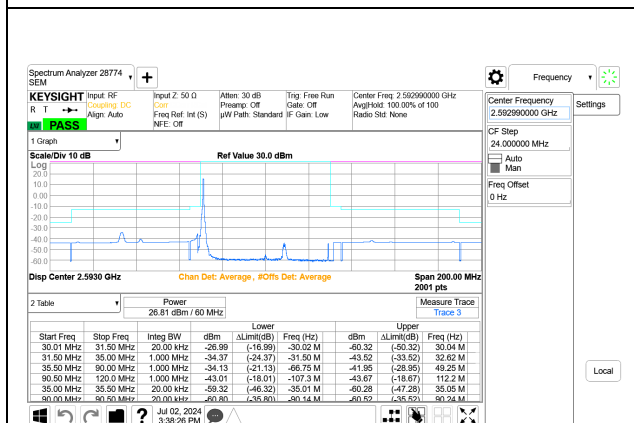
5G NR n41 60MHz BPSK Middle Channel RB1-0 Port A+B
