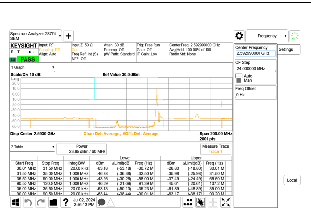
5G NR n41 60MHz BPSK Mid Channel RB1-161 Port A
