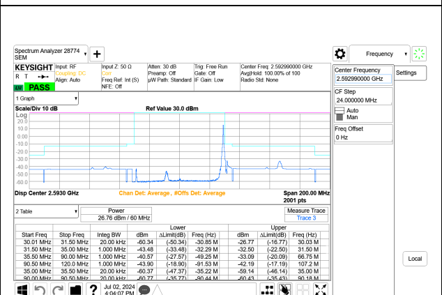
5G NR n41 60MHz BPSK Mid Channel RB1-161 Port A+B
