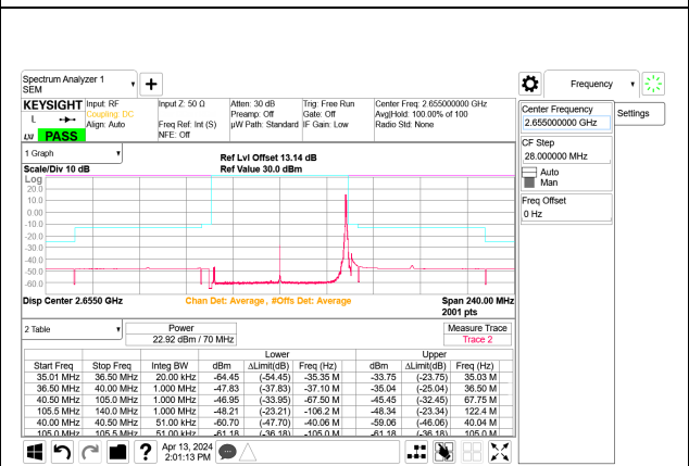
5G NR n41 70MHz BPSK High Channel RB1-188 Port B ID: 32546
