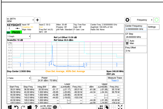
5G NR n41 70MHz BPSK Middle Channel RB1-0 Port A+B
