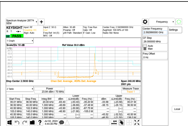
5G NR n41 70MHz BPSK Mid Channel RB1-188 Port A
