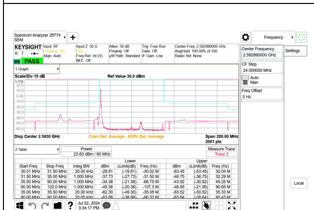
5G NR n41 60MHz BPSK Middle Channel RB1-0 Port B
