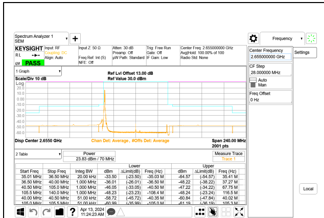
5G NR n41 70MHz BPSK High Channel RB1-0 Port A ID: 32546
