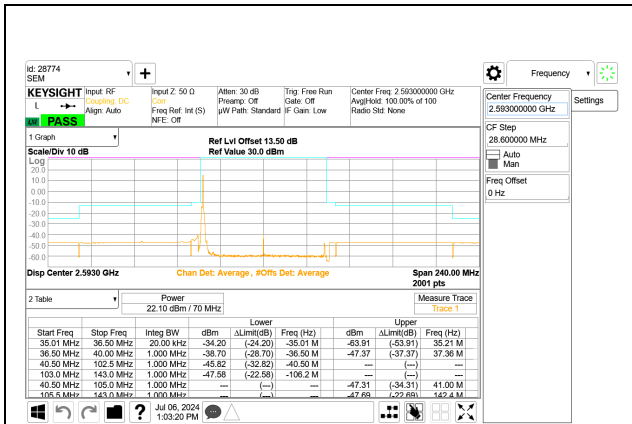
5G NR n41 70MHz BPSK Middle Channel RB1-0 Port A
