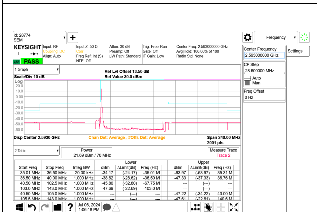
5G NR n41 70MHz BPSK Middle Channel RB1-0 Port B
