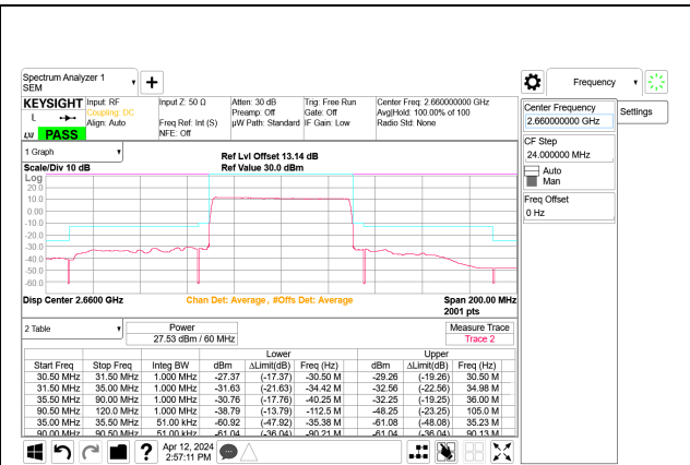
5G NR n41 60MHz BPSK High Channel RB162-0 Port B ID: 32546
