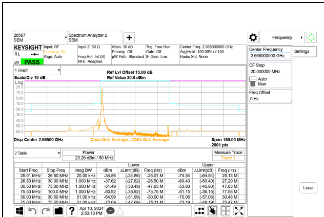
5G NR n41 50MHz BPSK High Channel RB1-0 Port A
