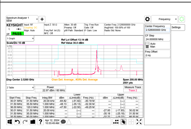
5G NR n41 60MHz BPSK Low Channel RB1-161 Port B ID: 32546
