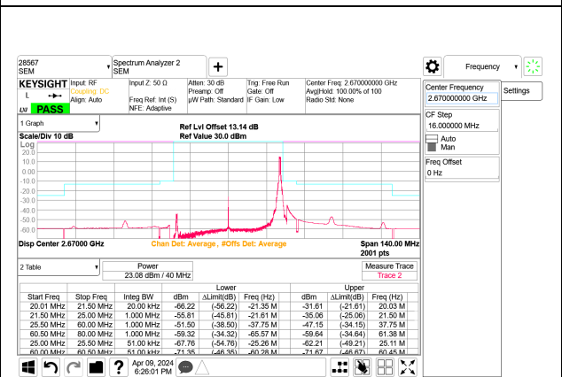
5G NR n41 40MHz BPSK High Channel RB1-105 Port B
