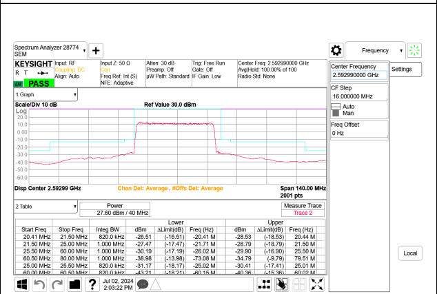
5G NR n41 40MHz BPSK Mid Channel RB100-0 Port B
