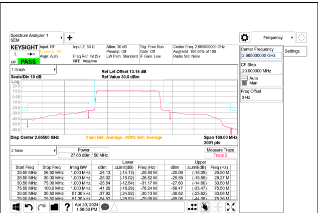
5G NR n41 50MHz BPSK High Channel RB128-0 Port B ID: 32546
