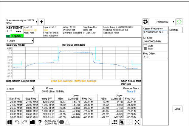
5G NR n41 40MHz BPSK Mid Channel RB100-0 Port A+B
