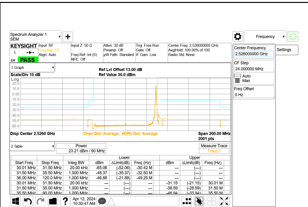
5G NR n41 60MHz BPSK Low Channel RB1-161 Port A ID: 32546
