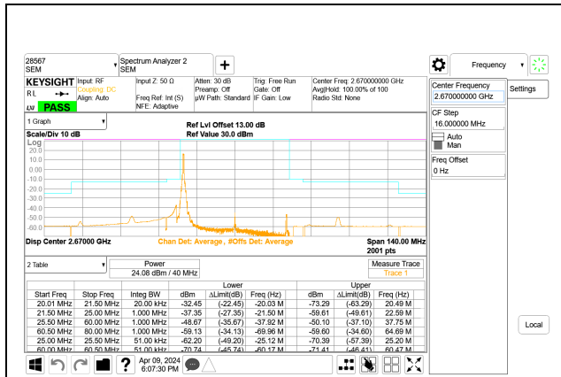
5G NR n41 40MHz BPSK High Channel RB1-0 Port A
