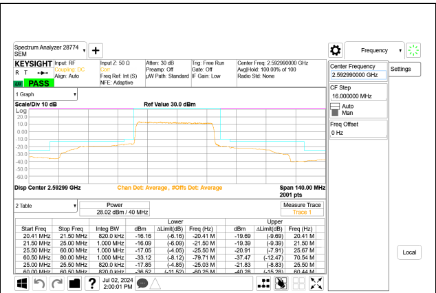
5G NR n41 40MHz BPSK Mid Channel RB100-0 Port A
