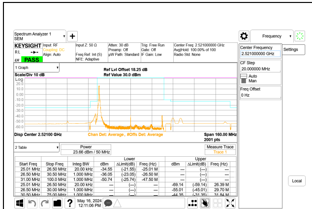
5G NR n41 50MHz BPSK Low Channel RB1-0 Port A ID: 32546
