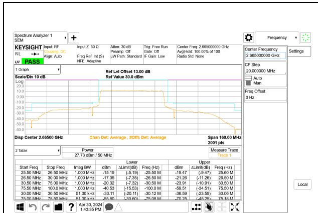
5G NR n41 50MHz BPSK High Channel RB128-0 Port A ID: 32546
