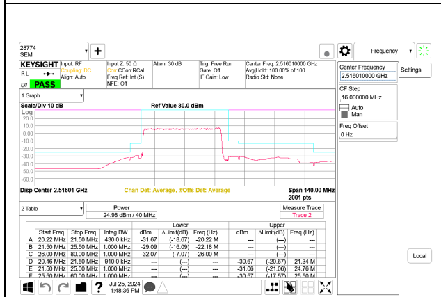
5G NR n41 40MHz BPSK Low Channel RB100-0 Port B
