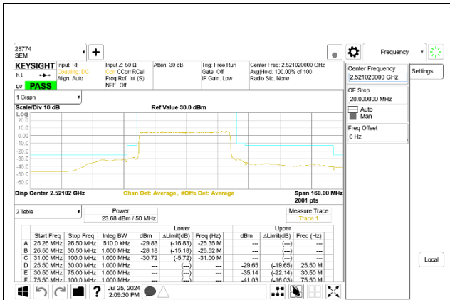
5G NR n41 50MHz BPSK Low Channel RB128-0 Port A
