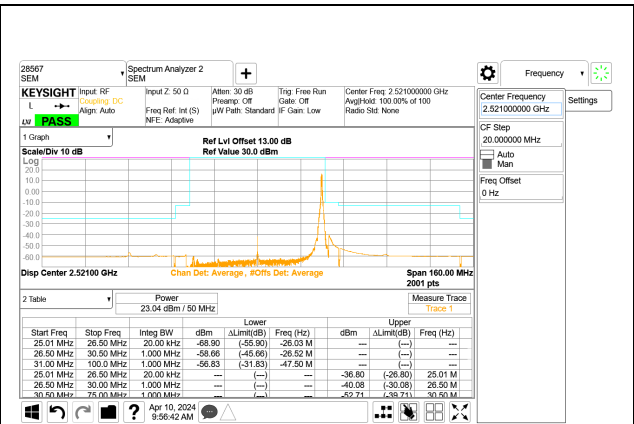
5G NR n41 50MHz BPSK Low Channel RB1-132 Port A
