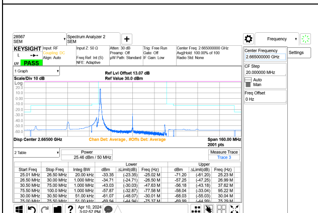
5G NR n41 50MHz BPSK High Channel RB1-0 Port A+B
