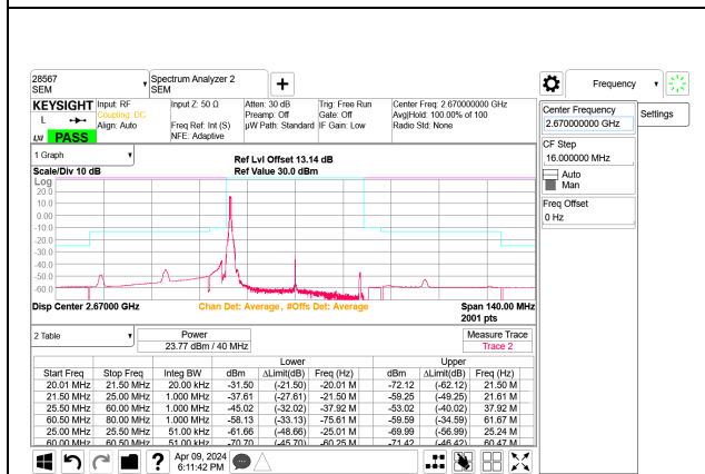
5G NR n41 40MHz BPSK High Channel RB1-0 Port B
