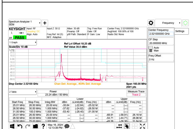
5G NR n41 50MHz BPSK Low Channel RB1-0 Port B ID: 32546
