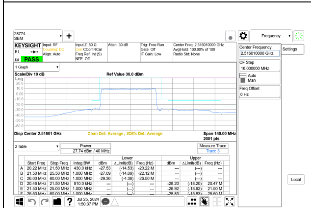
5G NR n41 40MHz BPSK Low Channel RB100-0 Port A+B
