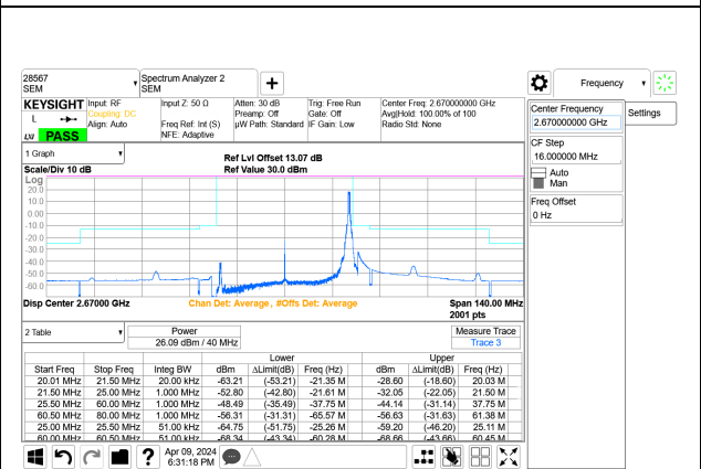
5G NR n41 40MHz BPSK High Channel RB1-105 Port A+B
