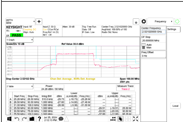
5G NR n41 50MHz BPSK Low Channel RB128-0 Port B
