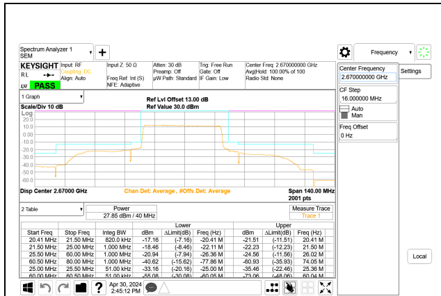
5G NR n41 40MHz BPSK High Channel RB100-0 Port A ID: 32546
