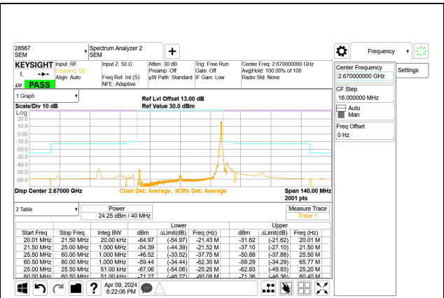
5G NR n41 40MHz BPSK High Channel RB1-105 Port A
