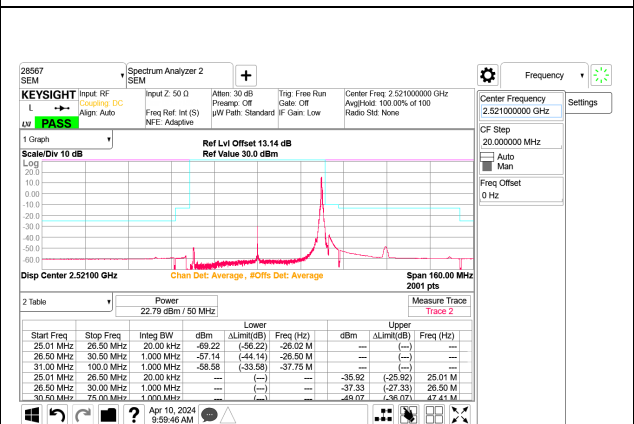
5G NR n41 50MHz BPSK Low Channel RB1-132 Port B ID:
