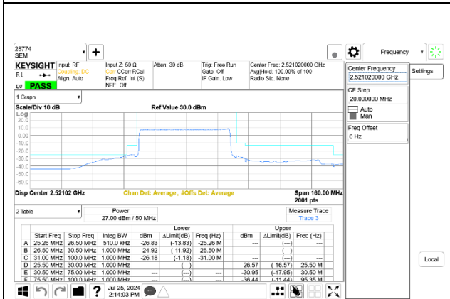
5G NR n41 50MHz BPSK Low Channel RB128-0 Port A+B
