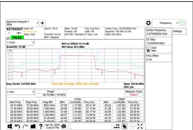
5G NR n41 40MHz BPSK High Channel RB100-0 Port B ID: 32546
