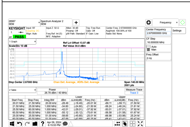
5G NR n41 40MHz BPSK High Channel RB1-0 Port A+B
