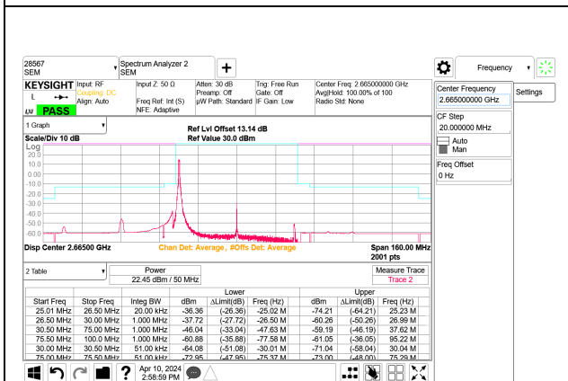
5G NR n41 50MHz BPSK High Channel RB1-0 Port B
