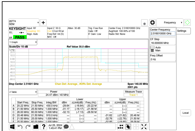
5G NR n41 40MHz BPSK Low Channel RB100-0 Port A
