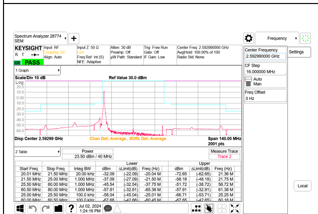
5G NR n41 40MHz BPSK Mid Channel RB1-0 Port B
