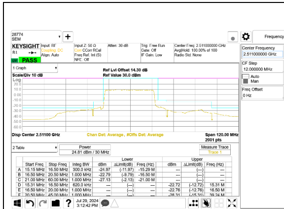
5G NR n41 30MHz BPSK Low Channel RB75-0 Port A
