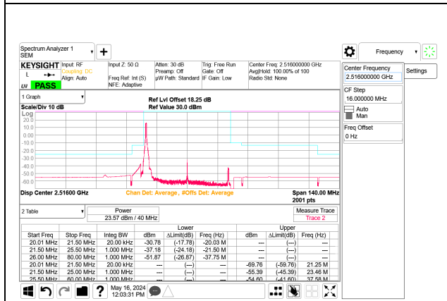
5G NR n41 40MHz BPSK Low Channel RB1-0 Port B ID: 32546
