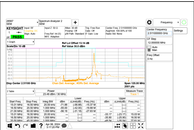
5G NR n41 30MHz BPSK Low Channel RB1-77 Port A
