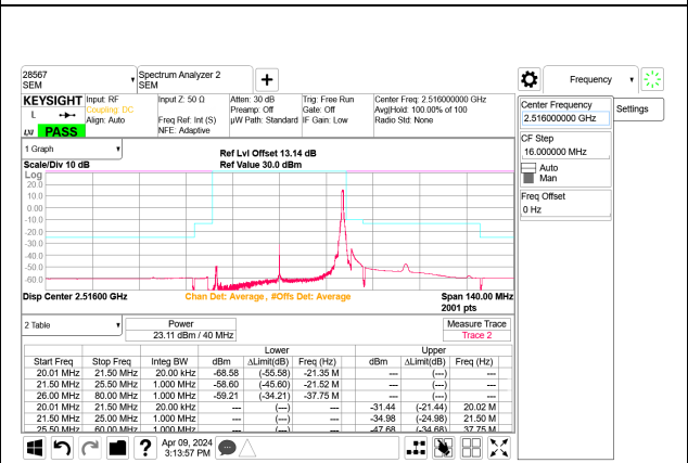
5G NR n41 40MHz BPSK Low Channel RB1-105 Port B
