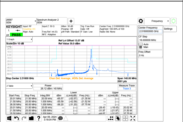
5G NR n41 40MHz BPSK Low Channel RB1-105 Port A+B
