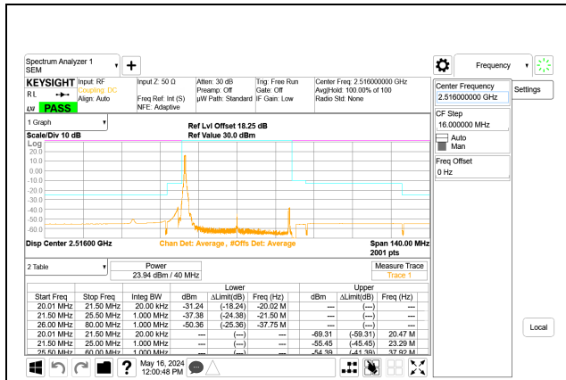
5G NR n41 40MHz BPSK Low Channel RB1-0 Port A ID: 32546
