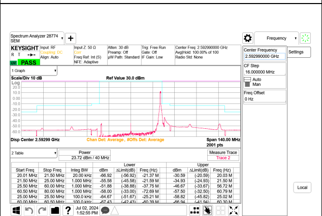
5G NR n41 40MHz BPSK Mid Channel RB1-105 Port B
