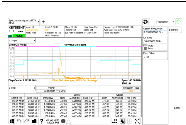
5G NR n41 40MHz BPSK Mid Channel RB1-0 Port A
