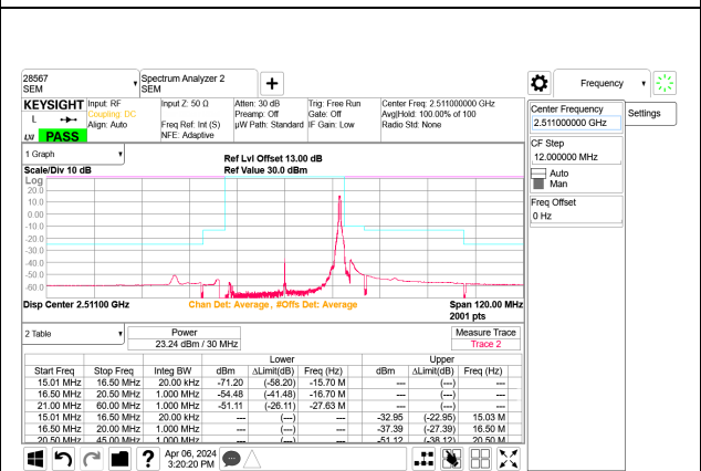
5G NR n41 30MHz BPSK Low Channel RB1-77 Port B
