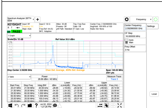
5G NR n41 40MHz BPSK Mid Channel RB1-0 Port A+B
