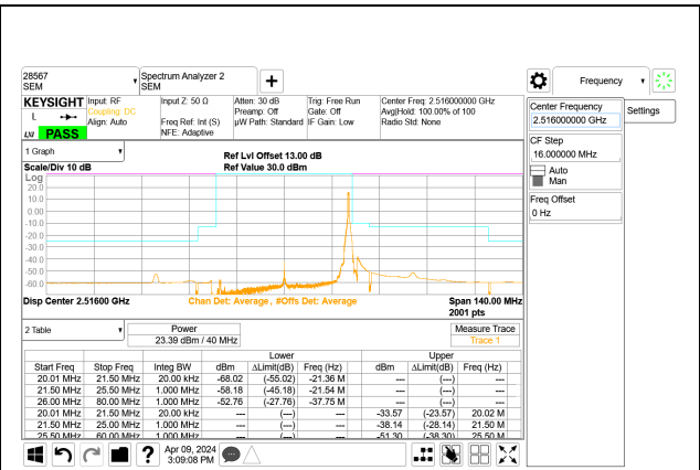
5G NR n41 40MHz BPSK Low Channel RB1-105 Port A
