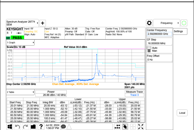
5G NR n41 40MHz BPSK Mid Channel RB1-105 Port A+B
