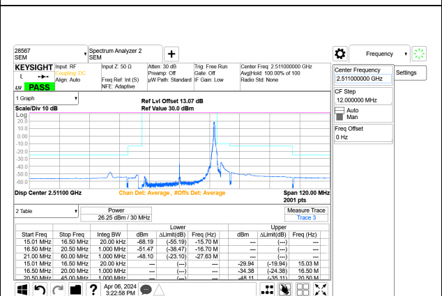
5G NR n41 30MHz BPSK Low Channel RB1-77 Port A+B
