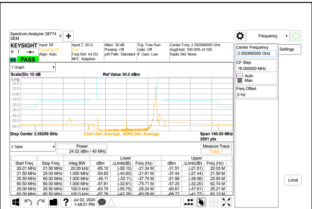
5G NR n41 40MHz BPSK Mid Channel RB1-105 Port A
