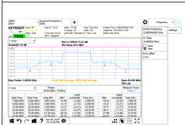
5G NR n41 15MHz BPSK High Channel RB36-0 Port A+B
