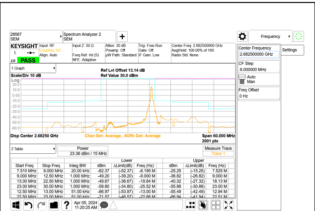
5G NR n41 15MHz BPSK High Channel RB1-37 Port A
