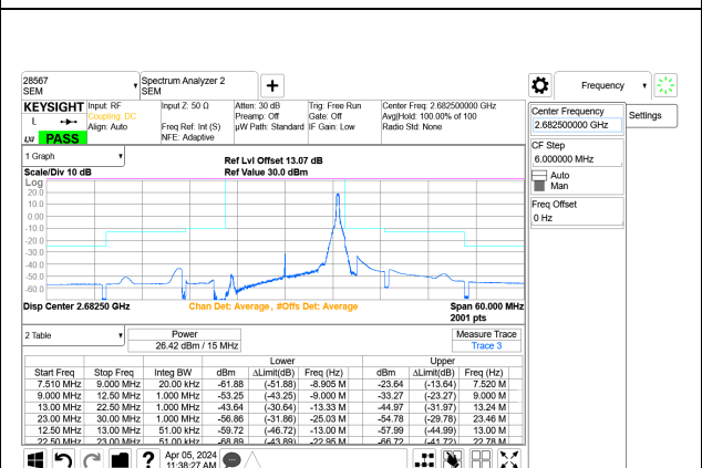
5G NR n41 15MHz BPSK High Channel RB1-37 Port A+B
