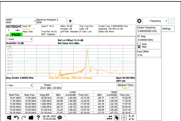
5G NR n41 20MHz BPSK High Channel RB1-50 Port A
