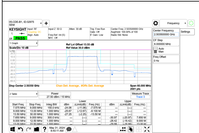
5G NR n41 15MHz BPSK Low Channel RB36-0 Port A+B
