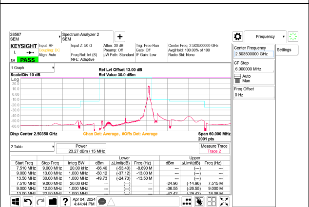
5G NR n41 15MHz BPSK Low Channel RB1-37 Port B
