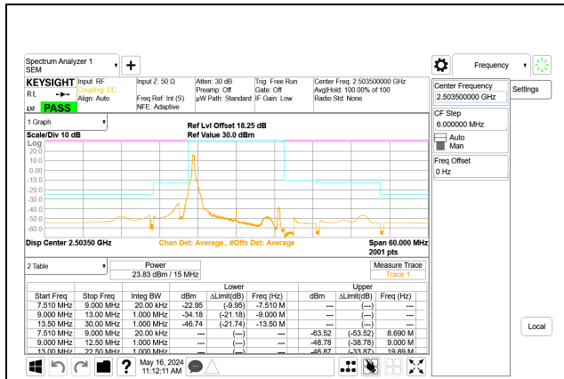
5G NR n41 15MHz BPSK Low Channel RB1-0 Port A ID: 32546
