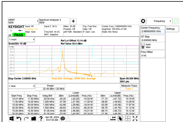
5G NR n41 20MHz BPSK High Channel RB1-0 Port A
