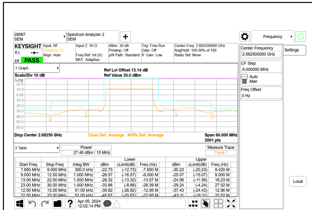
5G NR n41 15MHz BPSK High Channel RB36-0 Port A
