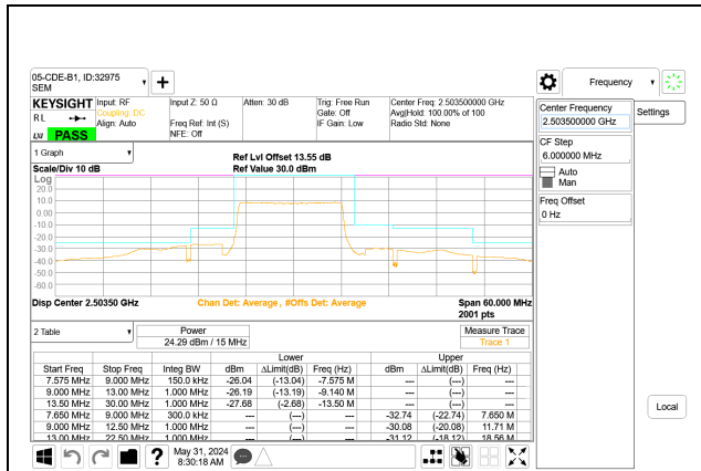
5G NR n41 15MHz BPSK Low Channel RB36-0 Port A
