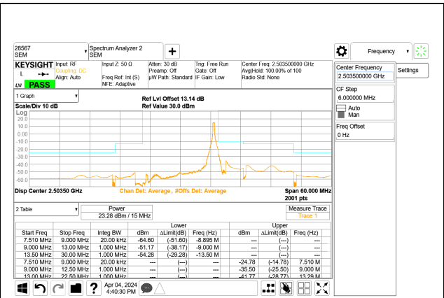
5G NR n41 15MHz BPSK Low Channel RB1-37 Port A
