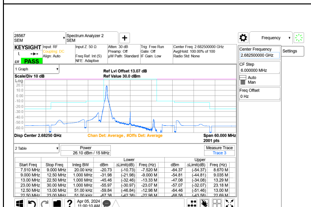
5G NR n41 15MHz BPSK High Channel RB1-0 Port A+B
