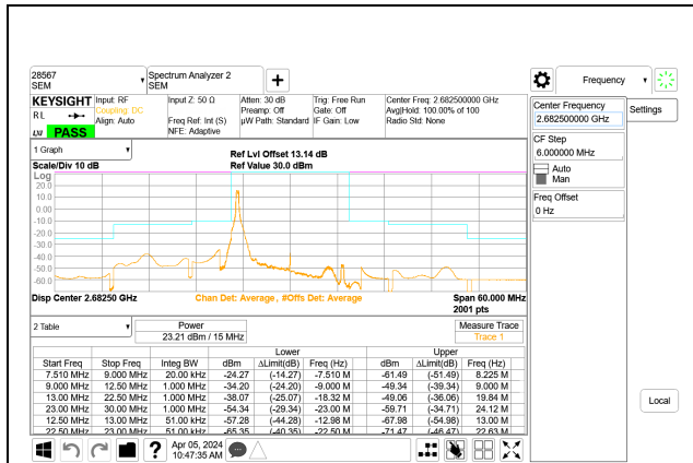
5G NR n41 15MHz BPSK High Channel RB1-0 Port A
