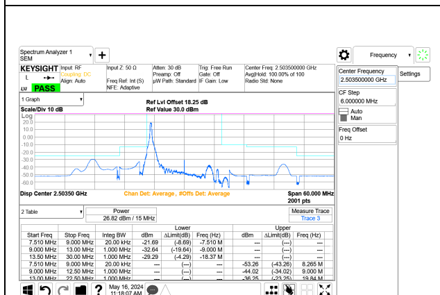
5G NR n41 15MHz BPSK Low Channel RB1-0 Port A+B ID: 32546
