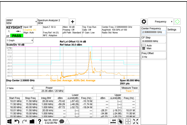
5G NR n41 20MHz BPSK Low Channel RB1-50 Port A
