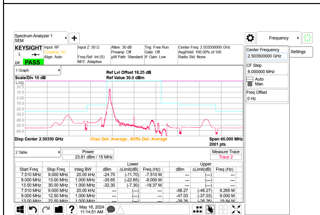
5G NR n41 15MHz BPSK Low Channel RB1-0 Port B ID: 32546
