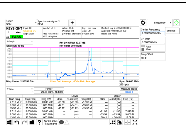
5G NR n41 15MHz BPSK Low Channel RB1-37 Port A+B
