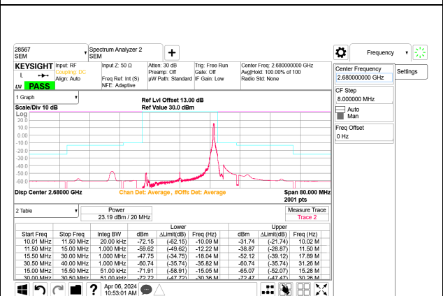
5G NR n41 20MHz BPSK High Channel RB1-50 Port B
