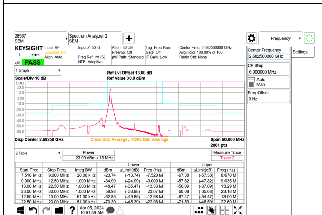
5G NR n41 15MHz BPSK High Channel RB1-0 Port B
