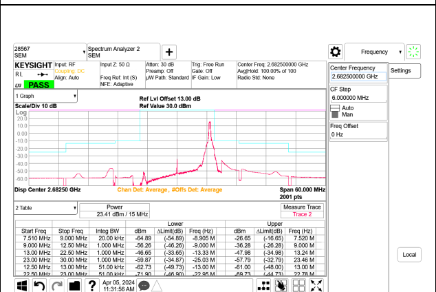
5G NR n41 15MHz BPSK High Channel RB1-37 Port B
