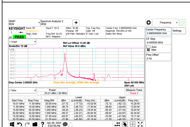
5G NR n41 20MHz BPSK High Channel RB1-0 Port B
