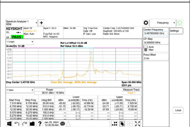
5G NR n77 15MHz BPSK Low Channel RB1-37, ID:27957
