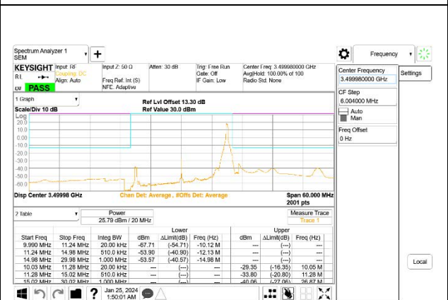
5G NR n77 20MHz BPSK Middle Channel RB1-50, ID:27957
