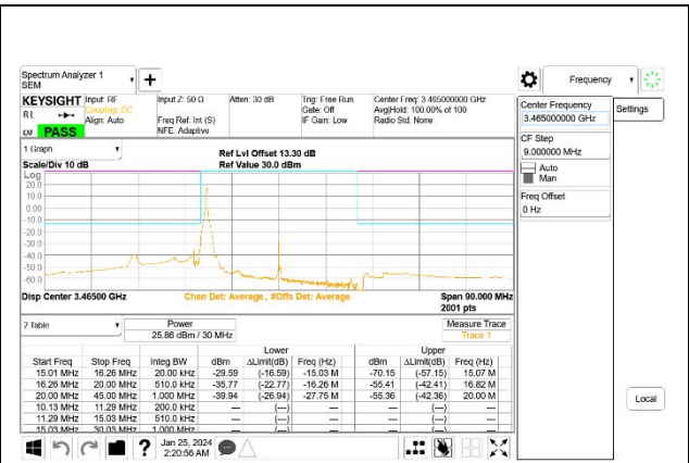
5G NR n77 30MHz BPSK Low Channel RB1-0, ID:27957
