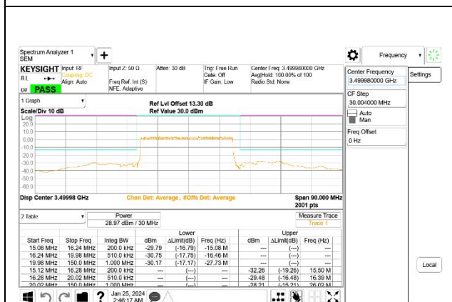
5G NR n77 30MHz BPSK Middle Channel RB75-0, ID:27957
