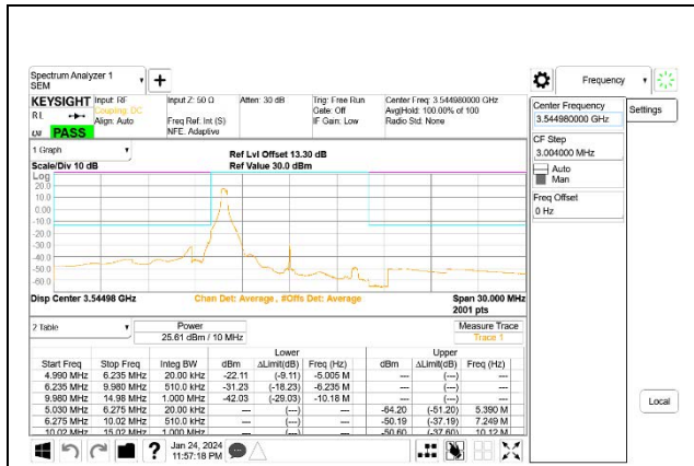
5G NR n77 10MHz BPSK High Channel RB1-0, ID:27957
