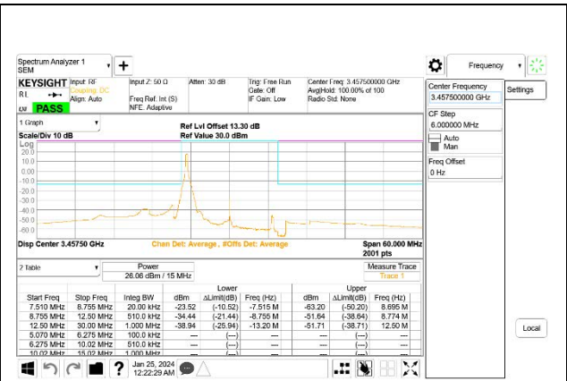
5G NR n77 15MHz BPSK Low Channel RB1-0, ID:27957
