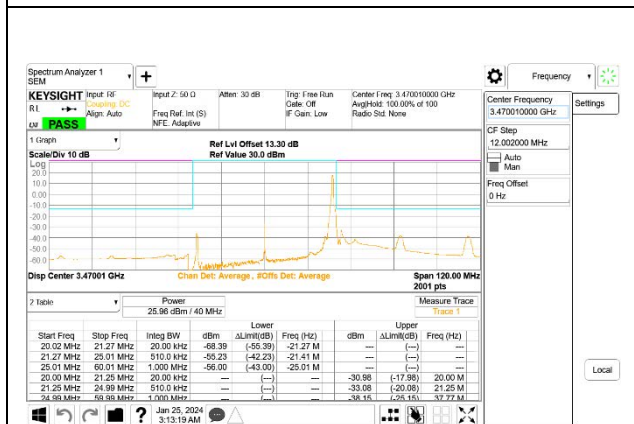
5G NR n77 40MHz BPSK Low Channel RB1-105, ID:27957
