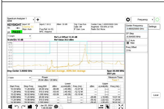
5G NR n77 20MHz BPSK Low Channel RB1-50, ID:27957
