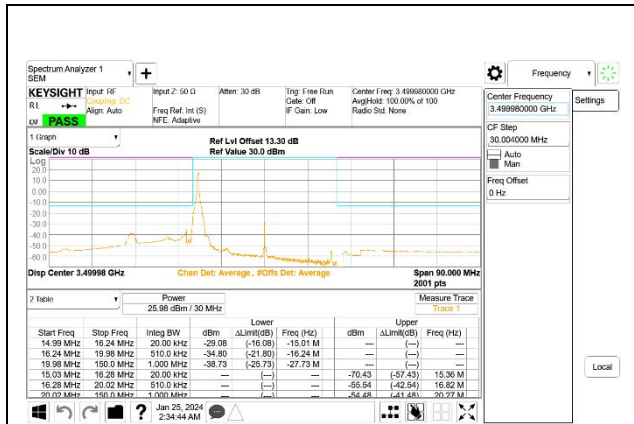
5G NR n77 30MHz BPSK Middle Channel RB1-0, ID:27957
