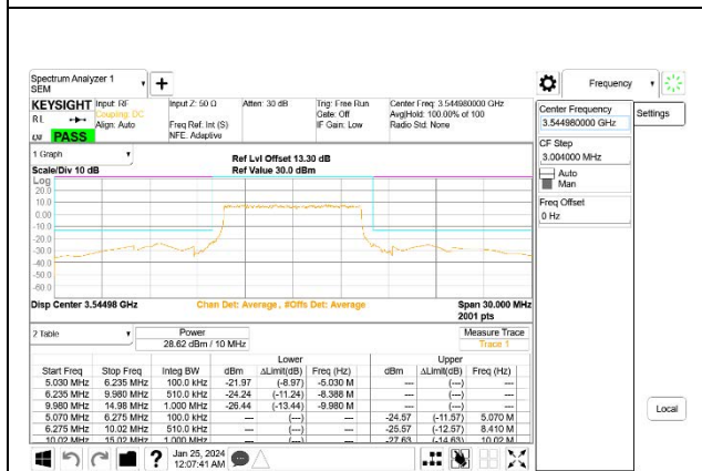
5G NR n77 10MHz BPSK High Channel RB24-0, ID:27957
