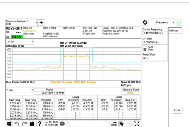
5G NR n77 15MHz BPSK Low Channel RB36-0, ID:27957
