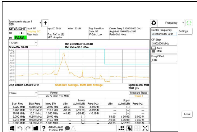
5G NR n77 10MHz BPSK Low Channel RB1-0, ID:27957
