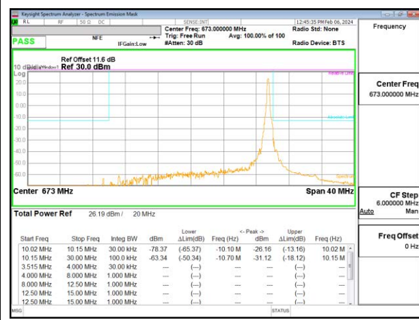
5G NR n71 20MHz BPSK Low Channel RB1-105, ID:28567
