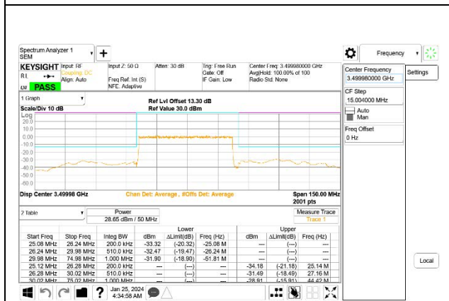
5G NR n77 50MHz BPSK Middle Channel RB128-0, ID:27957
