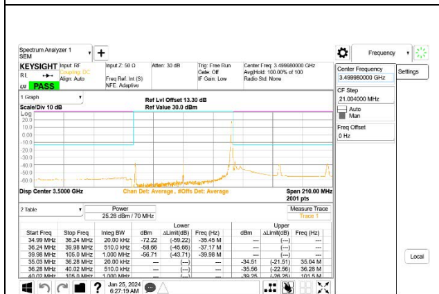
5G NR n77 70MHz BPSK Middle Channel RB1-188, ID:27957
