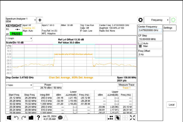
5G NR n77 50MHz BPSK Low Channel RB128-0, ID:27957
