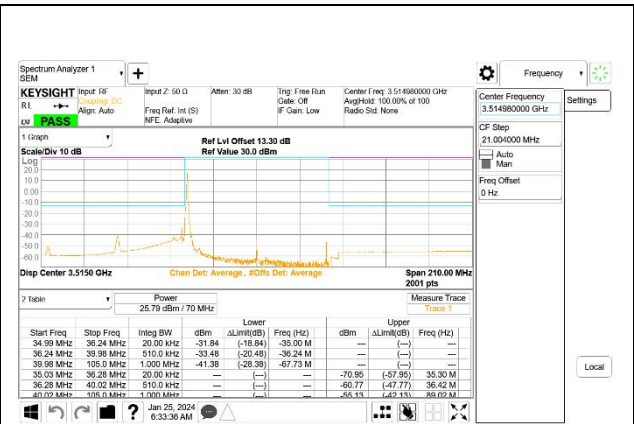
5G NR n77 70MHz BPSK High Channel RB1-0, ID:27957
