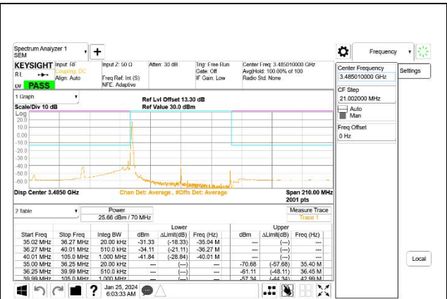
5G NR n77 70MHz BPSK Low Channel RB1-0, ID:27957
