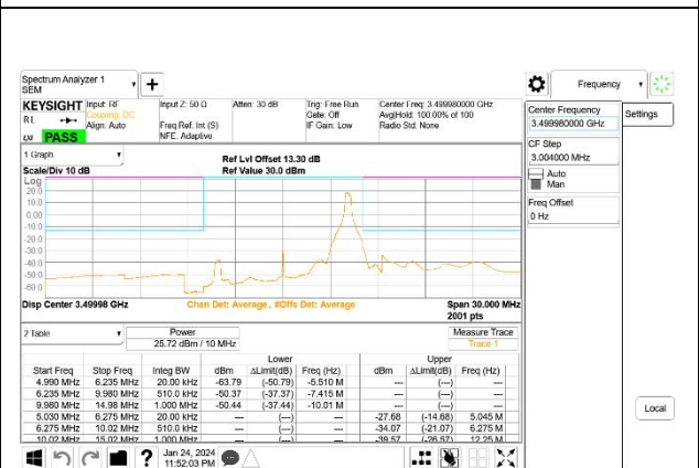
5G NR n77 10MHz BPSK Middle Channel RB1-23, ID:27957
