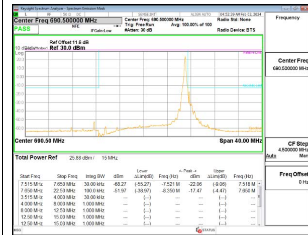
5G NR n71 15MHz BPSK High Channel RB1-78, ID:28567
