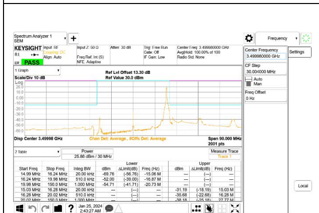
5G NR n77 30MHz BPSK Middle Channel RB1-77, ID:27957
