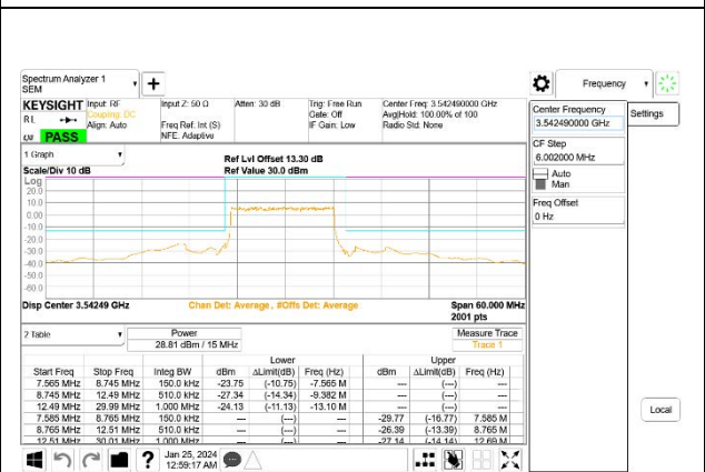
5G NR n77 15MHz BPSK High Channel RB36-0, ID:27957
