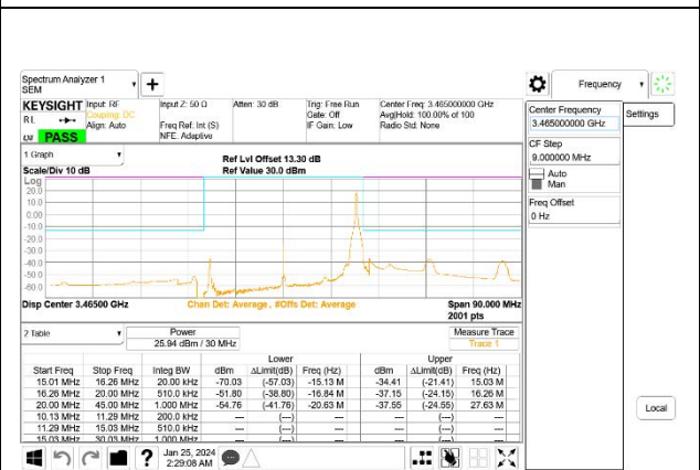
5G NR n77 30MHz BPSK Low Channel RB1-77, ID:27957
