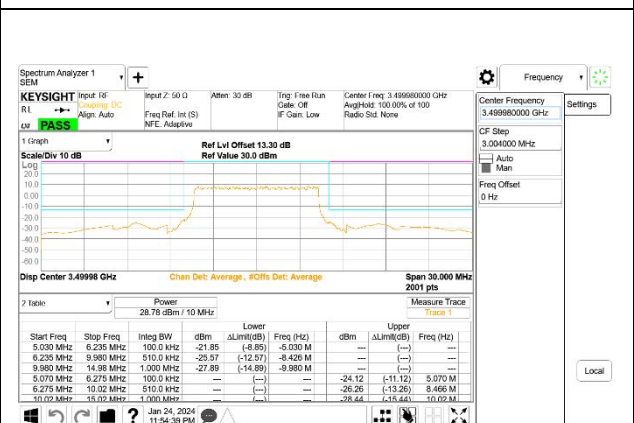
5G NR n77 10MHz BPSK Middle Channel RB24-0, ID:27957
