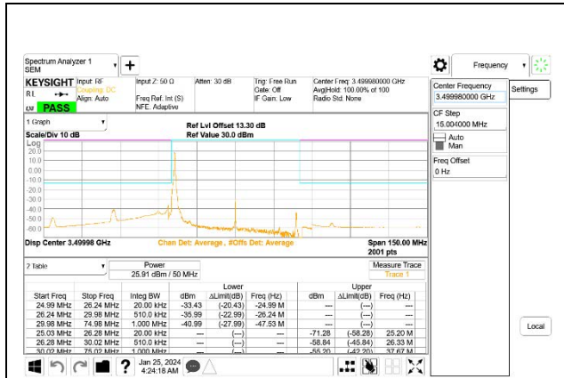
5G NR n77 50MHz BPSK Middle Channel RB1-0, ID:27957
