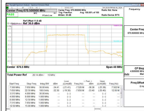
5G NR n71 15MHz BPSK Low Channel RB75-0, ID:28567
