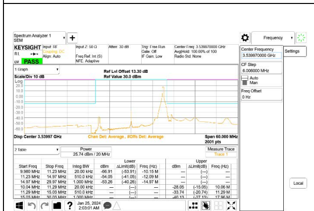
5G NR n77 20MHz BPSK High Channel RB1-50, ID:27957
