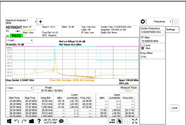
5G NR n77 50MHz BPSK High Channel RB1-0, ID:27957
