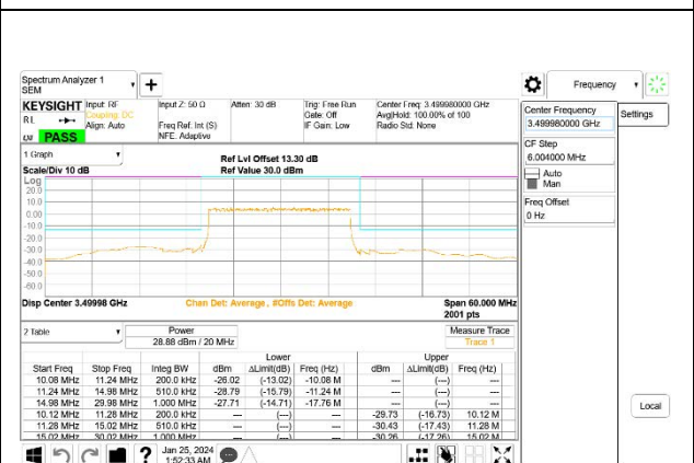
5G NR n77 20MHz BPSK Middle Channel RB50-0, ID:27957
