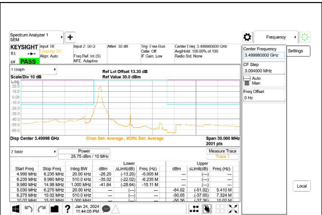
5G NR n77 10MHz BPSK Middle Channel RB1-0, ID:27957
