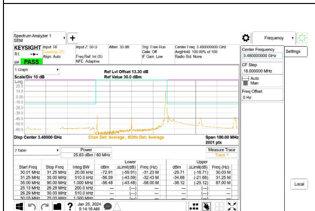
5G NR n77 60MHz BPSK Low Channel RB1-161, ID:27957
