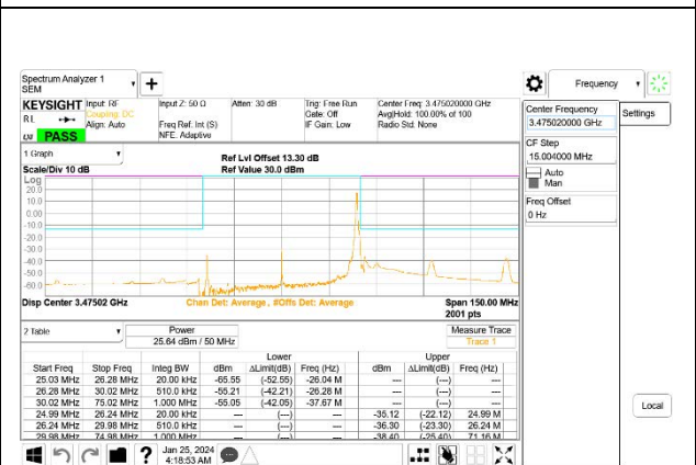
5G NR n77 50MHz BPSK Low Channel RB1-132, ID:27957
