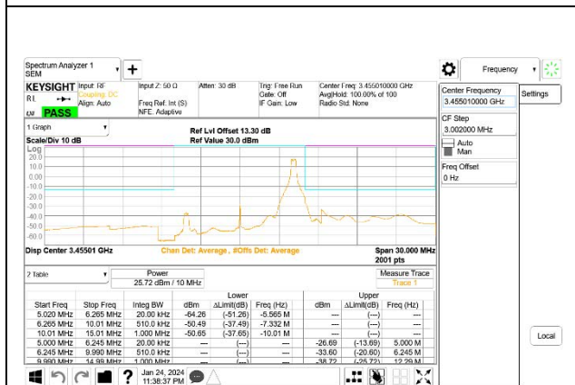
5G NR n77 10MHz BPSK Low Channel RB1-23, ID:27957
