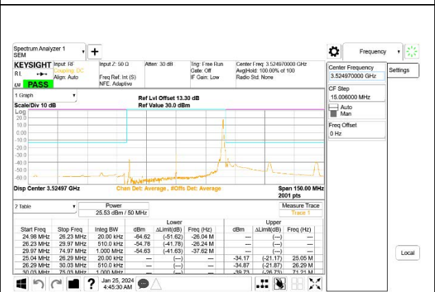
5G NR n77 50MHz BPSK High Channel RB1-132, ID:27957
