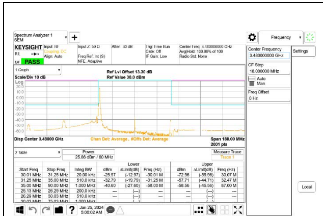
5G NR n77 60MHz BPSK Low Channel RB1-0, ID:27957
