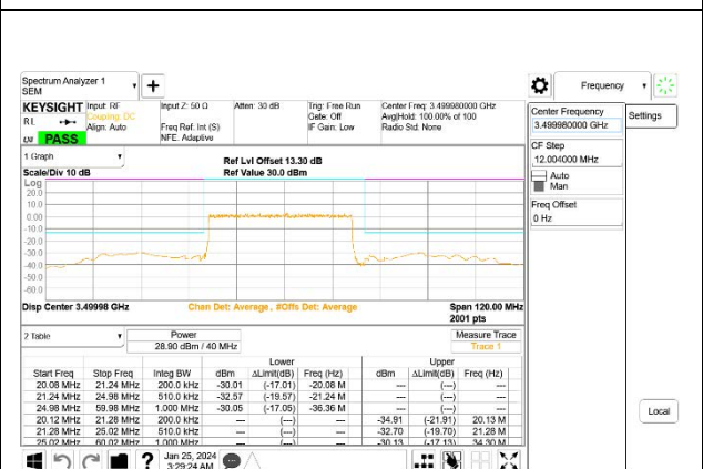
5G NR n77 40MHz BPSK Middle Channel RB100-0, ID:27957
