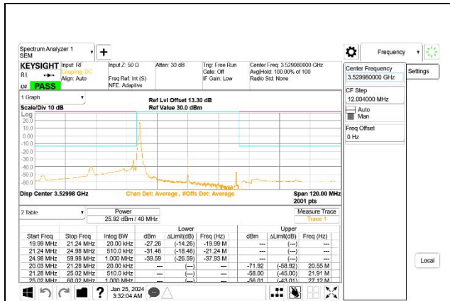
5G NR n77 40MHz BPSK High Channel RB1-0, ID:27957
