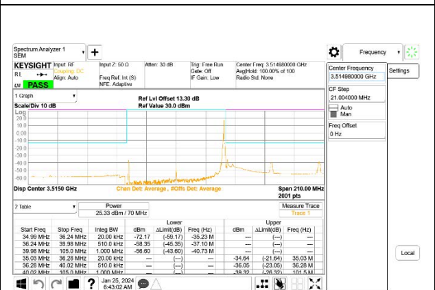
5G NR n77 70MHz BPSK High Channel RB1-188, ID:27957
