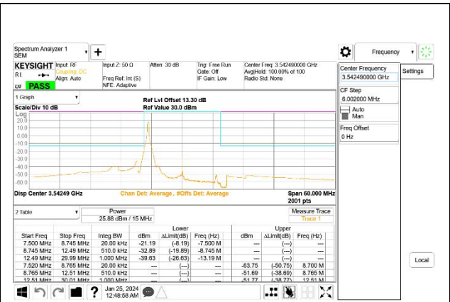
5G NR n77 15MHz BPSK High Channel RB1-0, ID:27957
