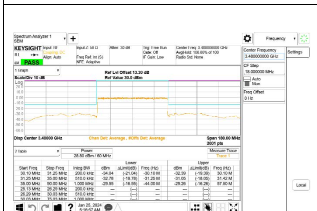
5G NR n77 60MHz BPSK Low Channel RB162-0, ID:27957
