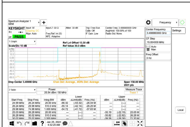
5G NR n77 50MHz BPSK Middle Channel RB1-132, ID:27957
