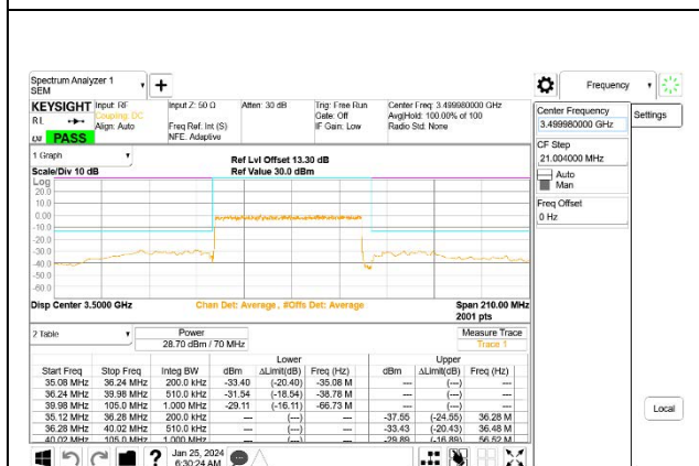
5G NR n77 70MHz BPSK Middle Channel RB180-0, ID:27957
