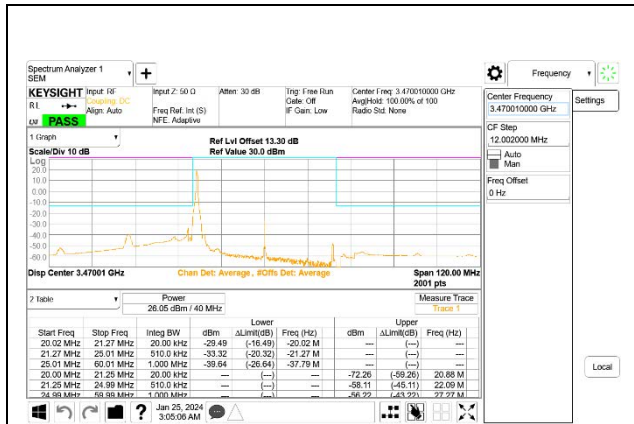
5G NR n77 40MHz BPSK Low Channel RB1-0, ID:27957
