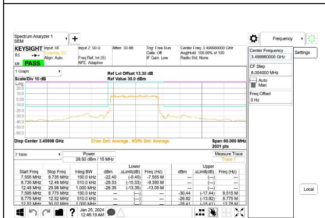
5G NR n77 15MHz BPSK Middle Channel RB36-0, ID:27957
