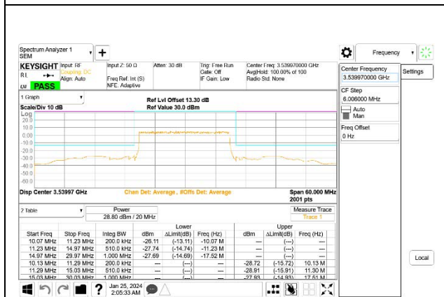
5G NR n77 20MHz BPSK High Channel RB50-0, ID:27957
