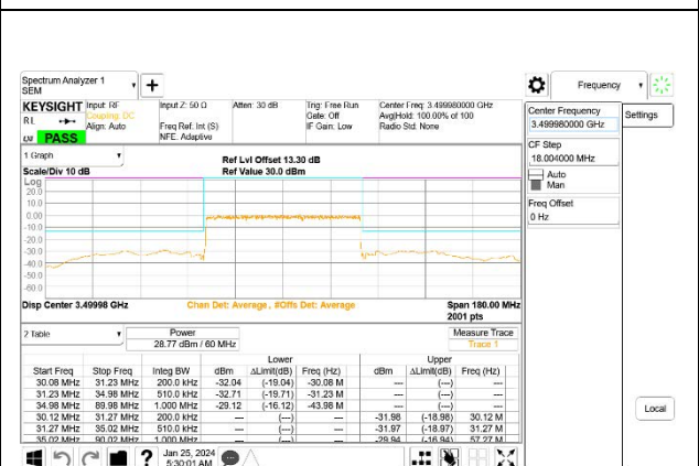
5G NR n77 60MHz BPSK Middle Channel RB162-0, ID:27957
