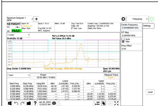
5G NR n77 10MHz BPSK High Channel RB1-23, ID:27957
