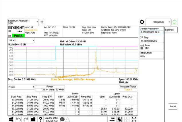
5G NR n77 60MHz BPSK High Channel RB1-161, ID:27957
