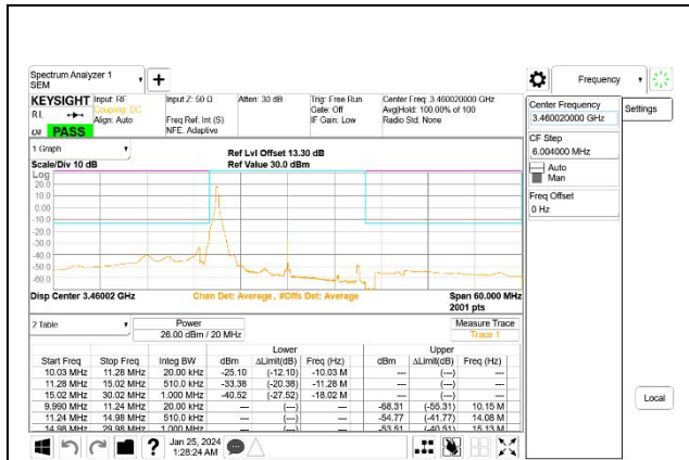
5G NR n77 20MHz BPSK Low Channel RB1-0, ID:27957
