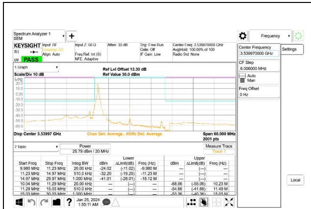
5G NR n77 20MHz BPSK High Channel RB1-0, ID:27957
