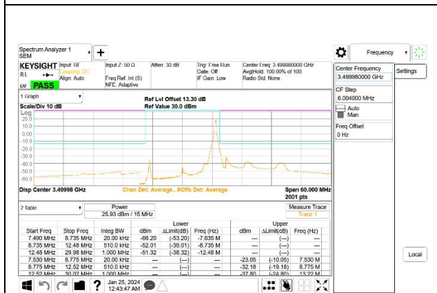
5G NR n77 15MHz BPSK Middle Channel RB1-37, ID:27957
