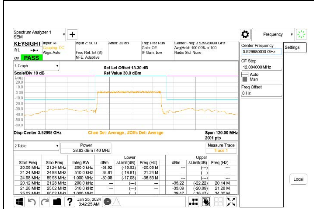
5G NR n77 40MHz BPSK High Channel RB100-0, ID:27957
