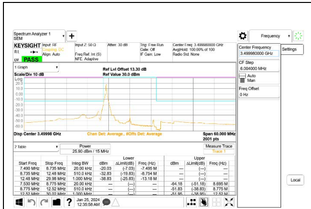
5G NR n77 15MHz BPSK Middle Channel RB1-0, ID:27957
