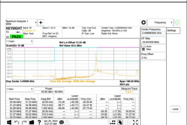
5G NR n77 60MHz BPSK Middle Channel RB1-161, ID:27957
