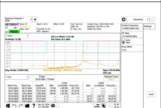
5G NR n77 70MHz BPSK Low Channel RB1-188, ID:27957
