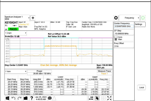
5G NR n77 50MHz BPSK High Channel RB128-0, ID:27957
