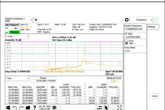
5G NR n77 40MHz BPSK Middle Channel RB1-105, ID:27957
