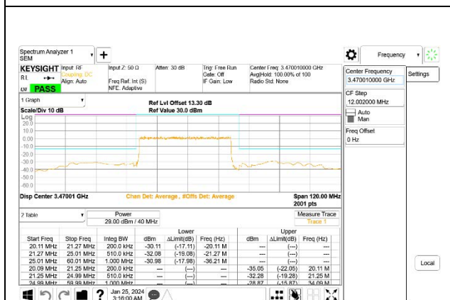
5G NR n77 40MHz BPSK Low Channel RB100-0, ID:27957
