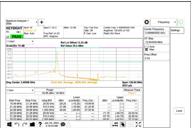
5G NR n77 40MHz BPSK Middle Channel RB1-0, ID:27957
