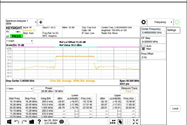
5G NR n77 30MHz BPSK Low Channel RB75-0, ID:27957
