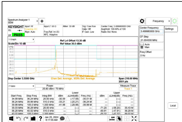
5G NR n77 70MHz BPSK Middle Channel RB1-0, ID:27957
