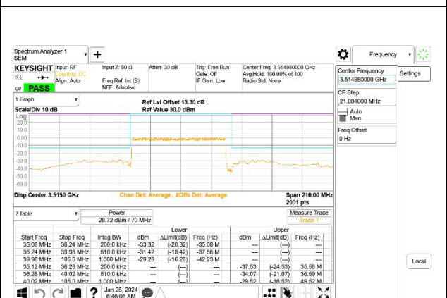
5G NR n77 70MHz BPSK High Channel RB180-0, ID:27957
