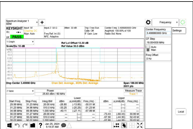
5G NR n77 60MHz BPSK Middle Channel RB1-0, ID:27957
