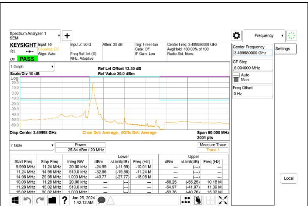
5G NR n77 20MHz BPSK Middle Channel RB1-0, ID:27957
