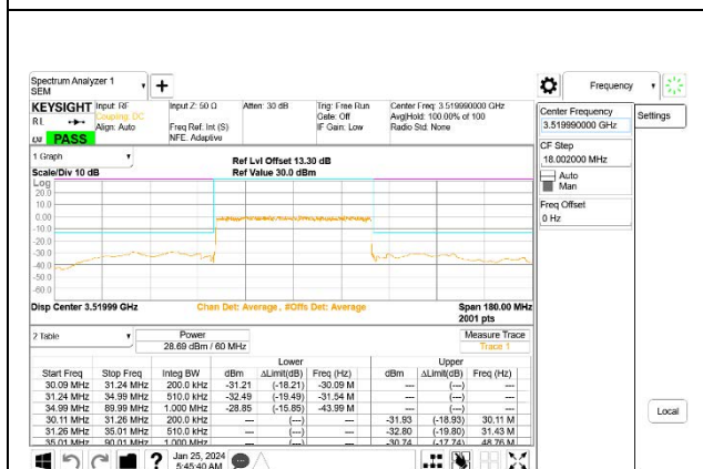
5G NR n77 60MHz BPSK High Channel RB162-0, ID:27957
