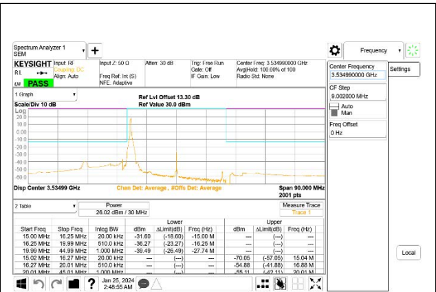
5G NR n77 30MHz BPSK High Channel RB1-0, ID:27957
