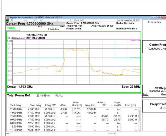
5G NR n70 5MHz BPSK Middle Channel (Upper Block) RB25-0
