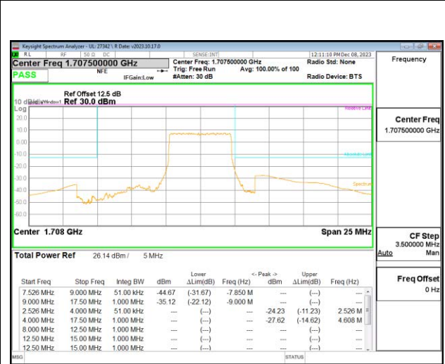
5G NR n70 5MHz BPSK High Channel (Upper Block) RB25-0
