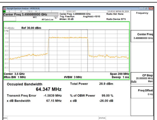
5G NR n77 70MHz BPSK Middle Channel RB180-0, ID 27342
