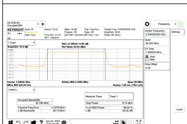
5G NR n77 40MHz BPSK Middle Channel RB100-0, ID 27342
