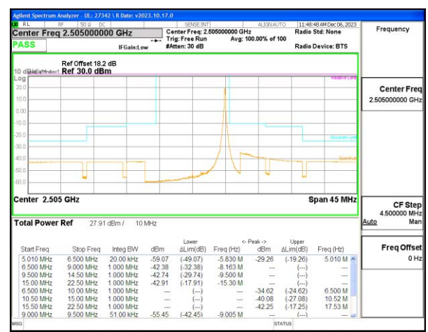
LTE B7 10MHz QPSK Low Channel RB1-49
