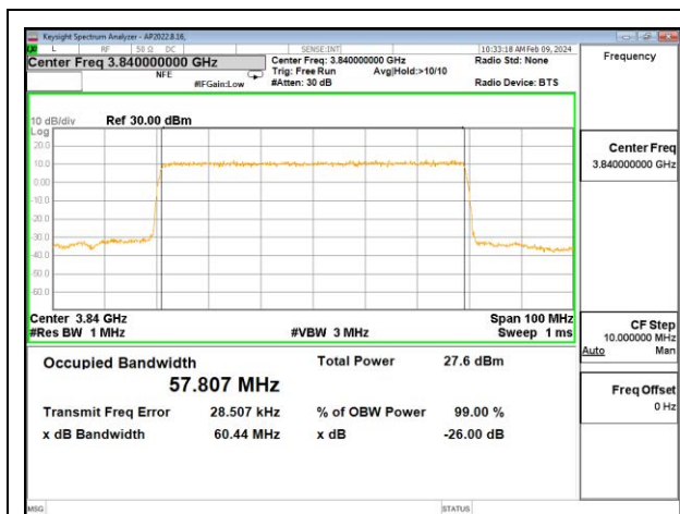
5G NR n77 60MHz BPSK Middle Channel RB162-0, ID 27342
