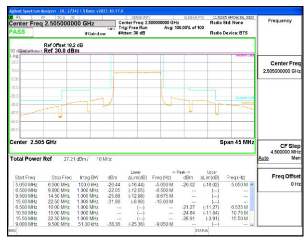
LTE B7 10MHz QPSK Low Channel RB50-0
