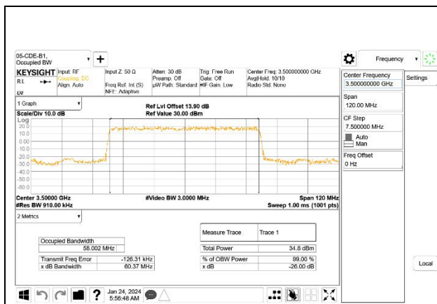
5G NR n77 60MHz BPSK Middle Channel RB162-0, ID 27342
