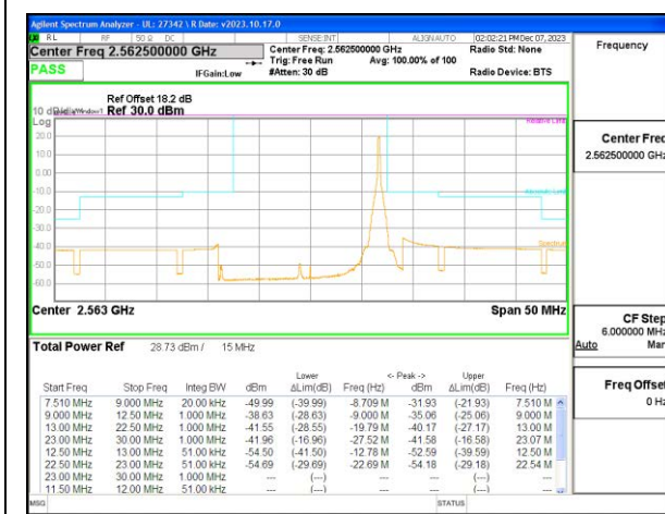
LTE B7 15MHz QPSK High Channel RB1-74
