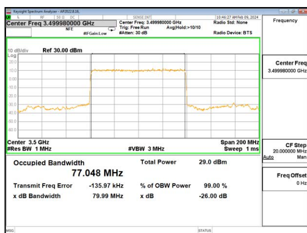
5G NR n77 80MHz BPSK Middle Channel RB216-0, ID 27342
