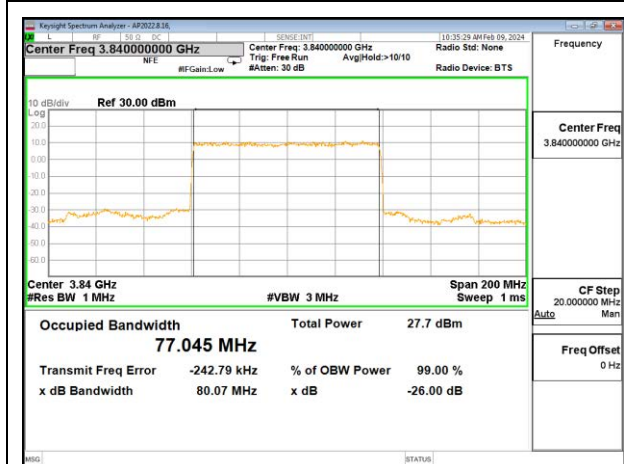
5G NR n77 80MHz BPSK Middle Channel RB216-0, ID 27342
