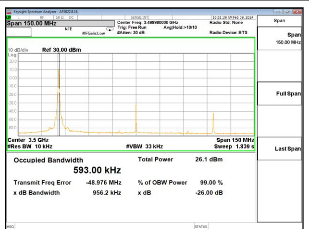
5G NR n77 100MHz BPSK Middle Channel RB1-0, ID 27342
