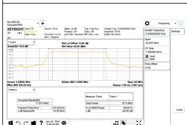
5G NR n77 20MHz BPSK Middle Channel RB50-0, ID 27342
