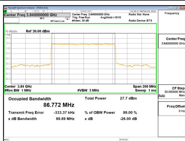
5G NR n77 90MHz BPSK Middle Channel RB243-0, ID 27342
