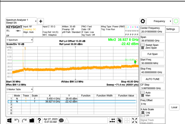
5G NR n77 15MHz BPSK Low Channel RB1-0, ID:19210
