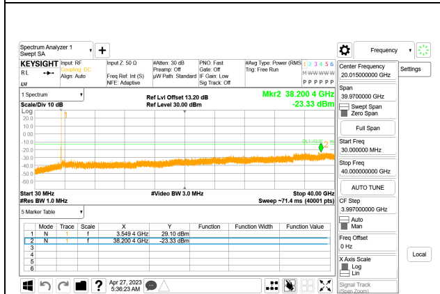
5G NR n77 10MHz BPSK High Channel RB1-23, ID:19210
