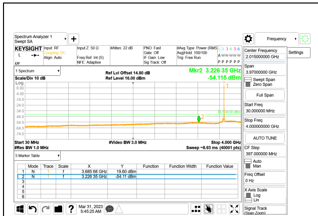
LTE B48 15MHz QPSK High Channel RB1-0 (30MHz to 4.0GHz) , ID:28567
