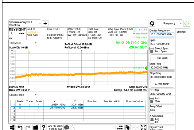
5G NR n41 60MHz BPSK High Channel RB1-161, ID:19210
