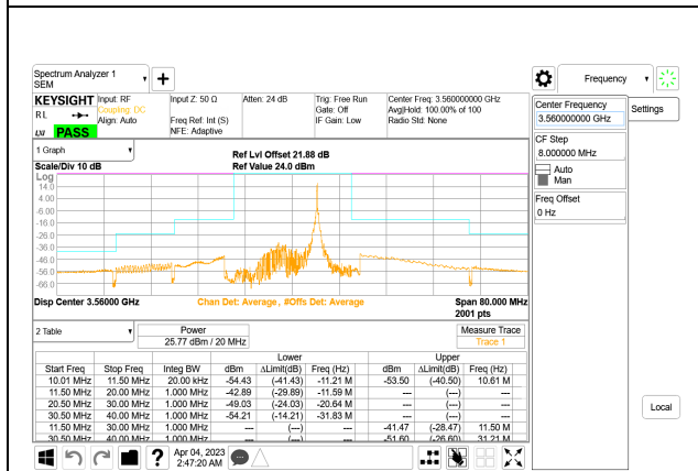
LTE B48 15MHz QPSK Low Channel RB1-74, ID:28567
