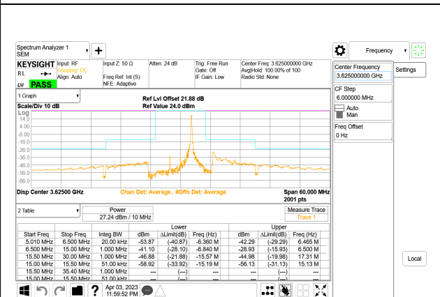
LTE B48 5MHz QPSK Middle Channel RB1-24, ID:28567
