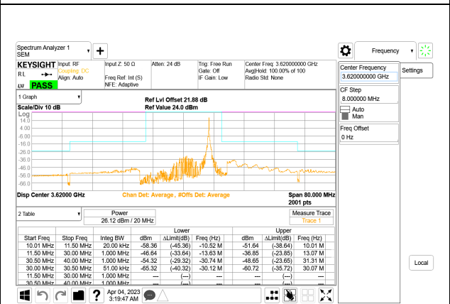
LTE B48 15MHz QPSK Middle Channel RB1-74, ID:28567
