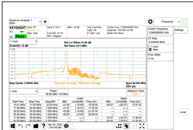
LTE B48 15MHz QPSK Low Channel RB1-0, ID:28567
