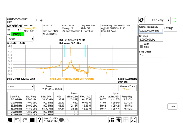
LTE B48 5MHz QPSK Middle Channel RB1-0, ID:28567
