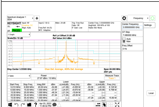
LTE B48 5MHz QPSK Low Channel RB1-24, ID:28567
