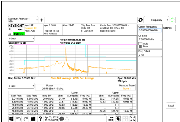
LTE B48 5MHz QPSK Low Channel RB1-0, ID:28567
